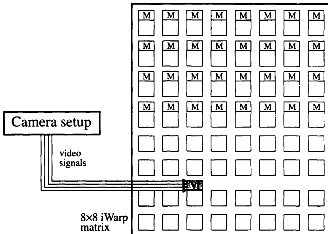
Fig. 4 Block diagram of the image acquisition system. The shaded boxes labeled "M" indicate the 16M DRAMs connected to local iWarp cells while the shaded box labeled "VI" refers to the video interface connected to one of the iWarp cells.
