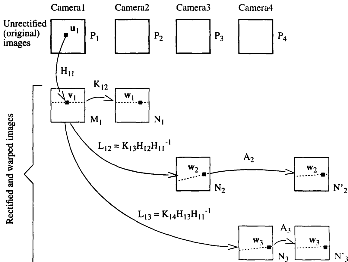
Fig. 12 The approximate depth recovery scheme (compare this with Fig. 11)
