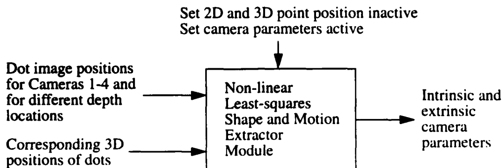
Fig. 7 Non-linear least-squares approach to extraction of camera parameters
