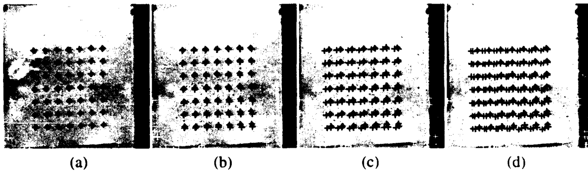
Fig. 6 Detecting and tracking the calibration points (only part of the image associated with Camera 1 is shown). The black + 's are the detected points while the white + 's are the spurious and rejected points: (a) Points detected in image of Camera 1; (b) Points detected in images of Cameras 1 and 2; (c) Points detected in images of Cameras 1, 2, and 3; (d) Points detected in all images.
