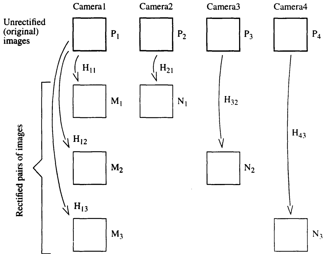
Fig. 9 Image rectification scheme
