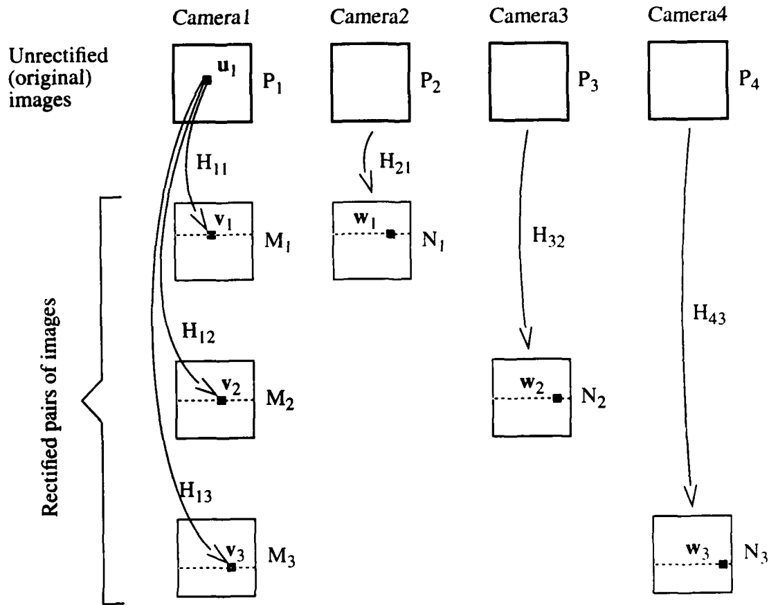
Fig. 10 Recovering depth from multibaseline stereo after rectification
