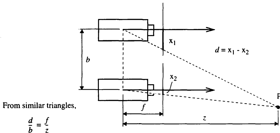
Fig. 2 Relationship between the baseline b , disparity d , focal length f , and depth z
