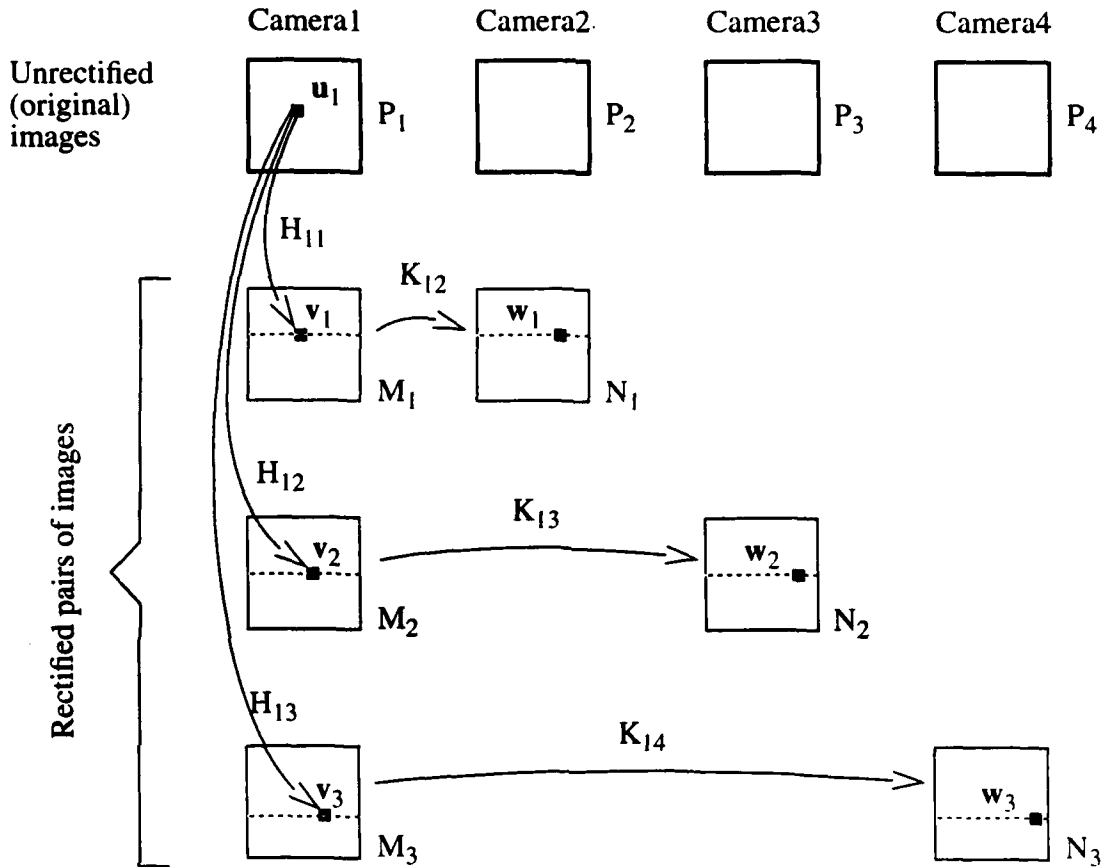
Fig. 11 A computationally more efficient depth recovery scheme
