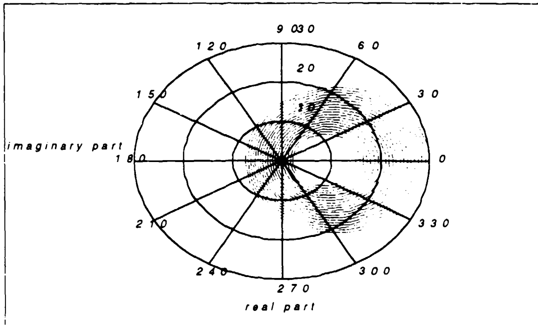
Figure 9-2 Tracking Error Rate Phasor Diagram
