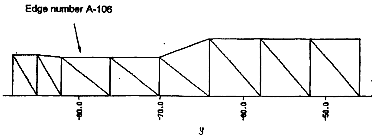
Figure 13. Antenna element on edge number 106 (astern).
