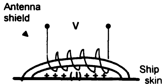
Figure 6. Ferrite loop on the ship's surface.
