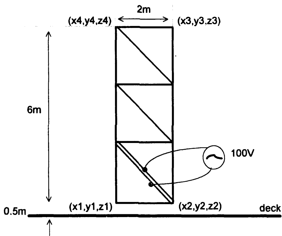
Figure 15. Transmit monopole and its excitation.
