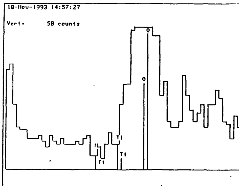
Figure 4.7 SEM EDX Spectrums in the vicinity of the oxygen and nitrogen K-lines, TiN inclusion (top), GMAW inclusion (bottom).
