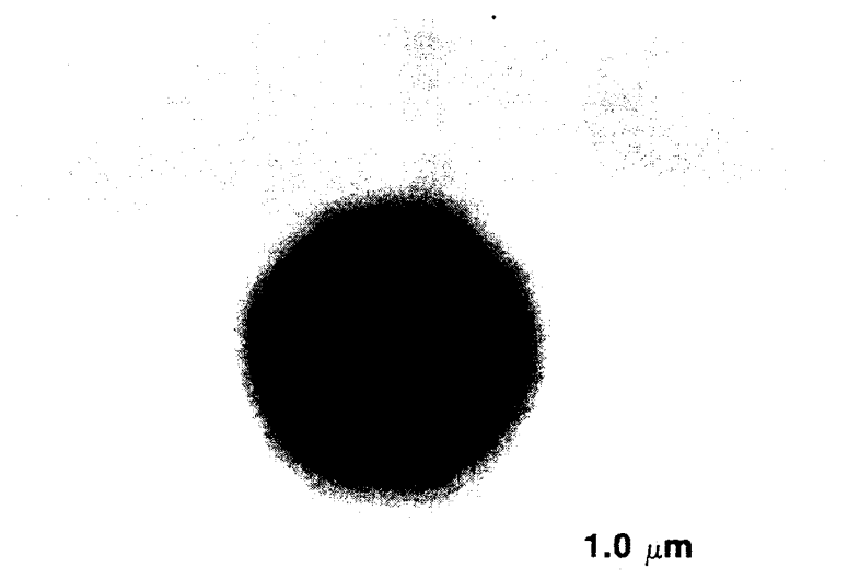
Figure 3.9 SEM EDX spectrum of titanium rich phase of a GMAW sample (top). Photograph of 0.7 micron inclusion (50.9 Kx) showing the titanium rich phase in the center of the inclusion (bottom).
