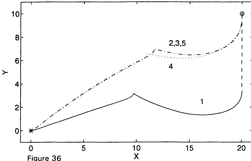
Path Comparison of Robot Programs, 270 Degree Turn
