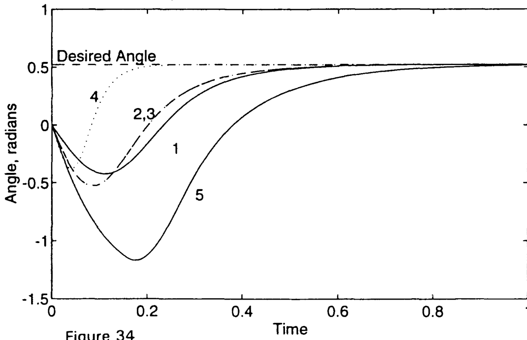
Angle Trajectory Comparison of Robot Programs, 30 Degree Turn
