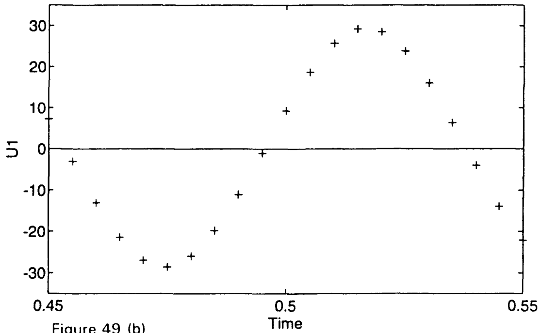
Discrete Time Velocities of U1: Robot 5, Highly Oscillatory Solution
