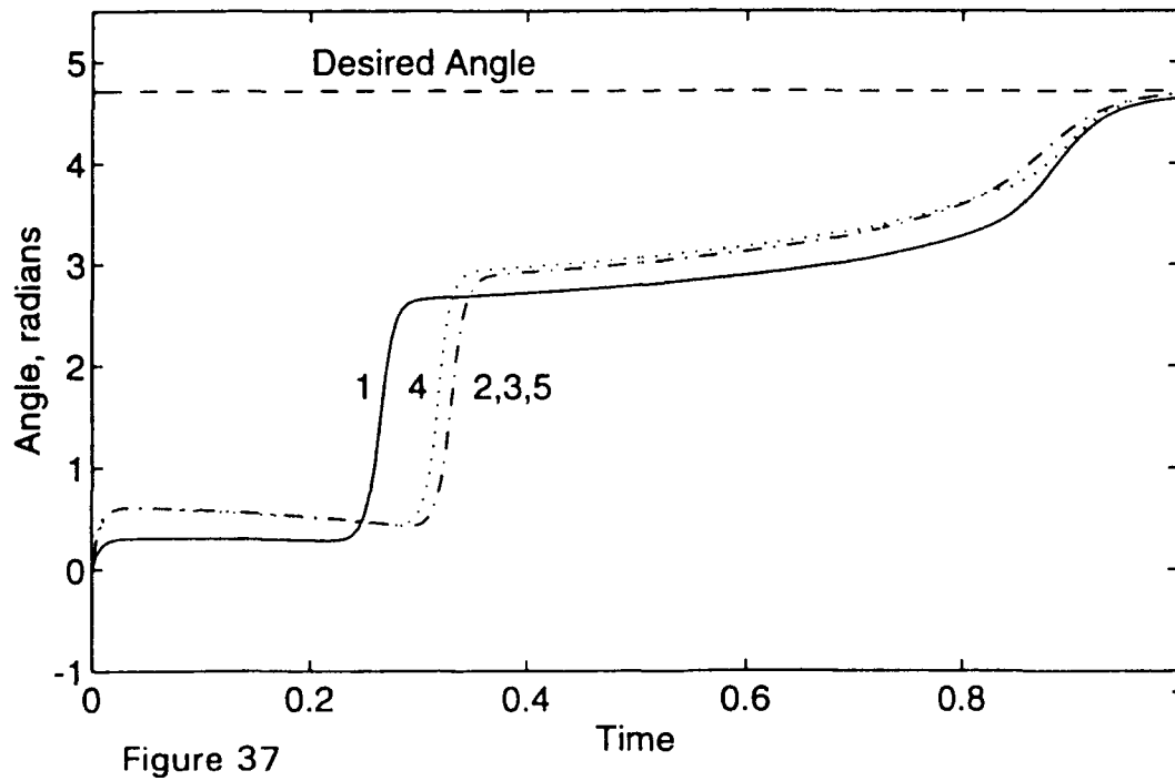
Angle Trajectory Comparison of Robot Programs, 270 Degree Turn
