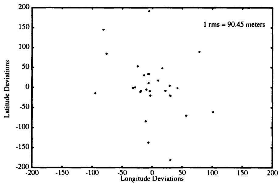
Figure 52. Motorola First Fix Accuracy After 3 Hours Off
