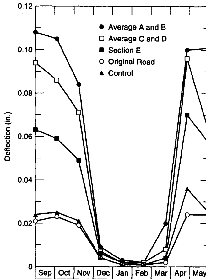
Figure 18. Plate deflections, 1992-1993.
