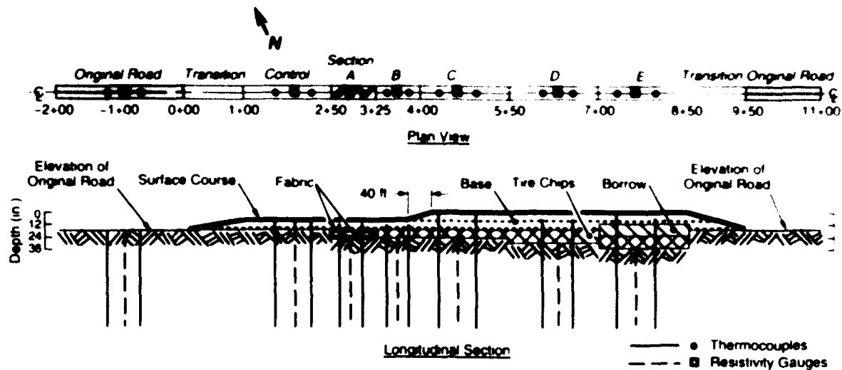
Figure 9. Location of thermocouples and resistivity gauges.
