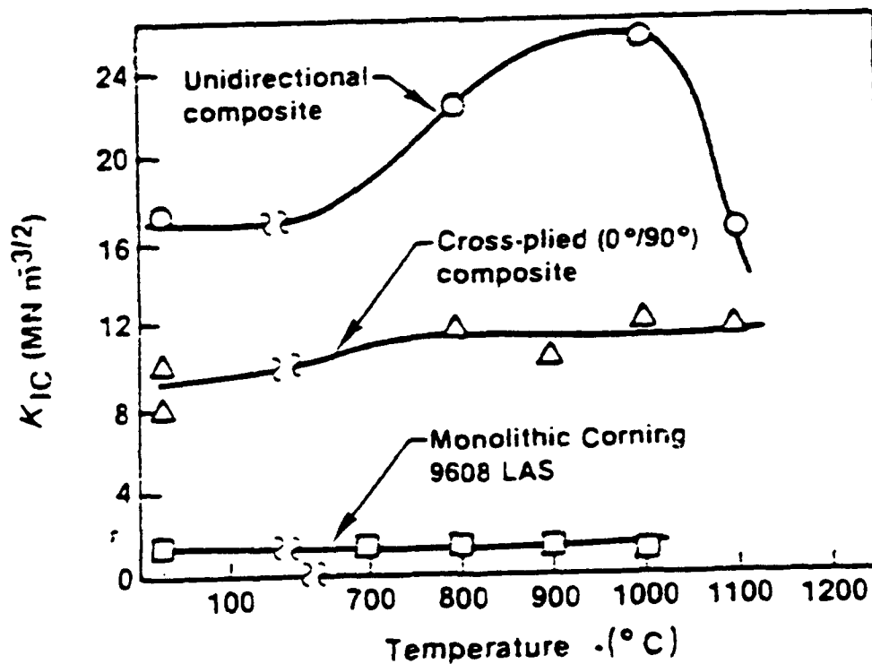
Figure 7. Fracture toughness K_{IC} of LAS-SiC yarn composites [Ref.7]
