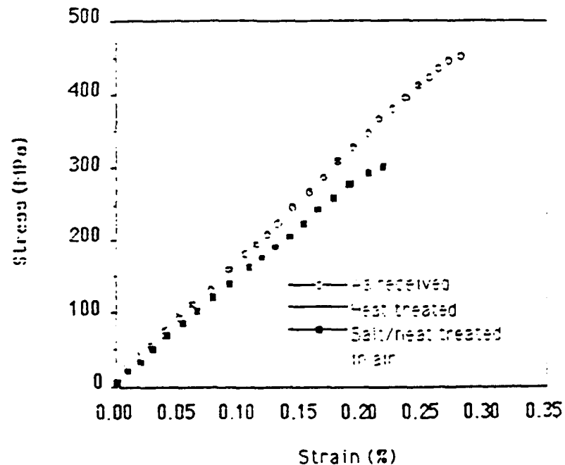
Figure 13. Stress-strain curves of LAS- \text{SiC} tensile specimens exposed to varying atmospheres [Ref. 16]
