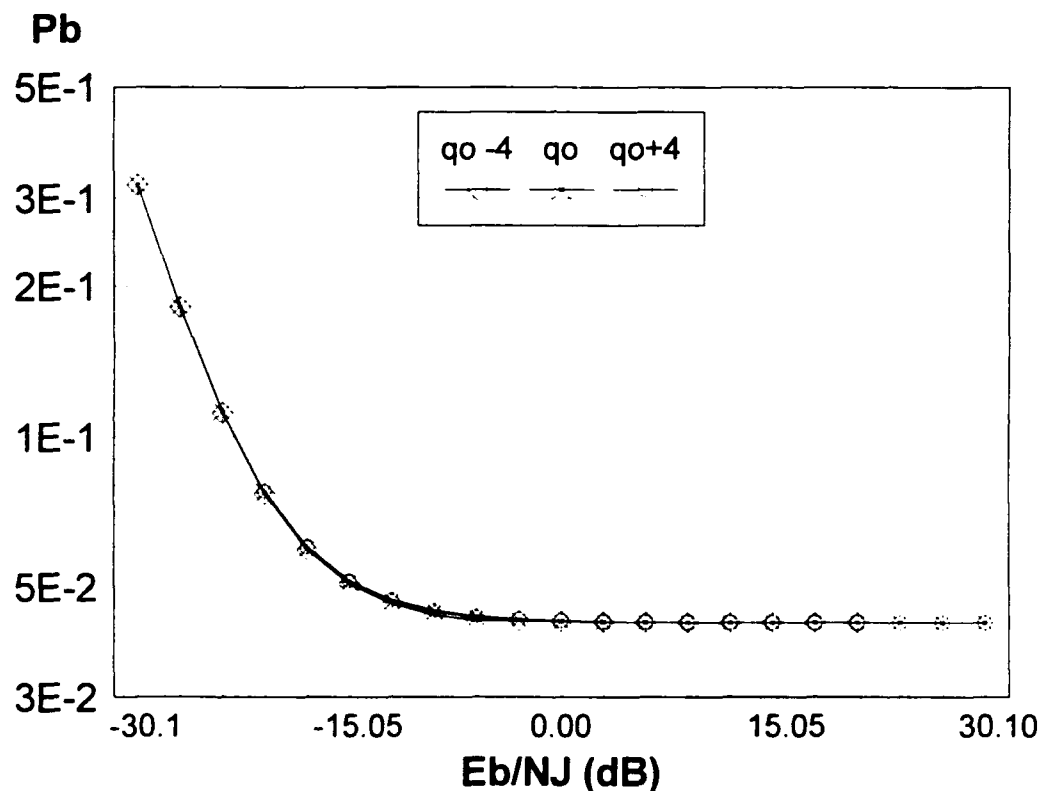
Figure 36. Worst Case Multi-Tone Jamming for E_b/N_j=13.35\text{dB} , R_b=0 , R_j=100
