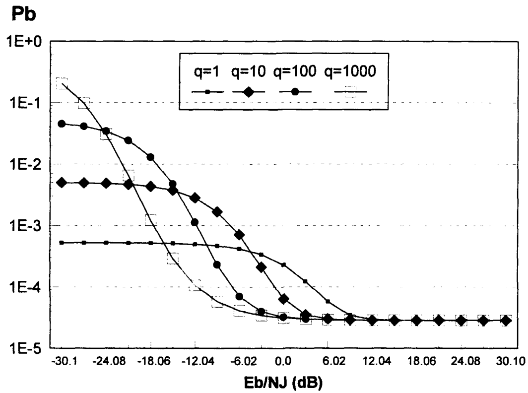
Figure 26. E_b/N_0=13.35\text{dB} , R_b=100 , R_f=0.0
