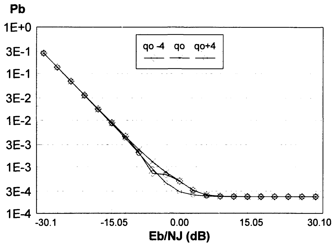
Figure 39. Worst Case Multi-Tone Jamming E_b/N_0=13.35\text{dB} , R_b=25 , R_j=25 ,
