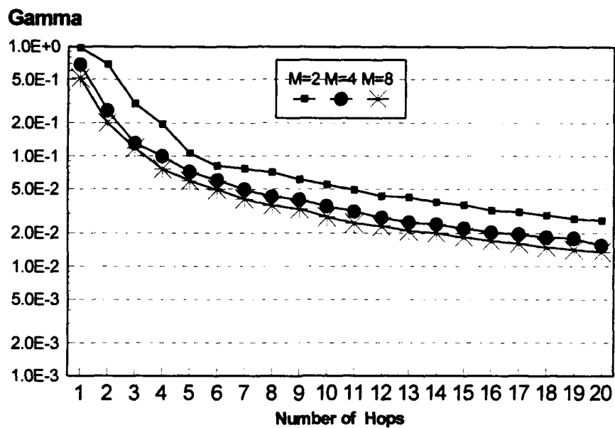
Figure 10. Fraction of Jammed Bandwidth E_h/N_o=13.35\text{dB} , E_h/N_f=3\text{dB} , R_b=100
