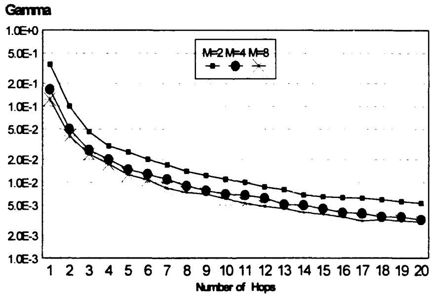
Figure 13. Fraction of Bandwidth Jammed E_b/N_o=13.35\text{dB} , E_b/N_f=10\text{dB} , R_b=10
