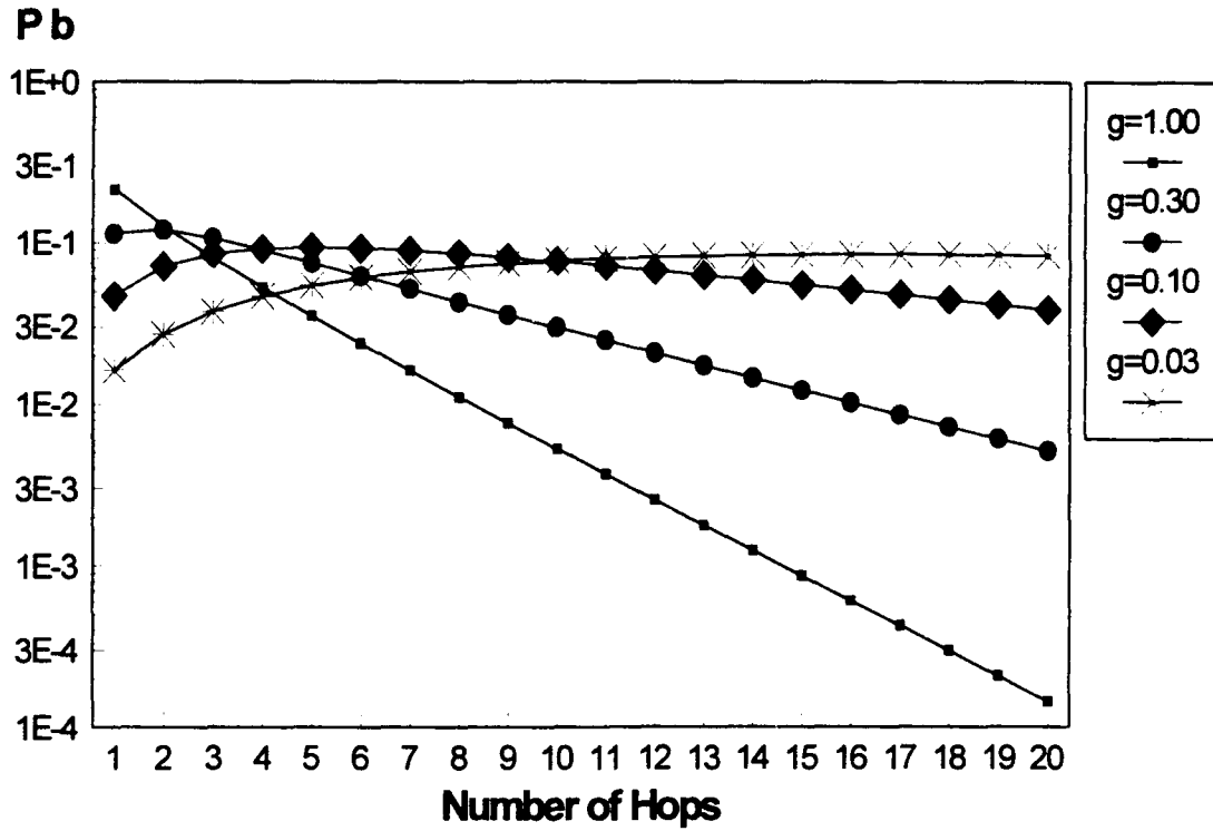
Figure 19. Performance for fixed values of gamma E_b/N_o=13.35\text{dB} , E_b/N_f=3\text{dB} , R_b=10
