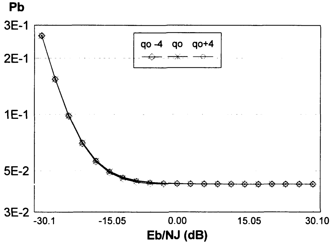
Figure 37. Worst Case Multi-Tone Jamming E_b/N_0 = 13.35 dB, R_b = 0 , R_j = 0
