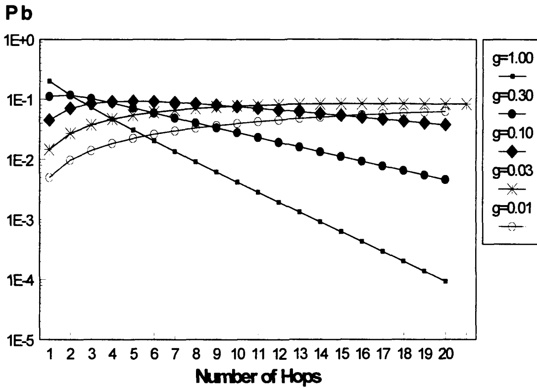
Figure 23. Performance for fixed values of gamma E_b/N_o=13.35\text{dB} , E_b/N_f=3\text{dB} , R_b=100
