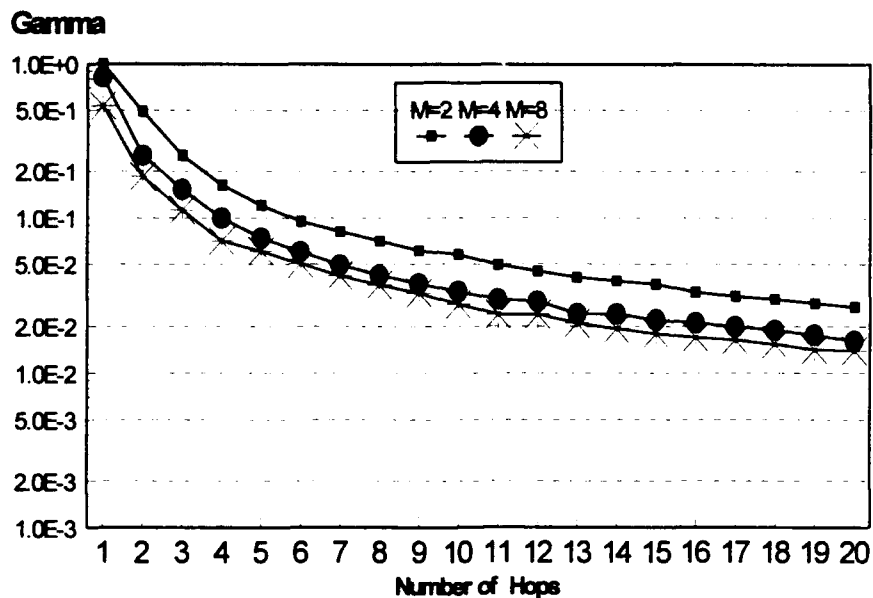
Figure 14. Fraction of Bandwidth Jammed E_b/N_o=16\text{dB} , E_b/N_f=3\text{dB} , R_b=10
