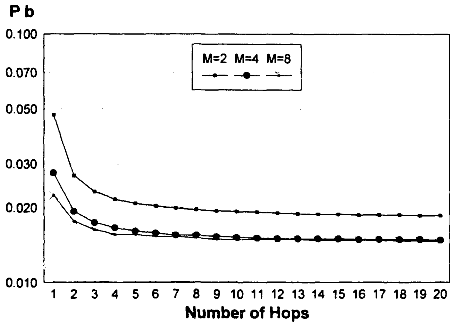
Figure 4. Worst Case Partial-band Jamming E_b/N_0=13.35\text{dB} , E_b/N_f=10\text{dB} , R_b=100
