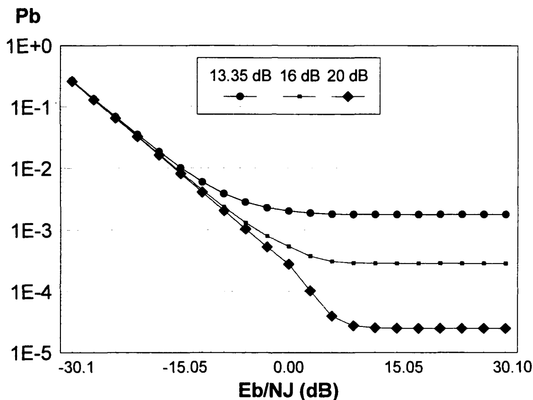
Figure 42. Worst Case Multi-Tone Jamming for Several Values of E_b/N_o , R_b=10 , R_j=10
