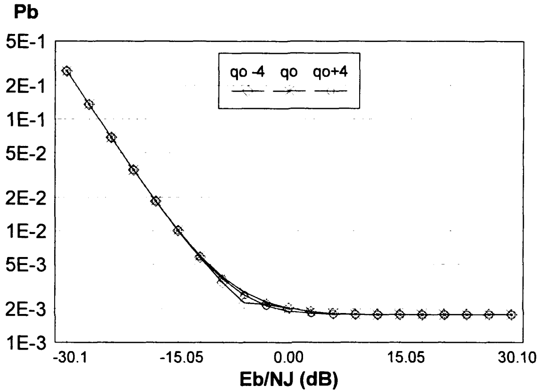
Figure 38. Worst Case Multi-Tone Jamming E_b/N_0=20\text{dB} , R_b=10 , R_J=10 ,
