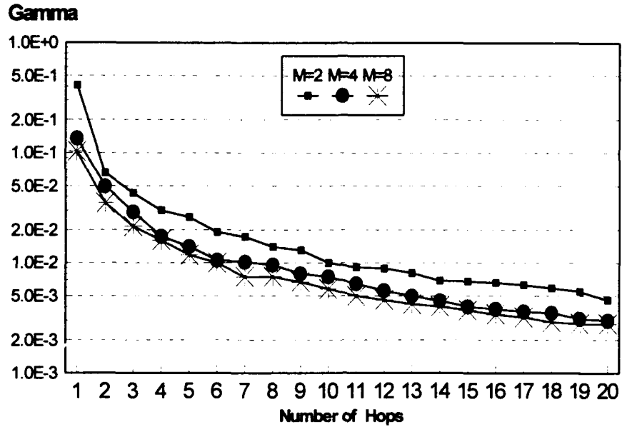
Figure 12. Fraction of Bandwidth Jammed E_b/N_o=13.35\text{dB} , E_b/N_f=10\text{dB} , R_b=100
