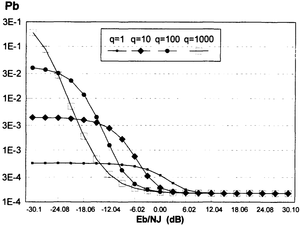
Figure 30. E_b/N_0=13.35\text{dB} , R_b=10 , R_j=1
