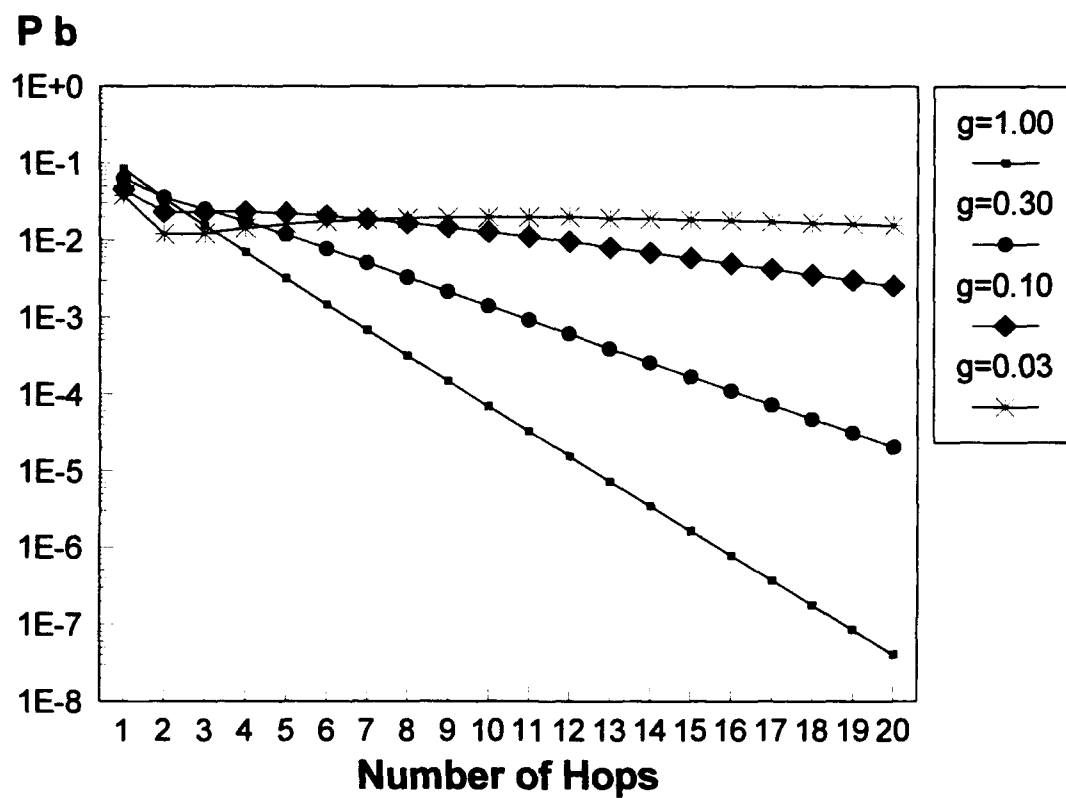
Figure 21. Performance for fixed values of gamma E_h/N_o=13.35\text{dB} , E_h/N_f=3\text{dB} , R_b=1
