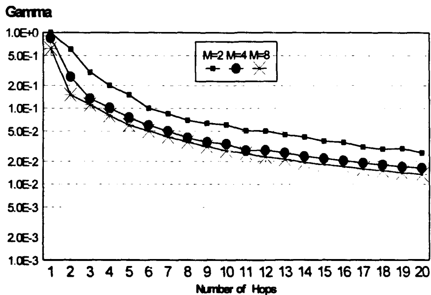
Figure 11. Fraction of Bandwidth Jammed E_h/N_o=13.35\text{dB} , E_h/N_f=3\text{dB} , R_b=10
