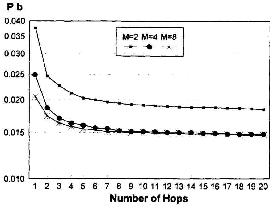
Figure 4. Worst Case Partial-band Jamming E_b/N_0=13.35\text{dB} , E_b/N_f=10\text{dB} , R_b=100
