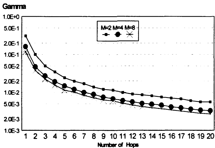
Figure 15. Fraction of Bandwidth Jammed E_b/N_o=16\text{dB} , E_b/N_f=3\text{dB} , R_b=10
