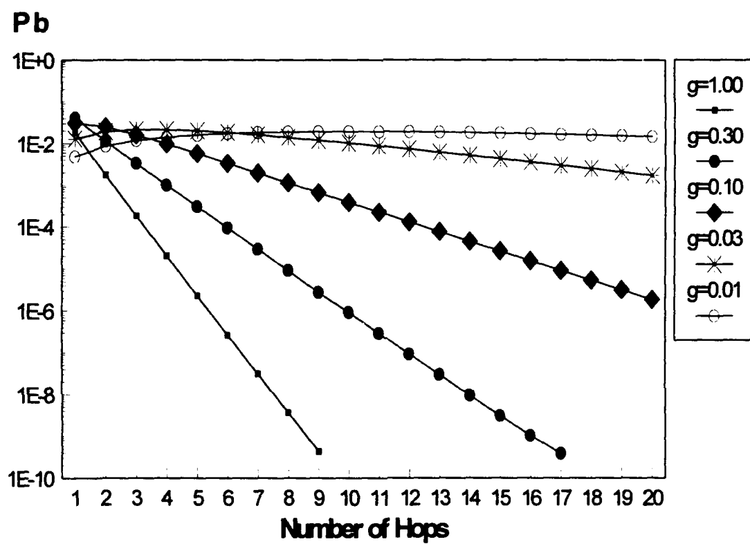
Figure 22. Performance for fixed values of gamma E_b/N_0=13.35\text{dB} , E_b/N_f=10\text{dB} , R_b=100
