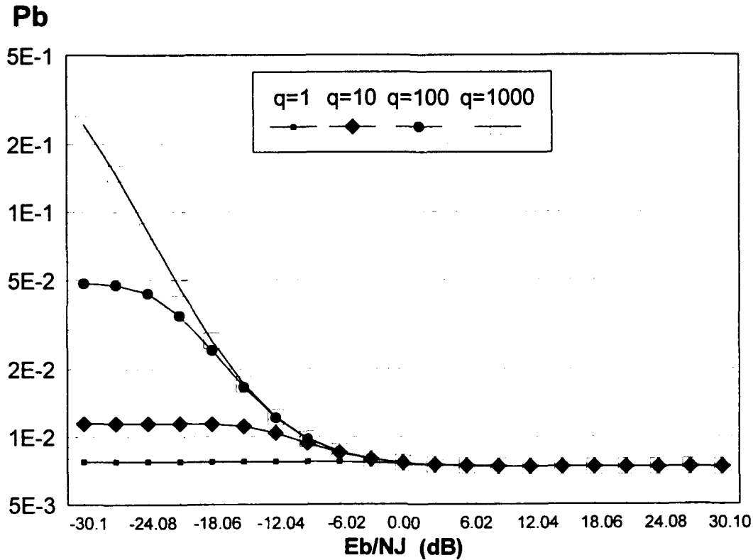
Figure 34. E_b/N_o=20\text{dB} , R_b=10 , R_j=10
