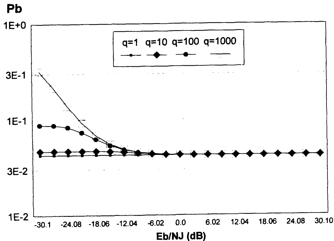
Figure 27. E_b/N_o=13.35\text{dB} , R_b=0 , R_j=100
