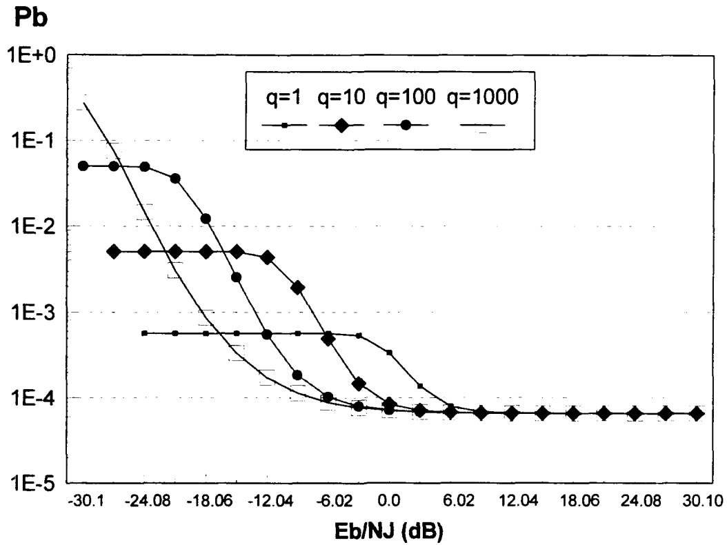
Figure 31. E_b/N_0=13.35\text{dB} , R_b=50 , R_j=50
