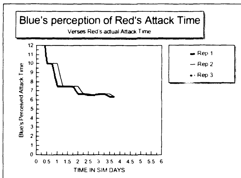
Figure 13. Attack Time
