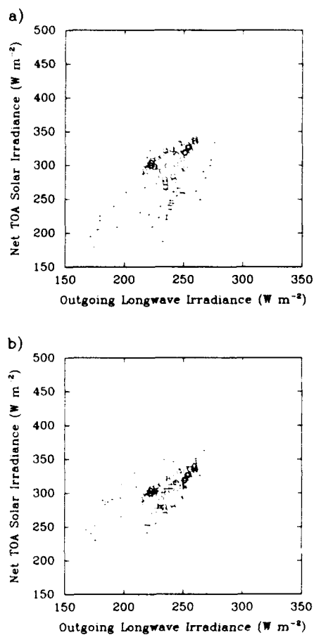
Figure 8. July mean TOA net solar irradiance for 9^{\circ} \times 9^{\circ} regions extending from 0^{\circ} to 9^{\circ}\text{N} plotted against July mean TOA outgoing longwave irradiance: (a) results from NOGAPS 3.3 (plus signs) and from ERB measurements (circles) and (b) results from NOGAPS 3.3MO (plus signs) and from ERB measurements (circles).
