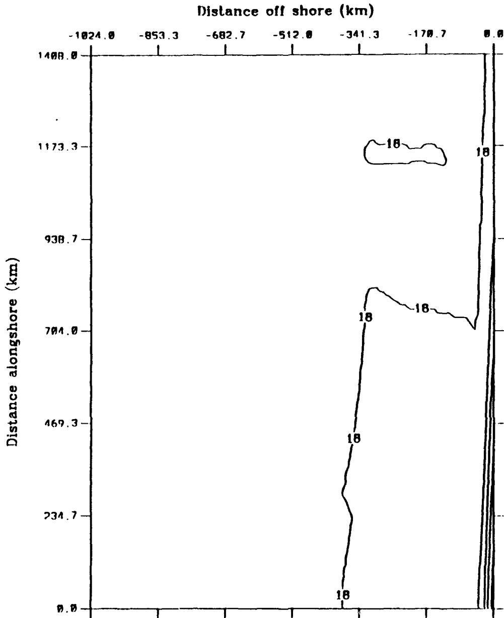
Temperature contour at model day 120.0
