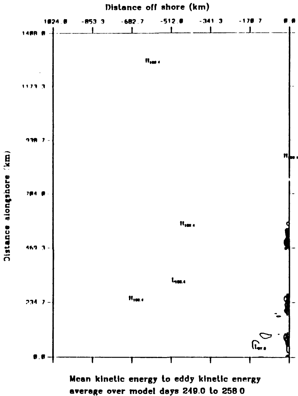
Figure C.5 Experiment 3: Energy transfers of mean to eddy kinetic energy (i.e., barotropic energy transfer) for 1983, for model days 249 to 258. The contour interval is 10 ergs \text{cm}^{-3} \text{s}^{-1} .
