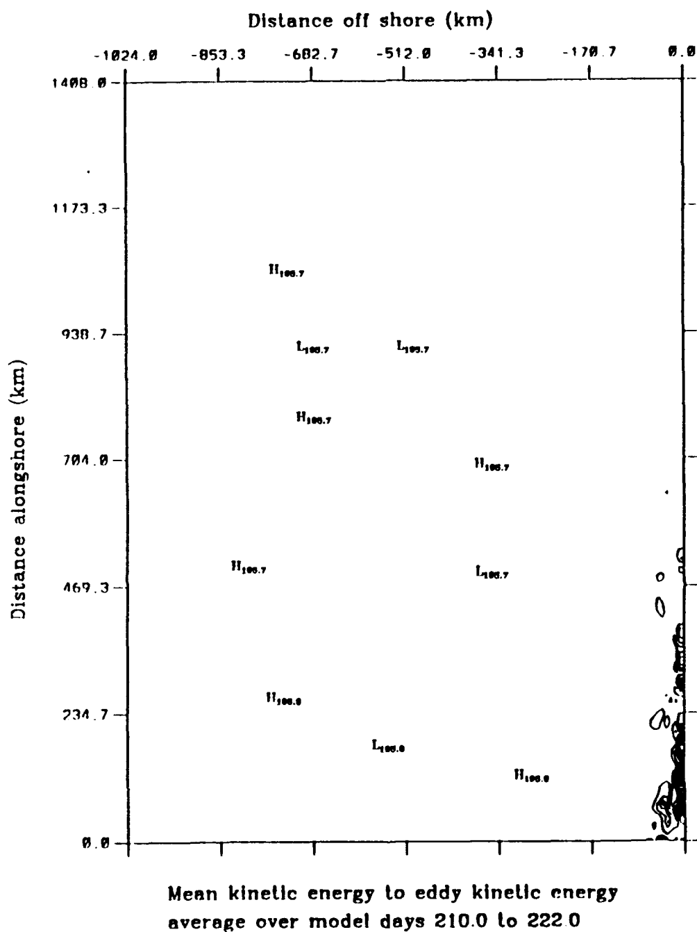
Figure B.1 Experiment 2: Energy transfers of mean to eddy kinetic energy (i.e., barotropic energy transfer) for 1981, for model days 210 to 222. The contour interval is 10 \text{ ergs cm}^{-3} \text{ s}^{-1} .
