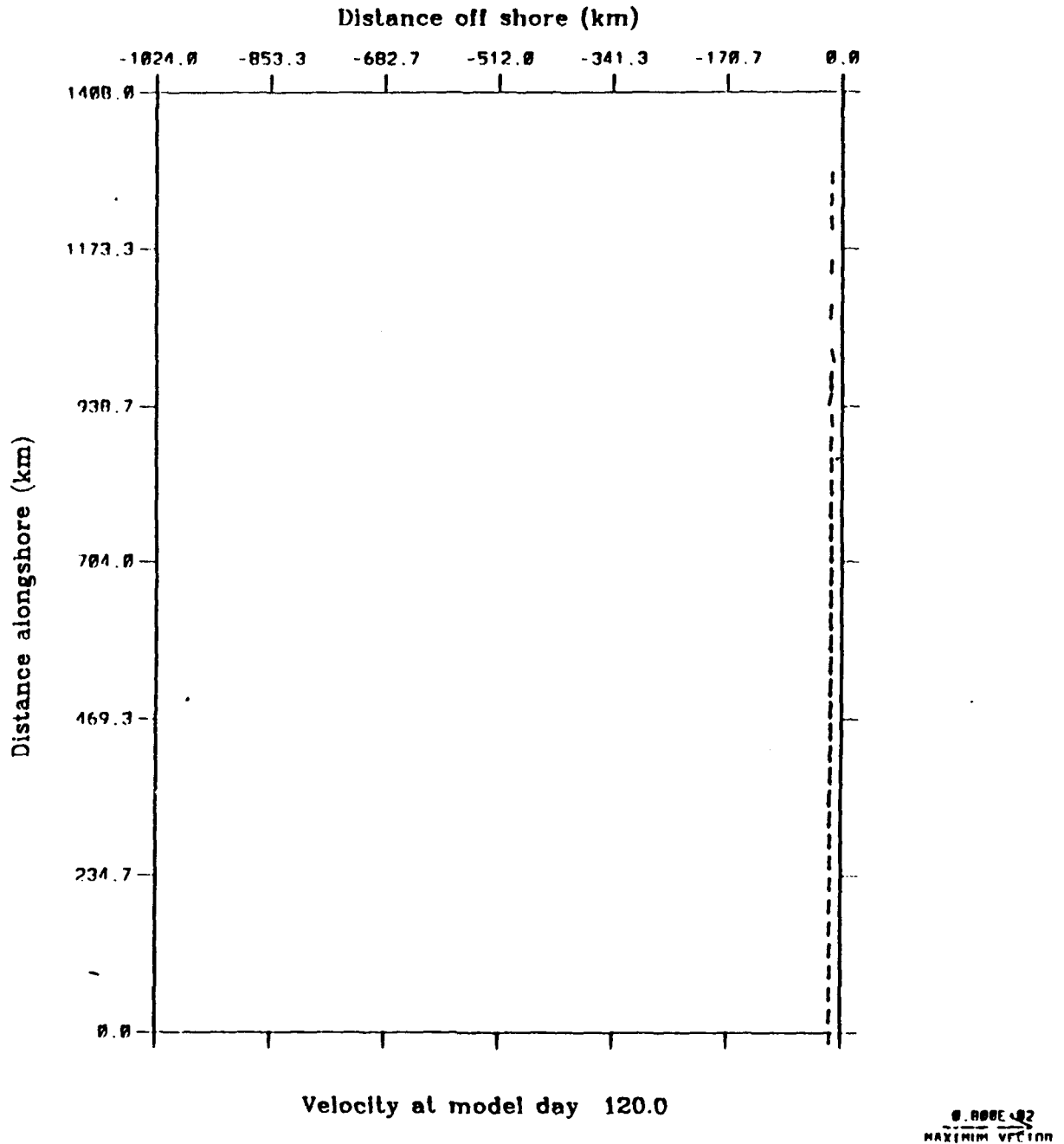
Figure 4.30 Experiment 3: Surface velocity vectors at day 120. To avoid clutter, velocity vectors are plotted at every third grid point in both the cross-shore and alongshore direction, and velocities less than 5 \text{ cm s}^{-1} are not plotted. Note equatorward surface current dominates. The number associated with the high at y \sim 250 \text{ km} corresponds to temperature, not velocity.
