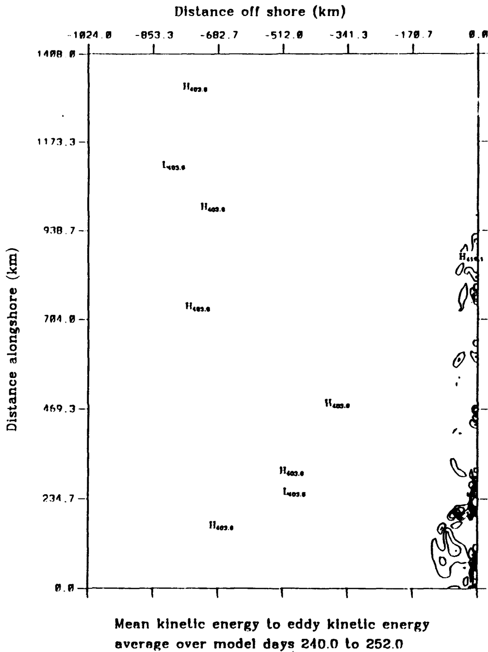
Figure B.3 Experiment 2: Energy transfers of mean to eddy kinetic energy (i.e., barotropic energy transfer) for 1981, for model days 240 to 252. The contour interval is 10 \text{ergs cm}^{-3} \text{ s}^{-1} .
