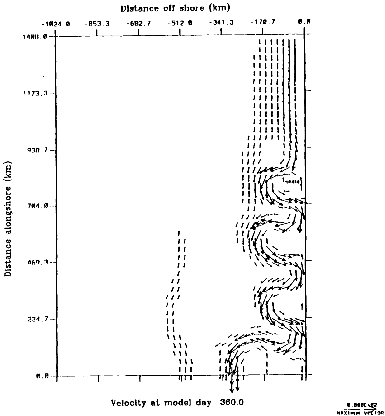
Figure 4.12 Experiment 1: Surface velocity vectors at day 360 as in Figure 4.3. Note equatorward surface current over a poleward undercurrent. The number associated with the low at y \sim 800 km corresponds to temperature, not velocity.
