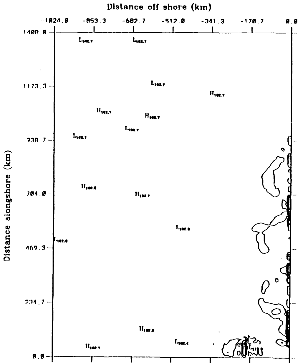
Eddy potential energy to eddy kinetic energy average over model days 309.0 to 333.0
