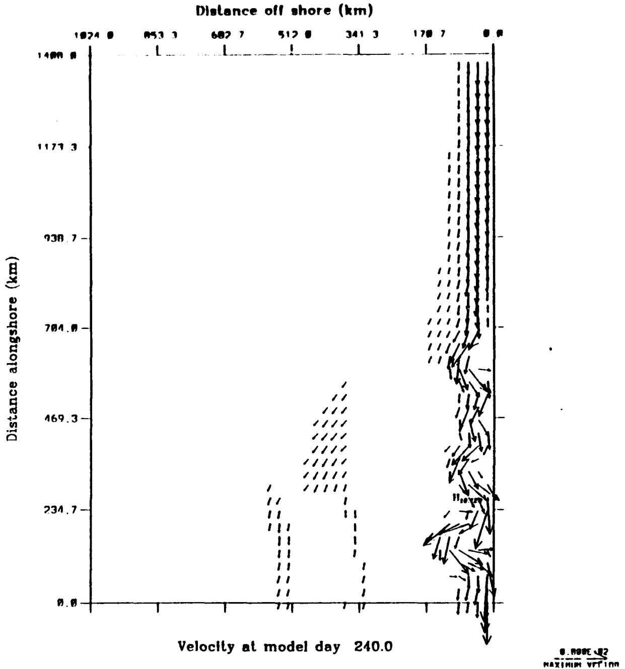
Figure 4.34 Experiment 3: Surface velocity vectors at day 240. To avoid clutter, velocity vectors are plotted at every third grid point in both the cross-shore and alongshore direction, and velocities less than 5 \text{ cm s}^{-1} are not plotted. The number associated with the high at y \sim 250 km corresponds to temperature, not velocity. Note existence of eddies.
