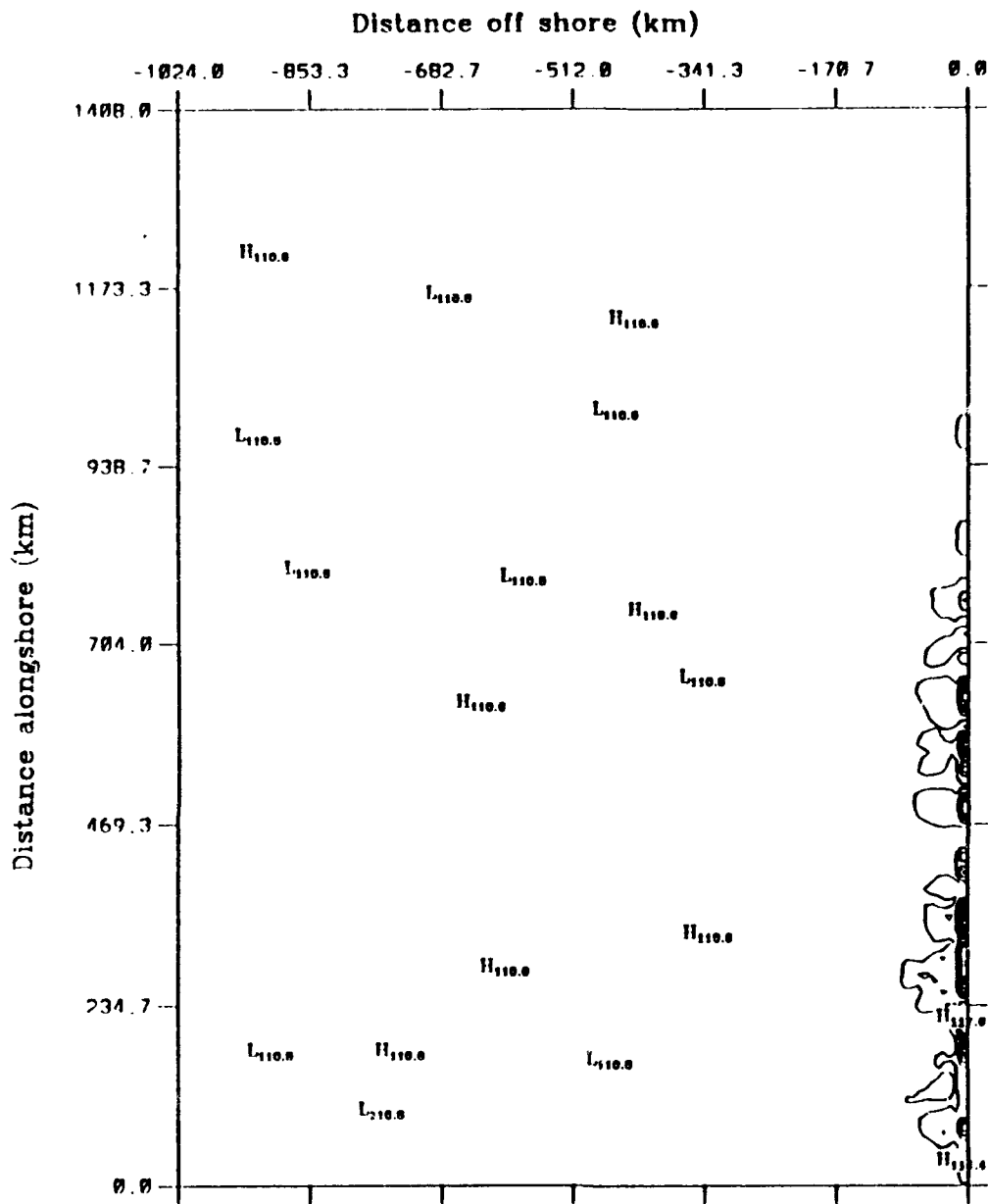
Eddy potential energy to eddy kinetic energy average over model days 186.0 to 192.0
