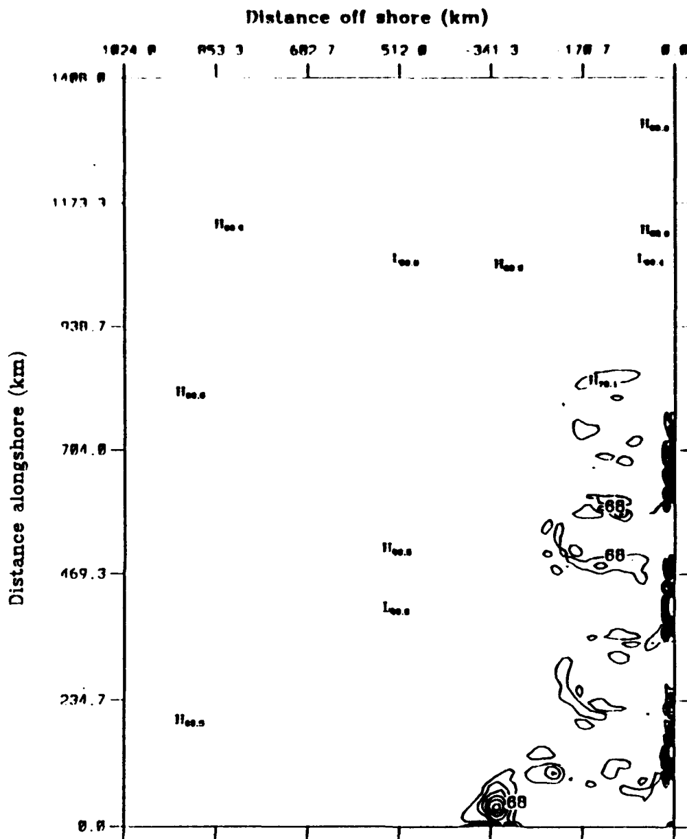
Mean kinetic energy to eddy kinetic energy average over model days 378.0 to 408.0
