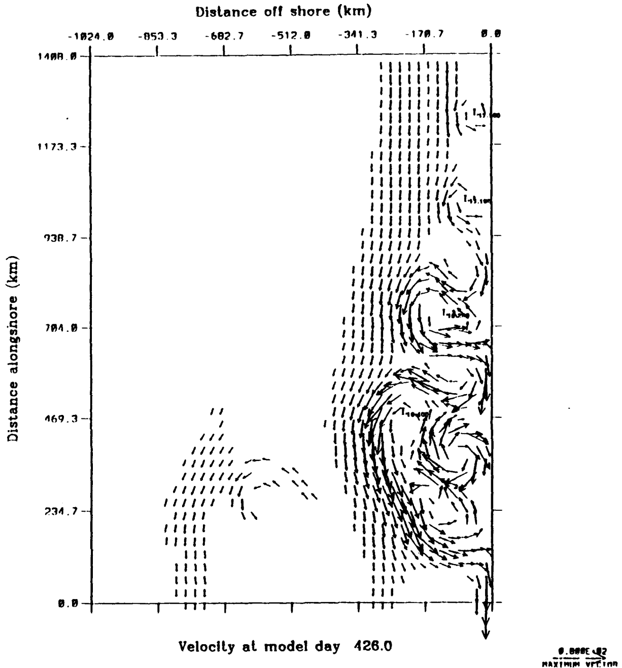
Figure 4.53 Experiment 5: Surface velocity vectors at day 426 (yd 60). To avoid clutter, velocity vectors are plotted at every third grid point in both the cross-shore and alongshore direction, and velocities less than 5 \text{ cm s}^{-1} are not plotted. The numbers associated with the lows embedded in the meanders and eddies along the coast correspond to temperature, not velocity.
