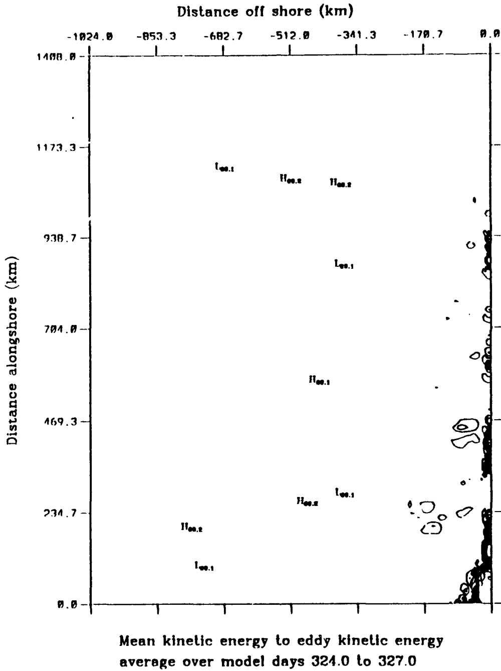
Figure C.11 Experiment 3: Energy transfers of mean to eddy kinetic energy (i.e., barotropic energy transfer) for 1983, for model days 324 to 327. The contour interval is 1 ergs \text{cm}^{-3} \text{s}^{-1} .
