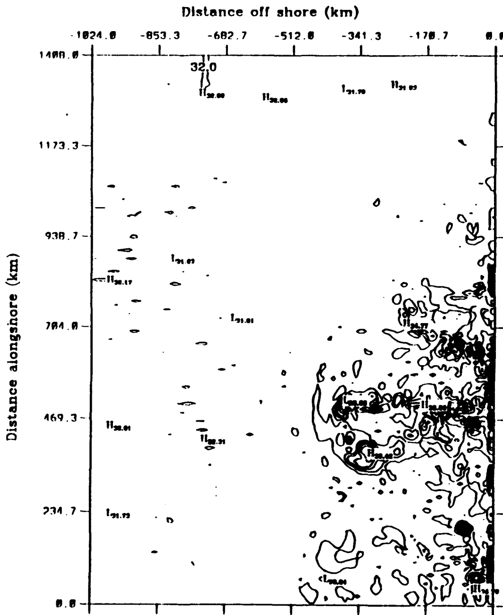
Eddy potential energy to eddy kinetic energy average over model days 624.0 to 636.0
