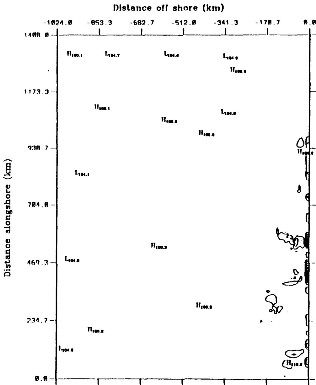
Eddy potential energy to eddy kinetic energy average over model days 606.0 to 624.0
