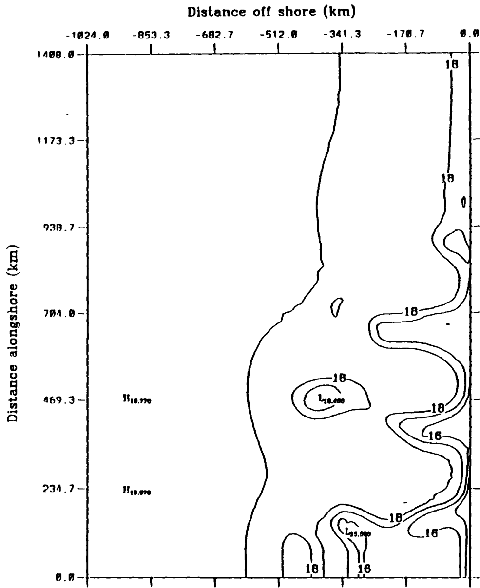
Temperature contour at model day 726.0
