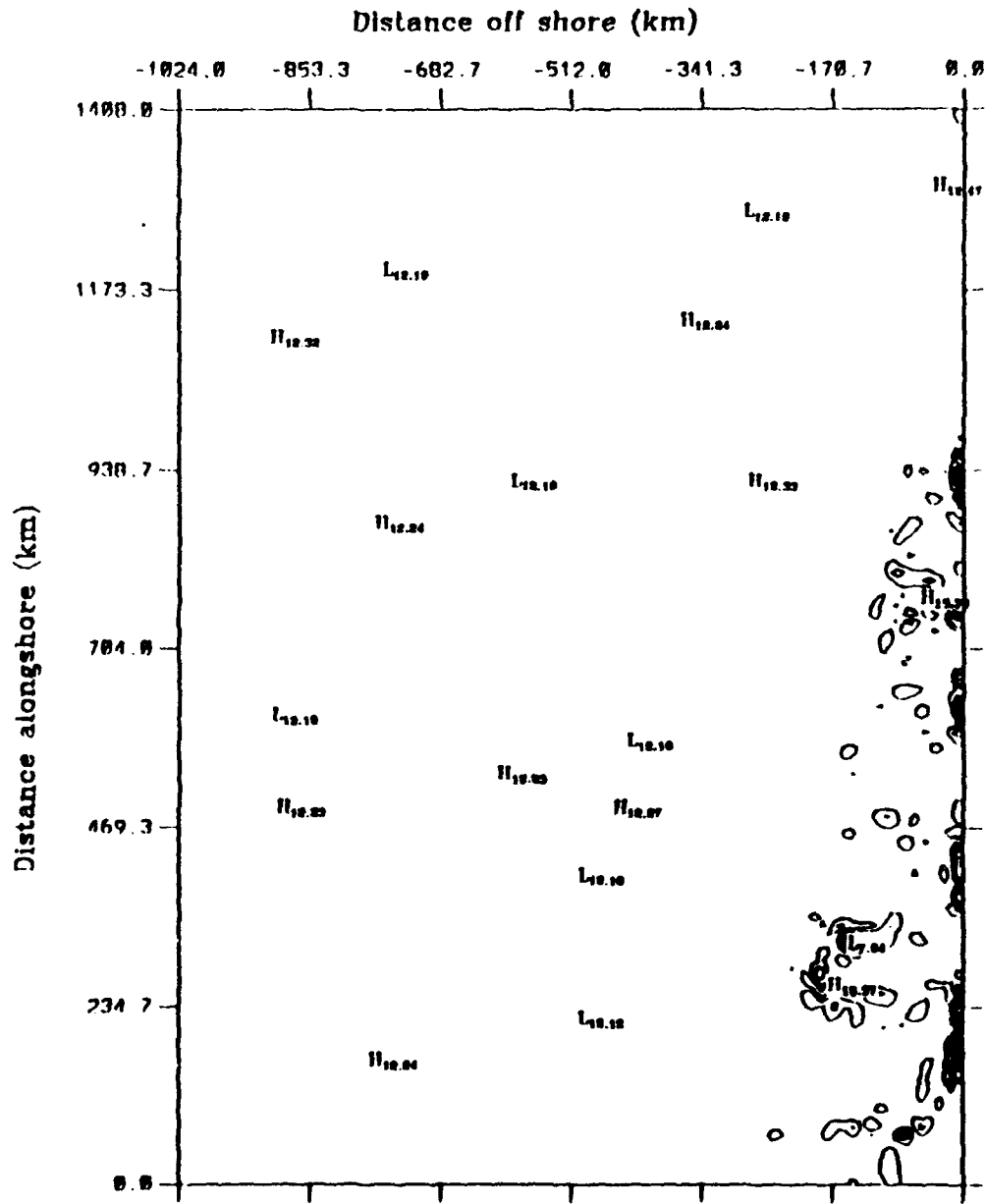
Mean kinetic energy to eddy kinetic energy average over model days 312.0 to 315.0
