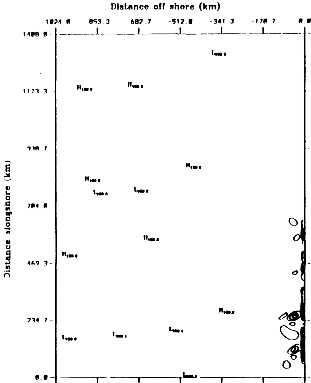
Eddy potential energy to eddy kinetic energy average over model days 222.0 to 234.0
