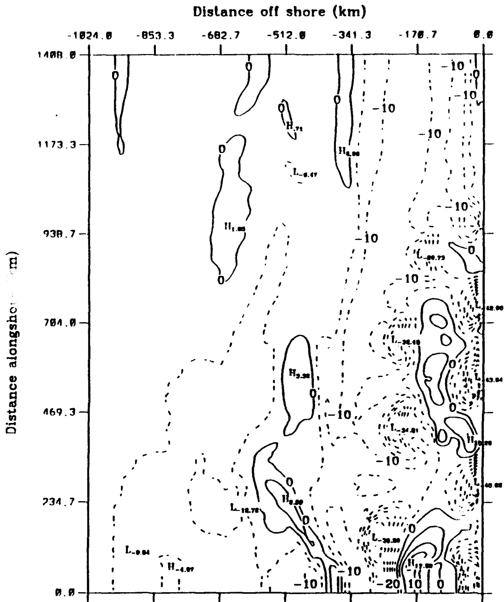
North-South vel contour at model day 426.0
