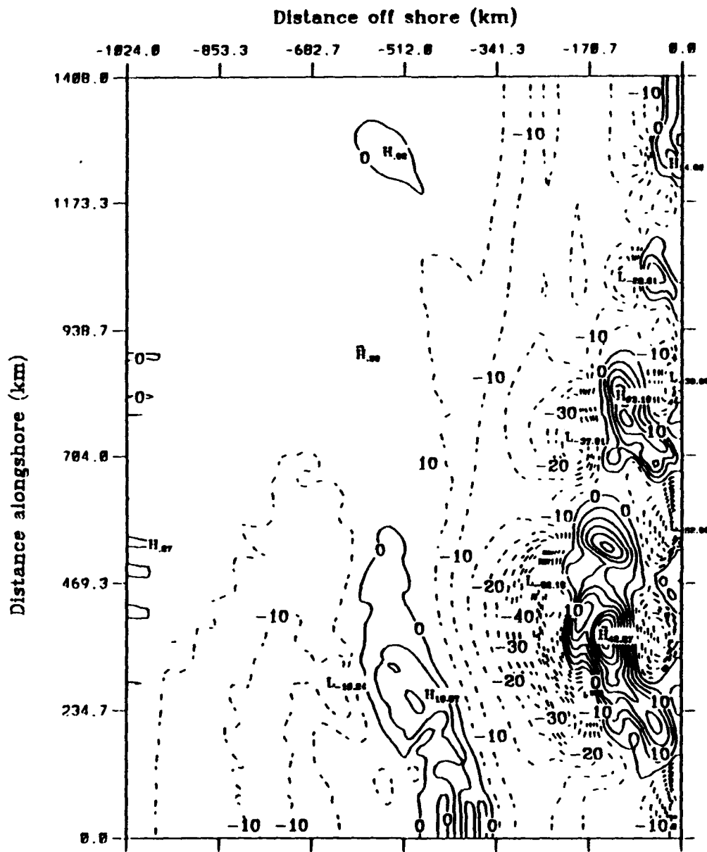
North-South vel contour at model day 426.0
