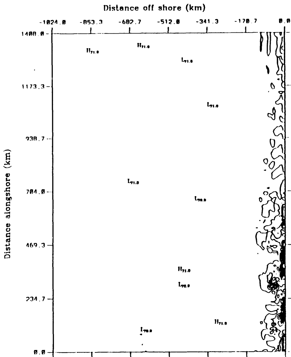
Mean kinetic energy to eddy kinetic energy average over model days 228.0 to 231.0
