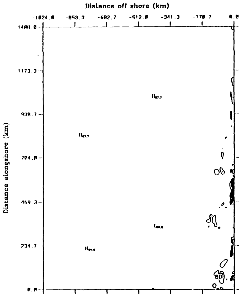
Mean kinetic energy to eddy kinetic energy average over model days 576.0 to 591.0
