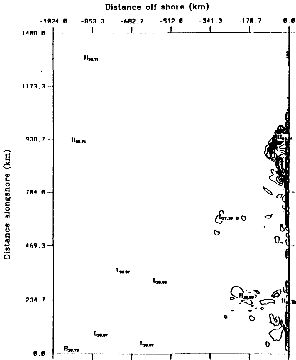
Eddy potential energy to eddy kinetic energy average over model days 504.0 to 516.0
