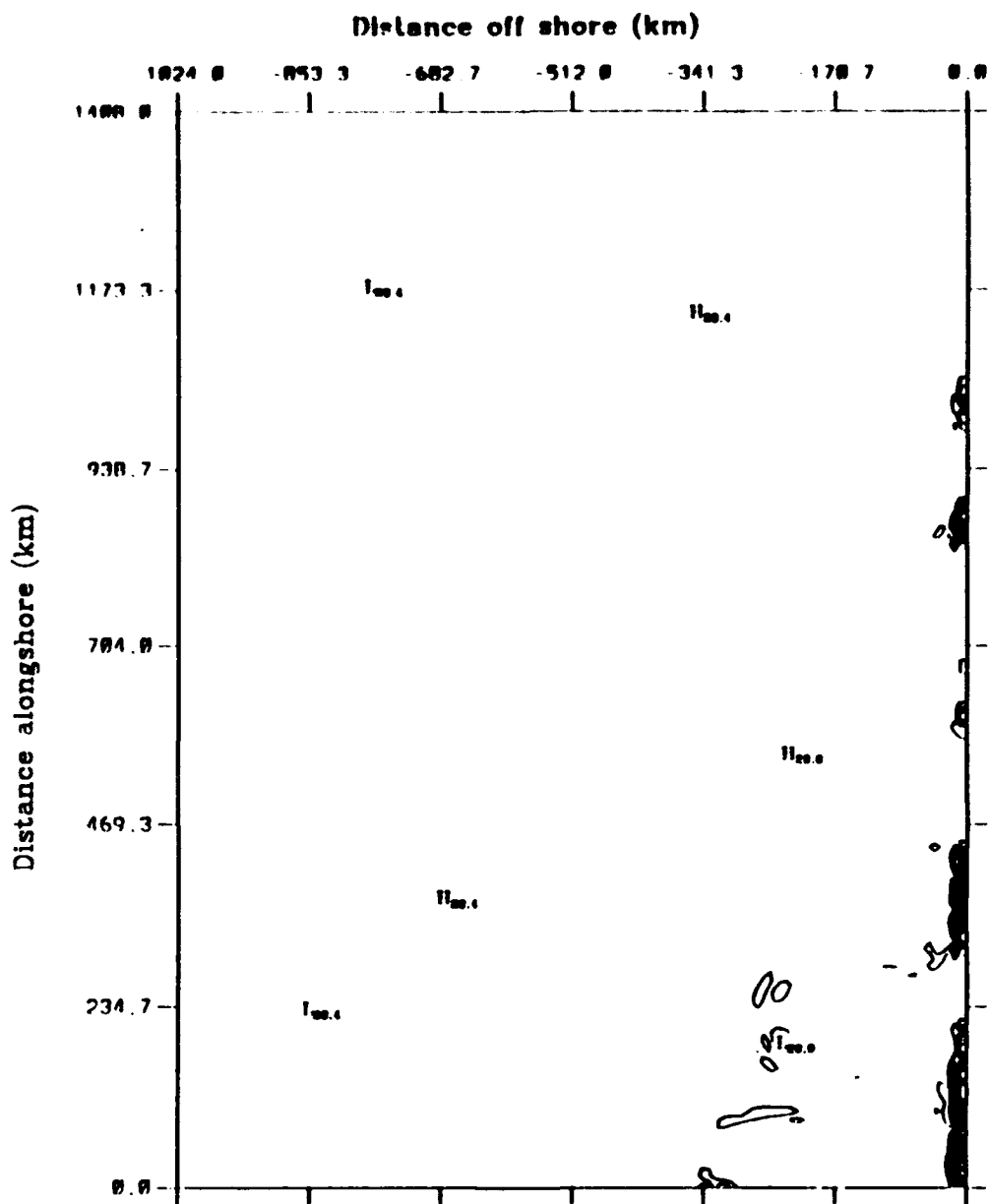
Mean kinetic energy to eddy kinetic energy average over model days 453.0 to 465.0
