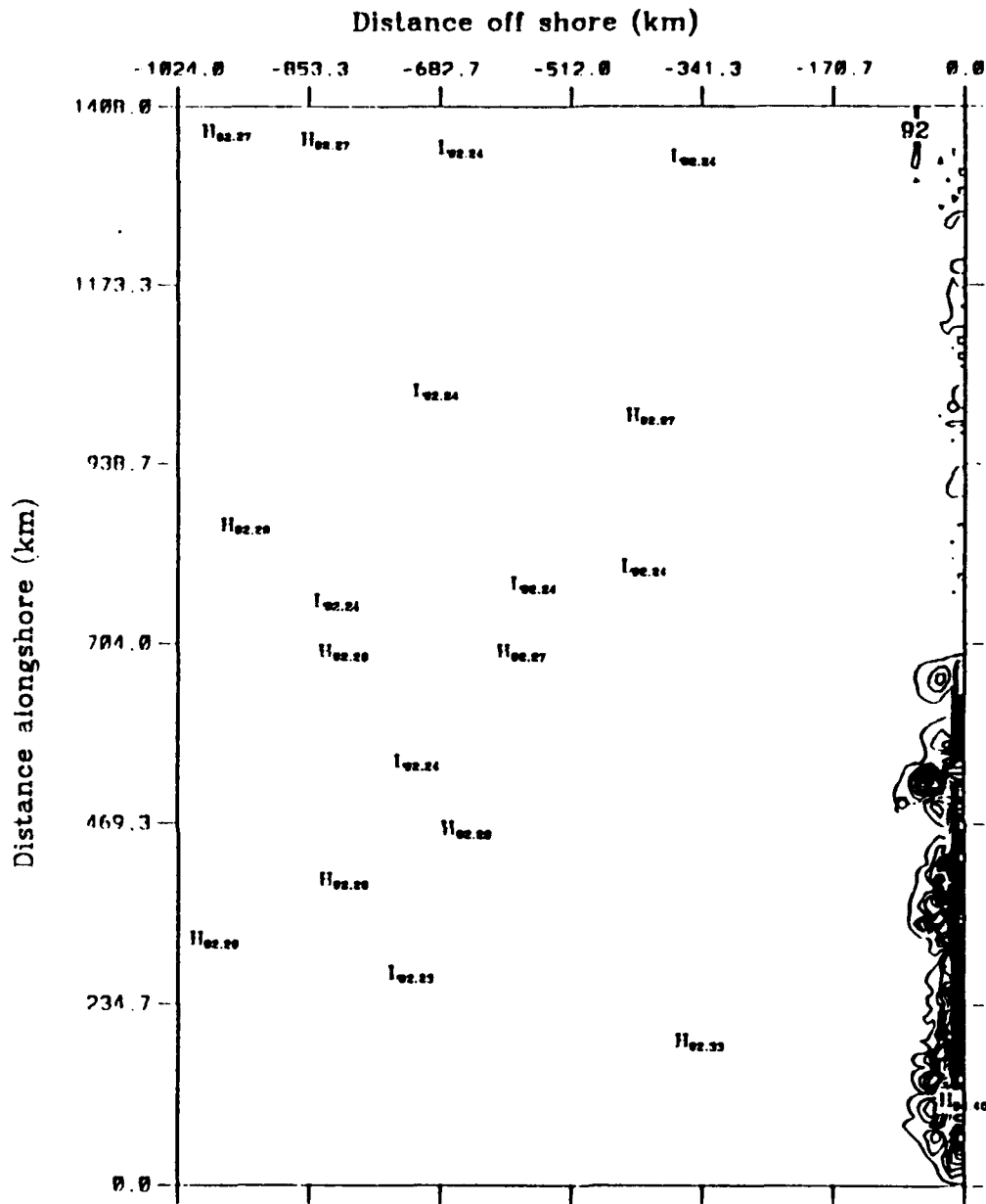
Fddy potential energy to eddy kinetic energy average over model days 207.0 to 216.0
