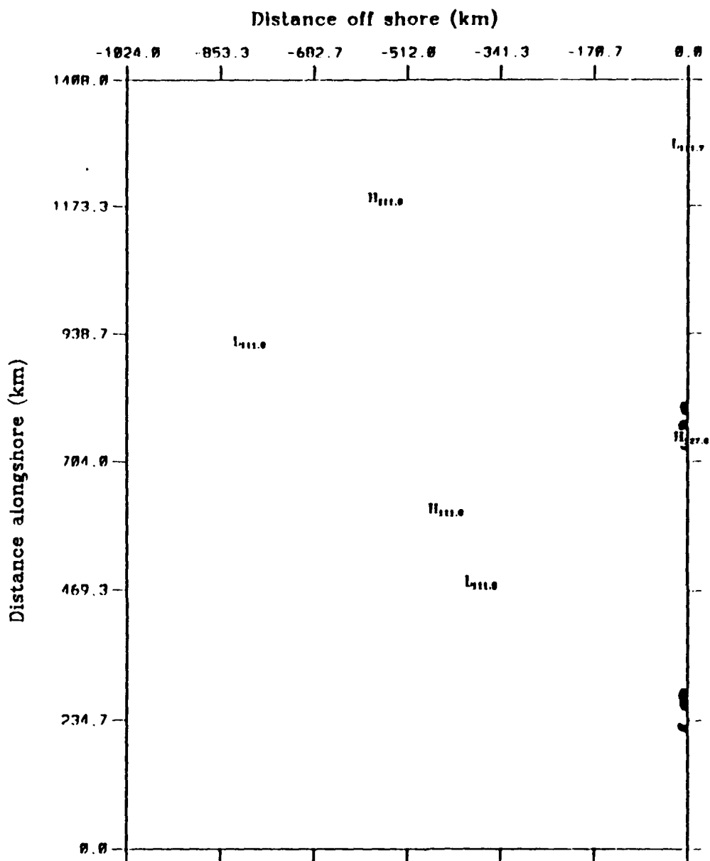
Mean kinetic energy to eddy kinetic energy average over model days 297.0 to 303.0
