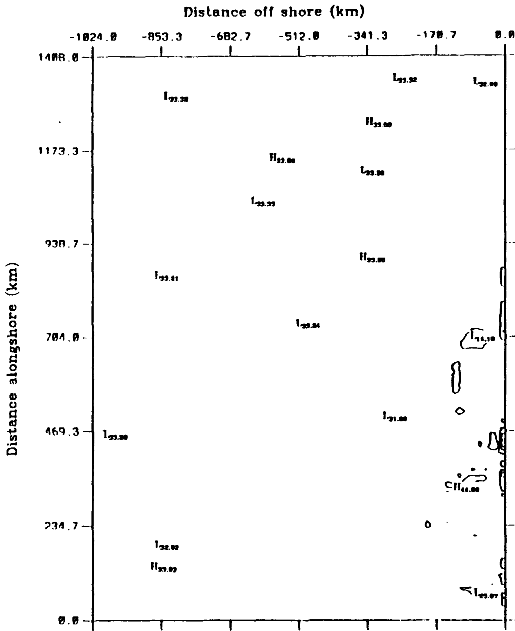
Eddy potential energy to eddy kinetic energy average over model days 645.0 to 657.0
