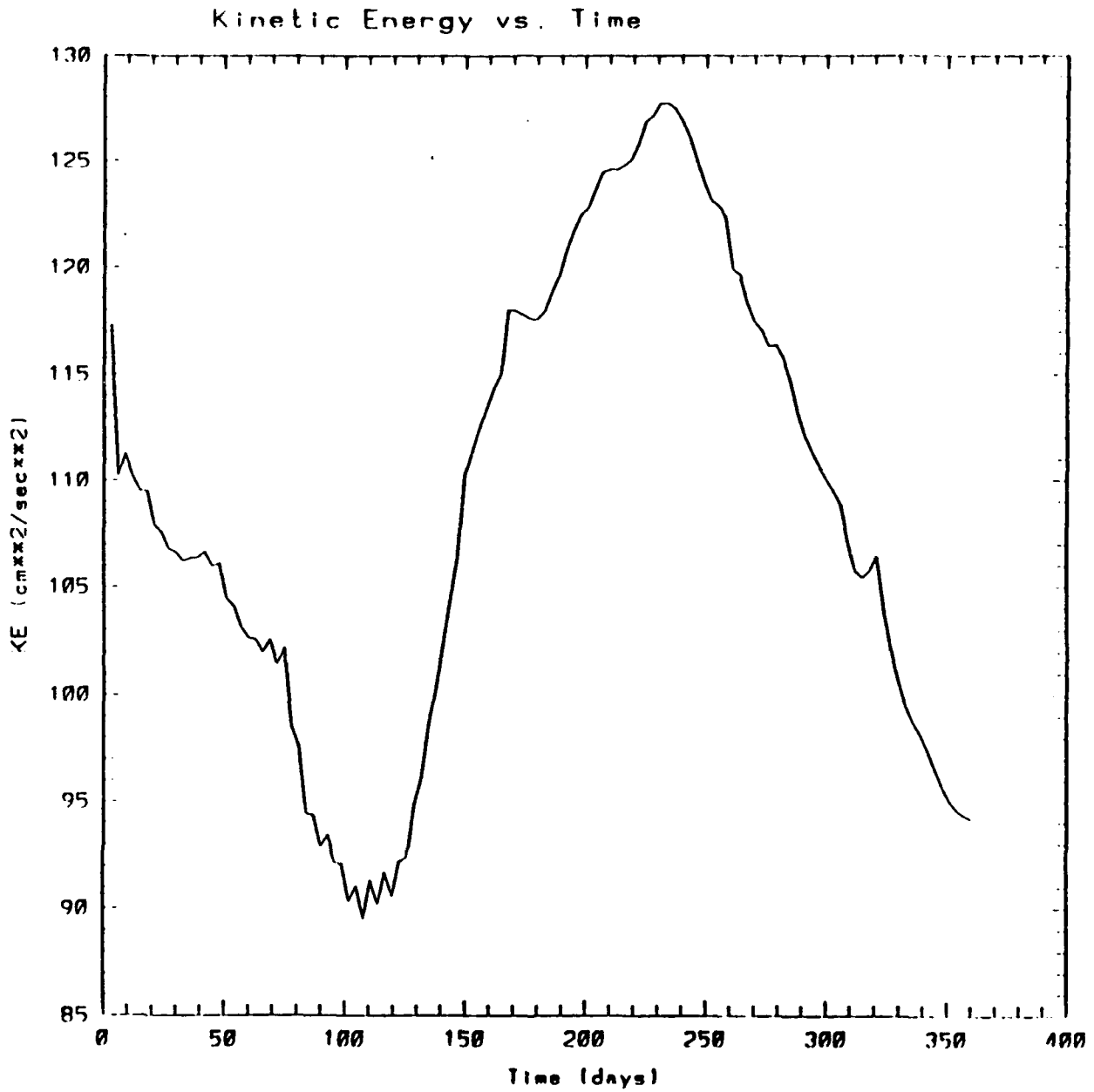
Figure 4.69 Experiment 8: Total kinetic energy per unit mass time series for 1983 over the entire domain (Units of the kinetic energy are \text{cm}^2\text{s}^{-2} ). Peak value of 128 \text{ cm}^2\text{s}^{-2} at day 963 (yd 233).
