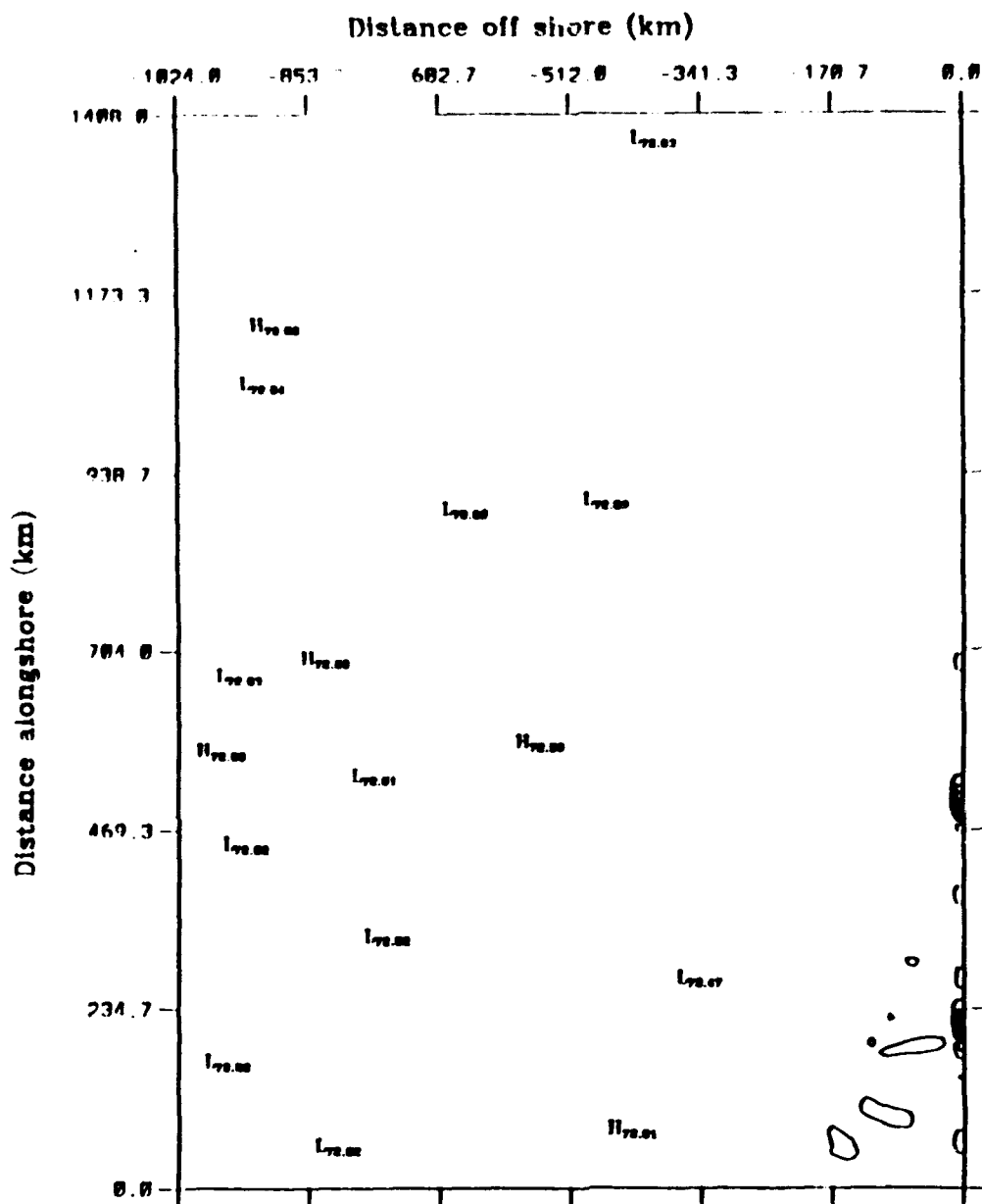
Eddy potential energy to eddy kinetic energy average over model days 249.0 to 258.0
