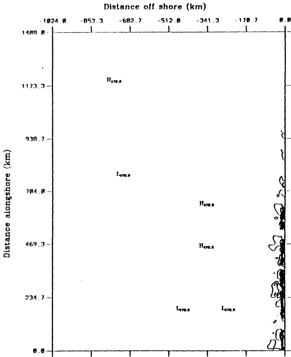
Mean kinetic energy to eddy kinetic energy average over model days 186.0 to 192.0
