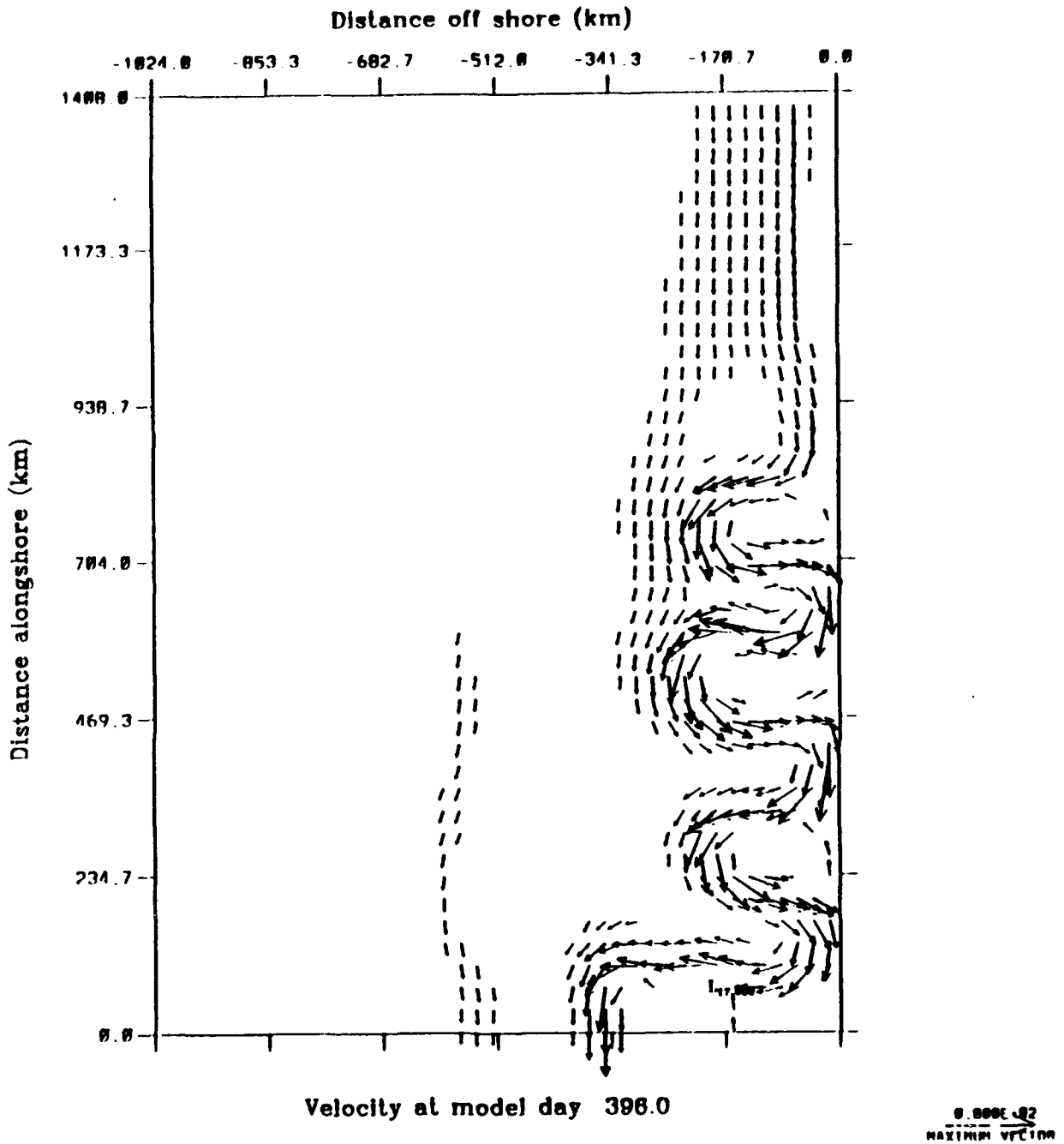
Figure 4.39 Experiment 4: Surface velocity vectors at day 396 (yd 30). To avoid clutter, velocity vectors are plotted at every third grid point in both the cross-shore and alongshore direction, and velocities less than 5 \text{ cm s}^{-1} are not plotted. The number associated with the low at y=80 \text{ km} corresponds to temperature, not velocity. Note equatorward surface current with embedded meanders and cyclonic eddies.
