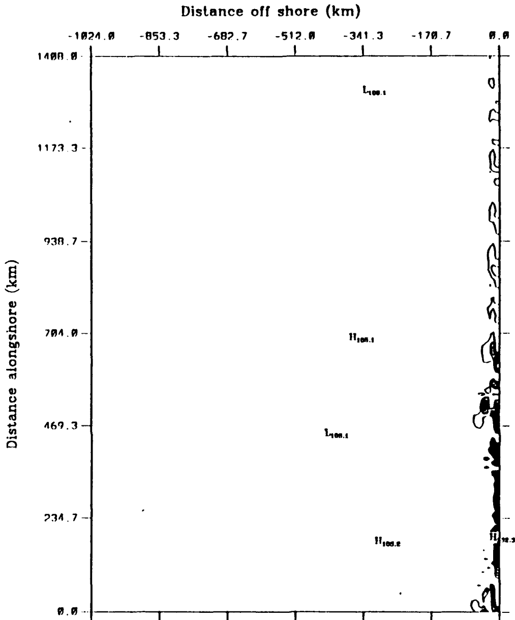
Mean kinetic energy to eddy kinetic energy average over model days 207.0 to 216.0
