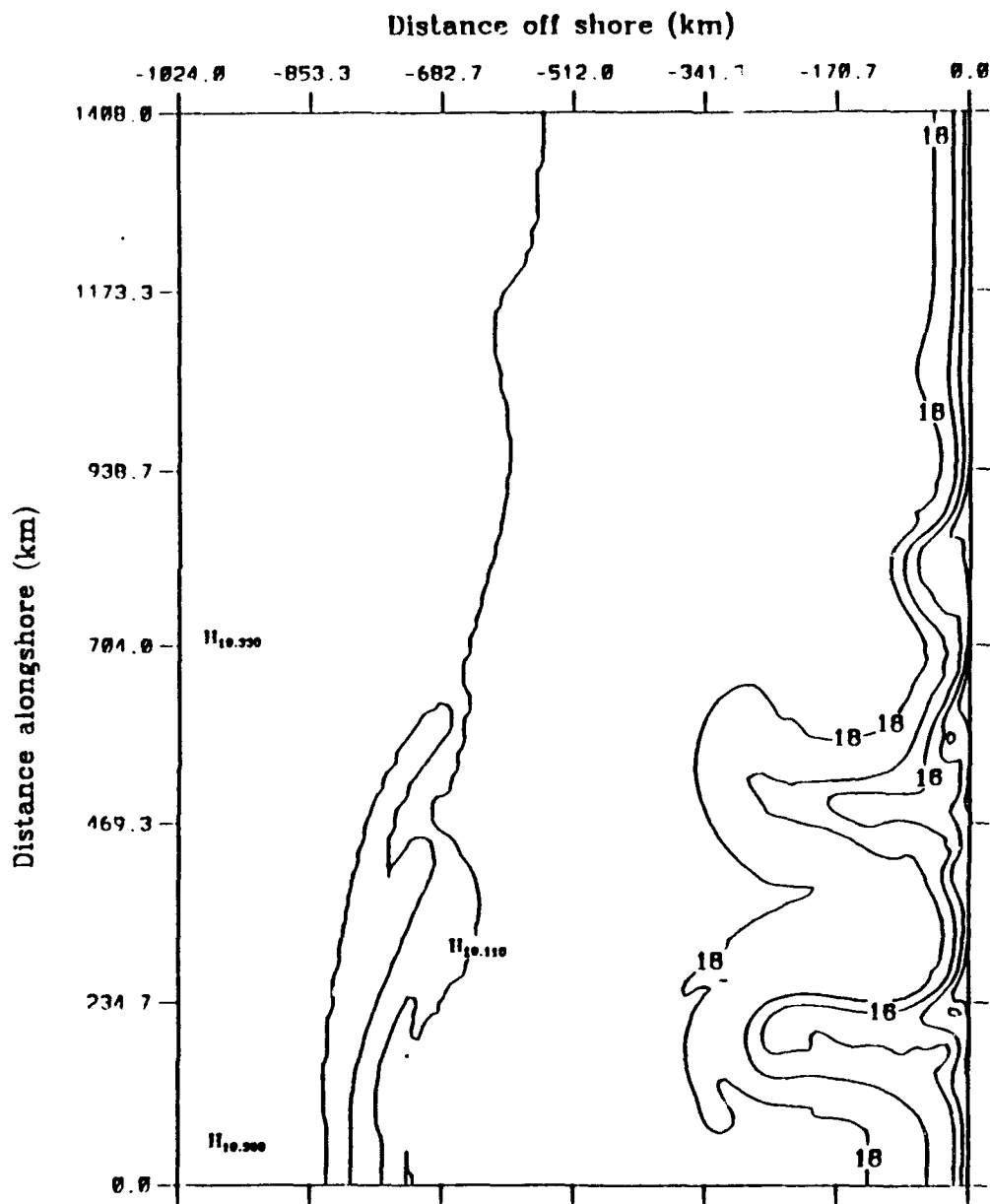
Temperature contour at model day 546.0
