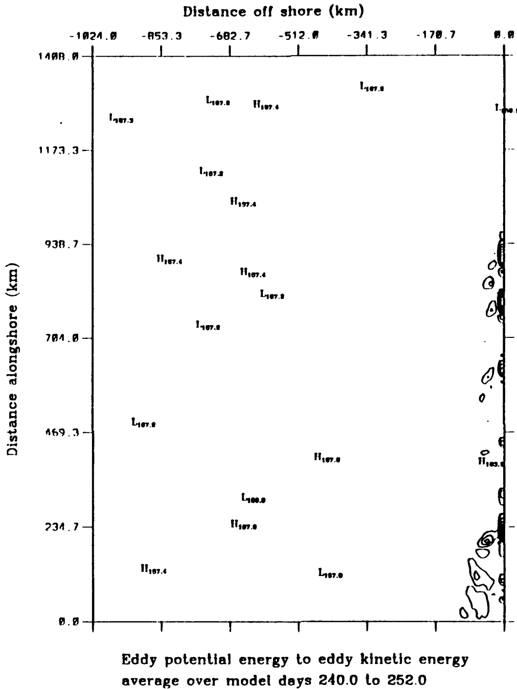
Figure B.4 Experiment 2: Energy transfers of eddy potential to eddy kinetic energy (i.e., baroclinic energy transfer) for 1981, for model days 240 to 252. The contour interval is 10 \text{ ergs cm}^{-3} \text{ s}^{-1} .
