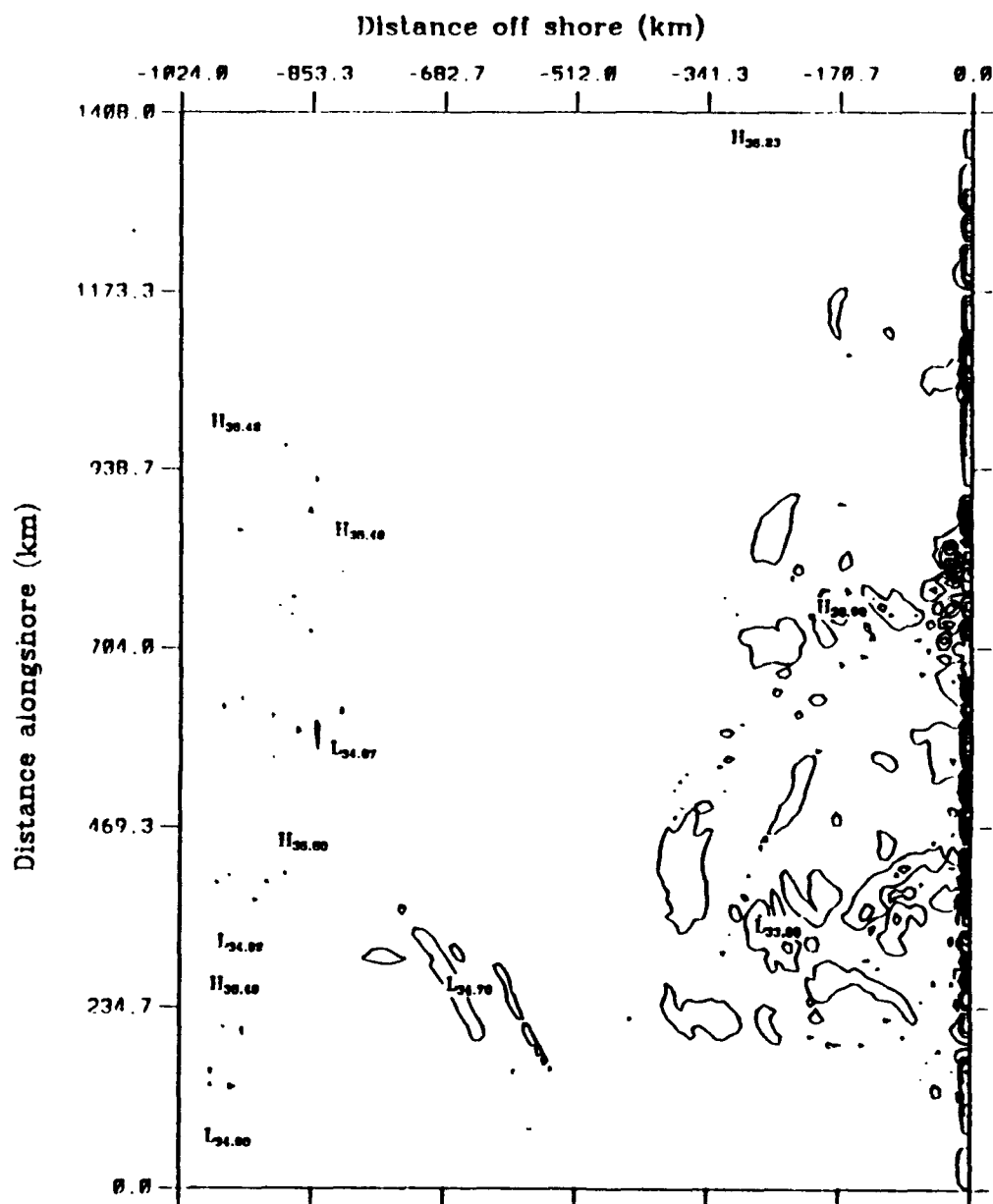
Eddy potential energy to eddy kinetic energy average over model days 507.0 to 516.0
