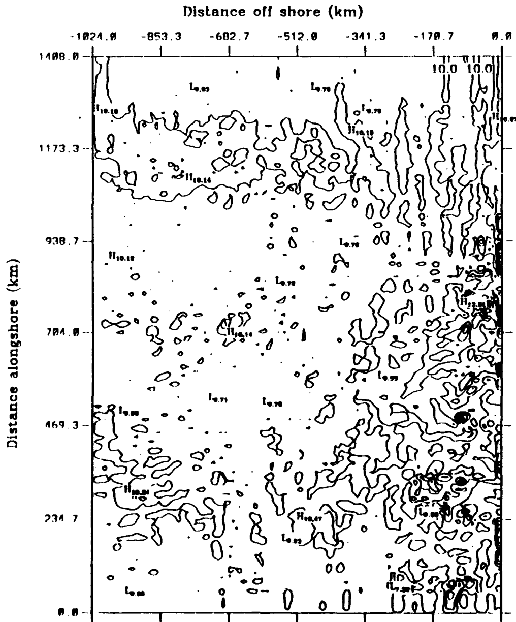
Eddy potential energy to eddy kinetic energy average over model days 312.0 to 315.0
