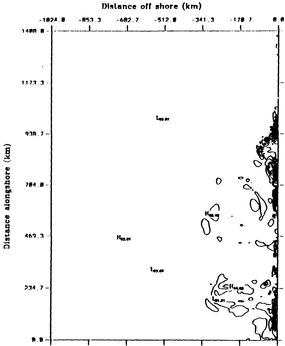
Mean kinetic energy to eddy kinetic energy average over model days 504.0 to 516.0
