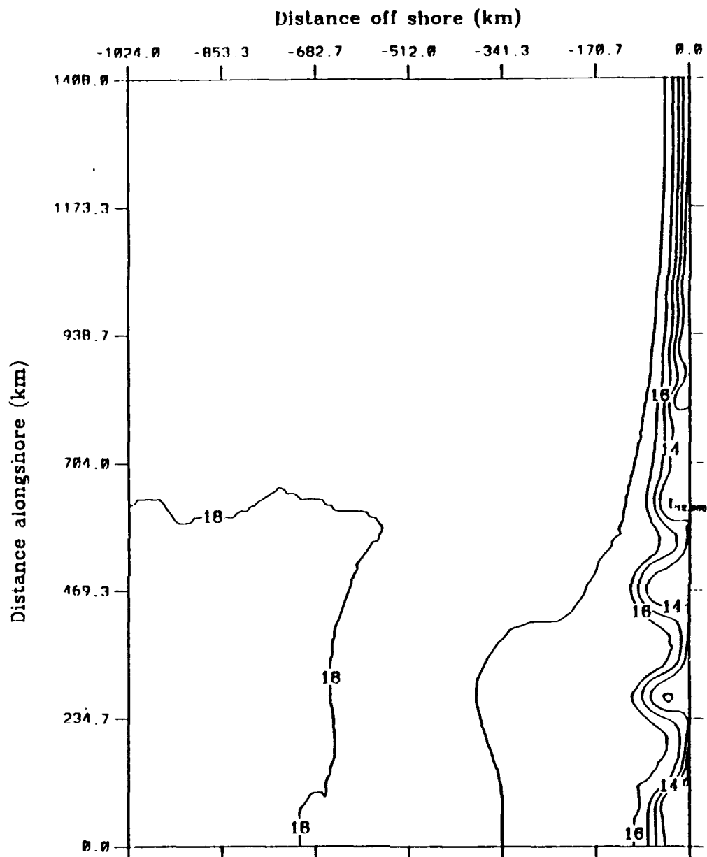
Temperature contour at model day 240.0
