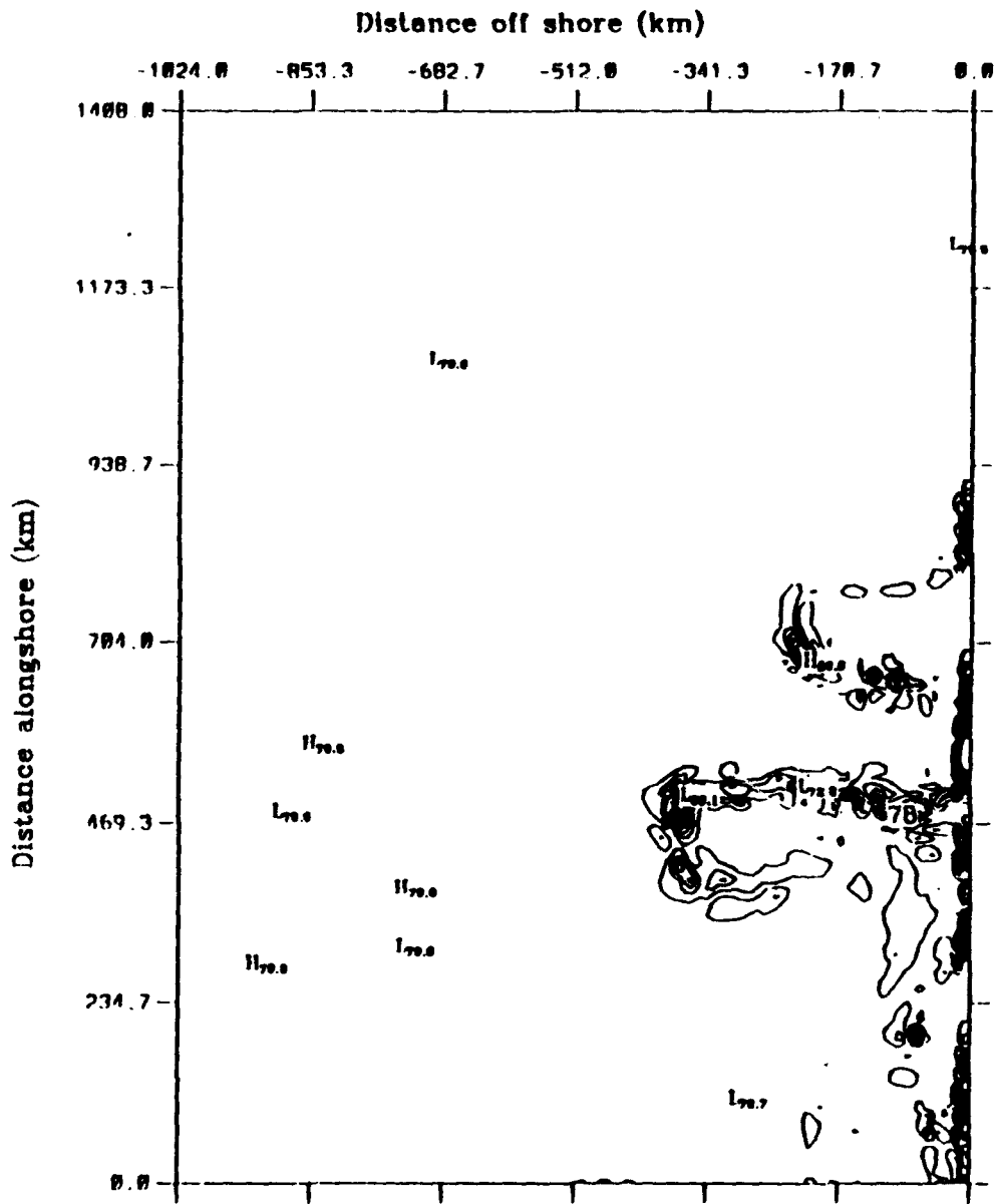
Mean kinetic energy to eddy kinetic energy average over model days 624.0 to 636.0
