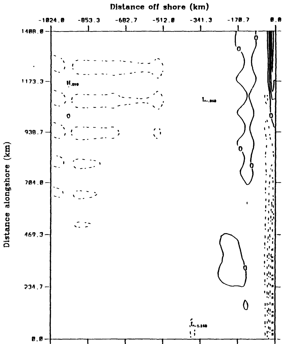
North-South vel contour at model day 30.0
