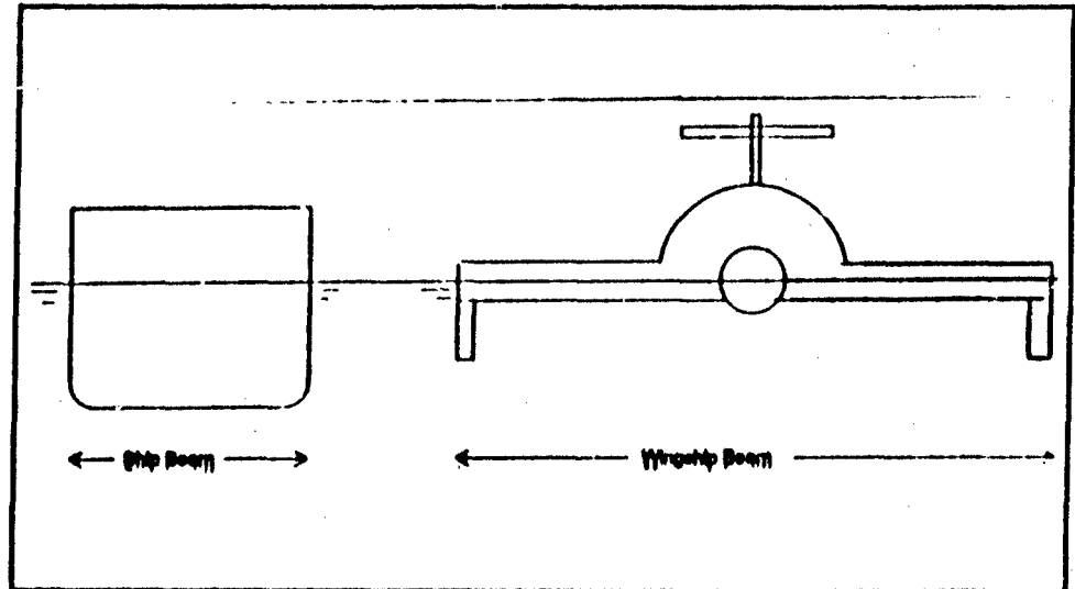
Figure 21: Wingship Stability Comparison
