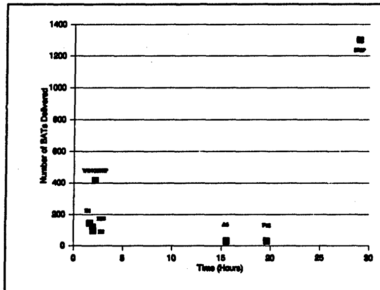
Figure 10: Ordnance Delivery Effectiveness
