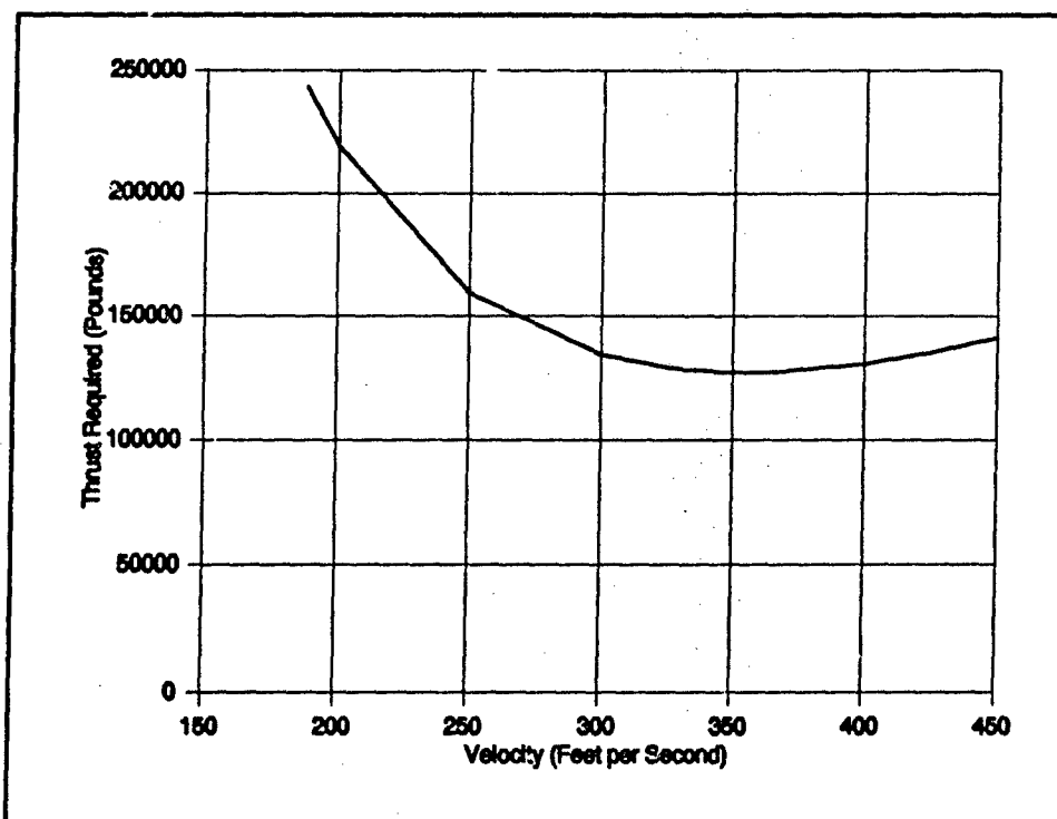
Figure 25: Takeoff Thrust Required
