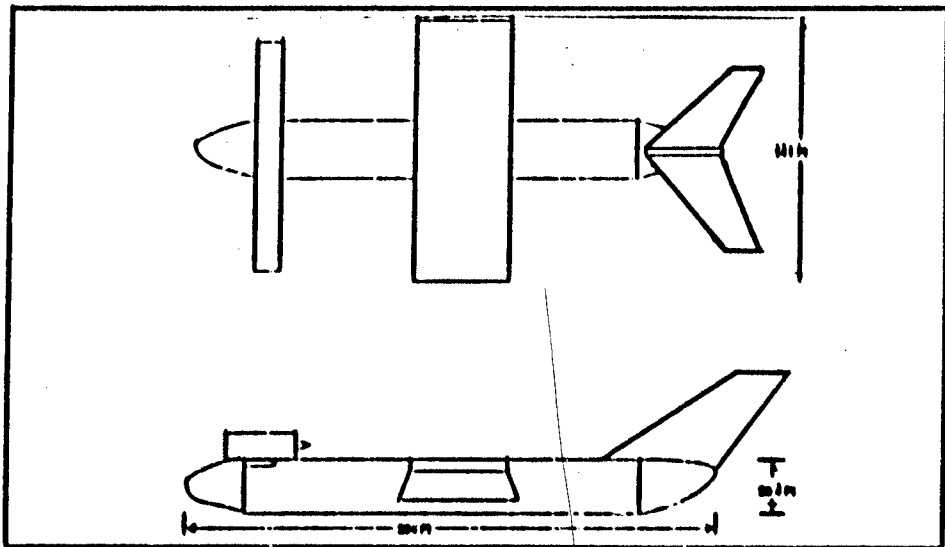
Figure 1: Wingship Schematic
