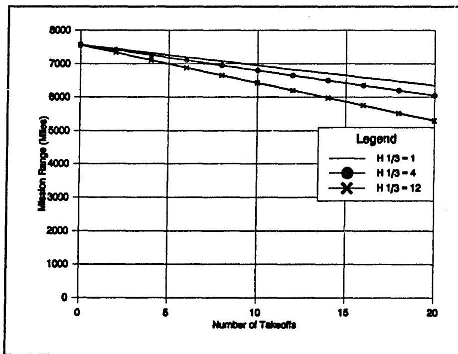
Figure 27: Mission Range Versus Number of Takeoffs
