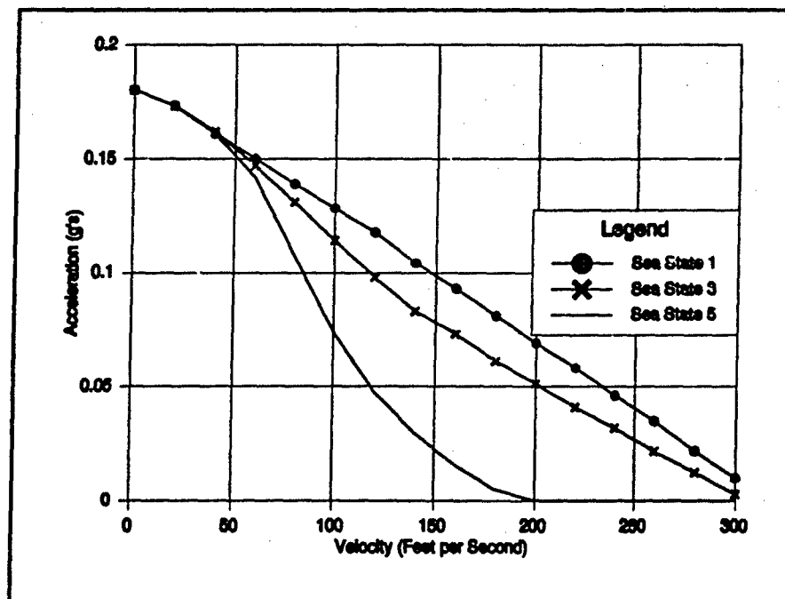
Figure 17: Takeoff Acceleration, 200 kt Takeoff Velocity
