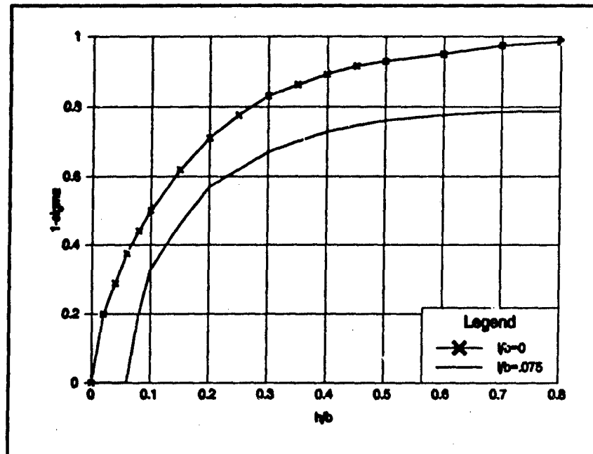
Figure 4: Endplate Effect on Correction Factor
