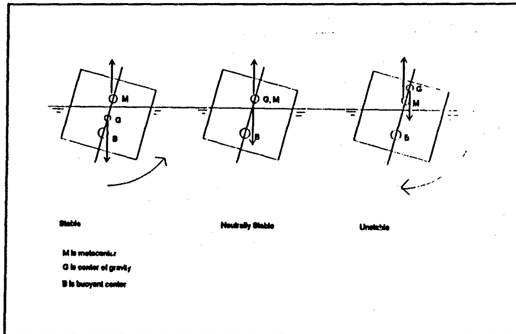
Figure 20: Stability Classification
