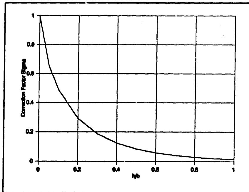
Figure 2: Height Correction Factor
