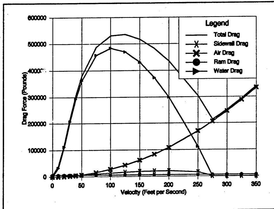
Figure 24: Takeoff Drag
