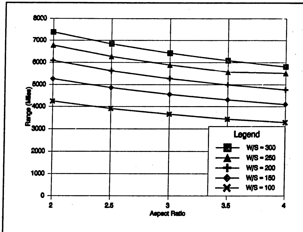
Figure 12: Wingship Range Map
