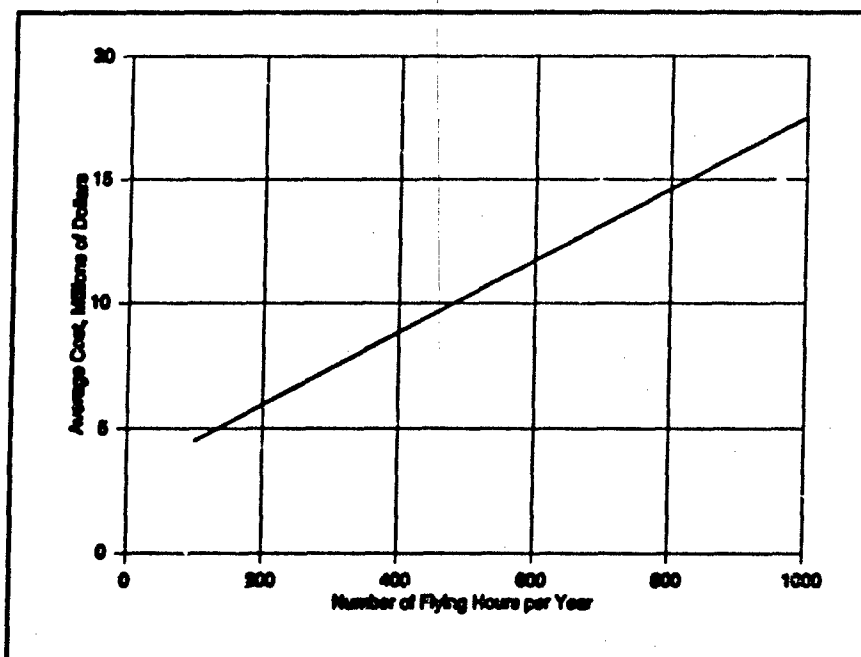
Figure 36: Average Operating Cost Versus Annual Flight Hours
