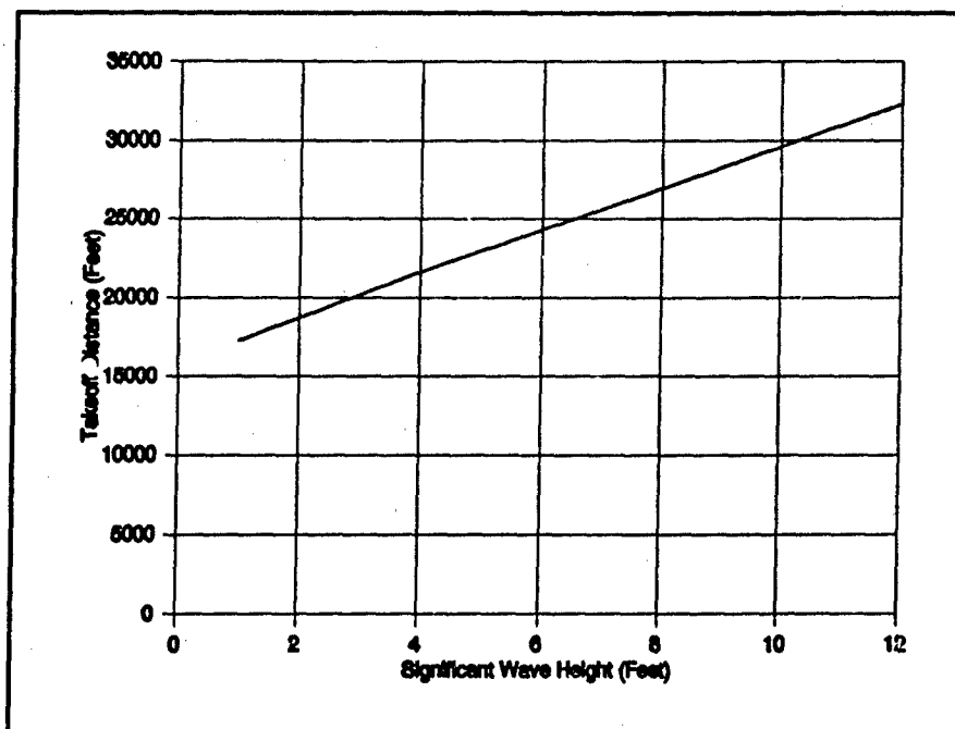
Figure 16: Takeoff Distance Versus Sea State
