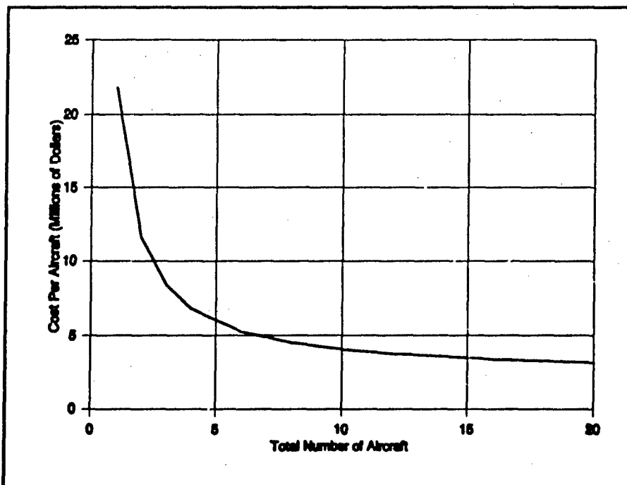
Figure 34: Average Wingship Operating Cost Versus Number of Aircraft
