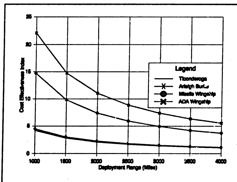
Figure 45: Effectiveness Comparison
