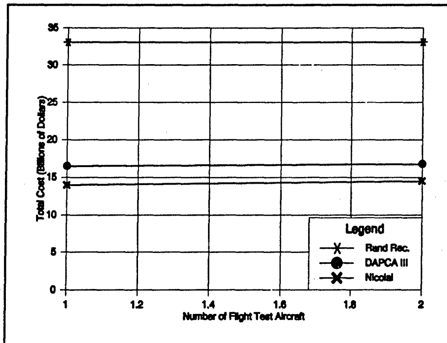
Figure 32: Total Wingship Program Cost Versus Number of Flight Test Aircraft
