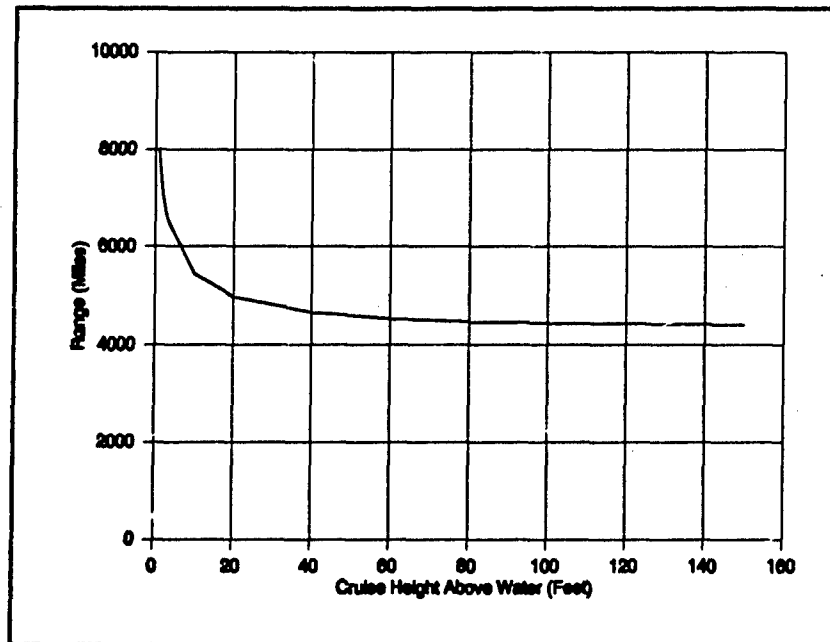
Figure 15: Range Versus Cruising Height
