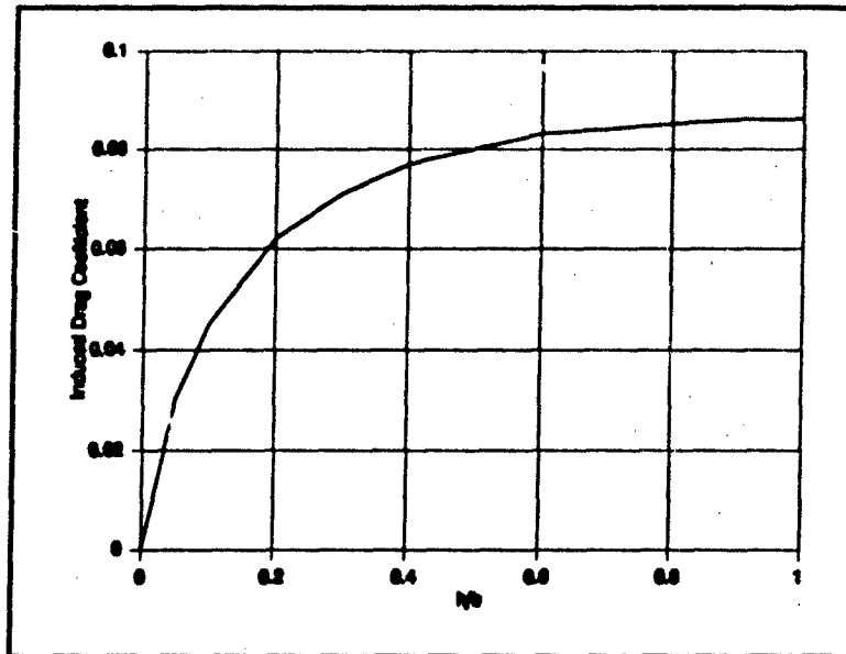
Figure 3: Example Induced Drag
