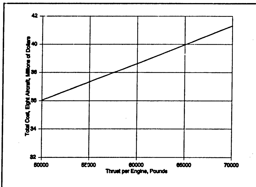
Figure 39: Total Wingship Operating Cost Versus Engine Thrust
