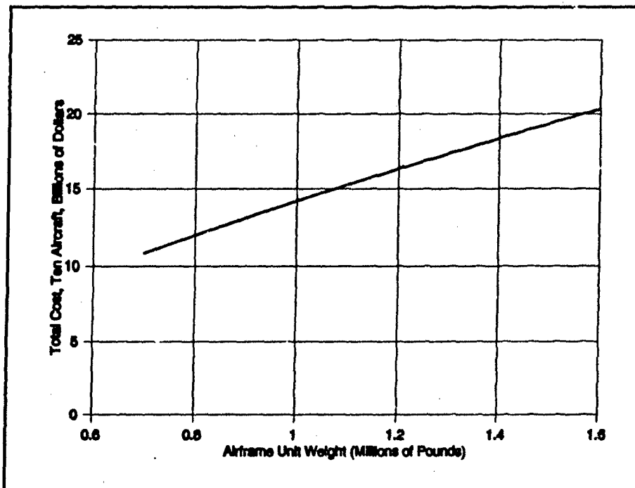
Figure 30: Wingship Cost Versus Airframe Unit Weight
