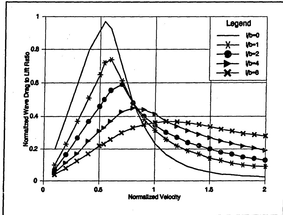
Figure 23: Water Wave Drag
