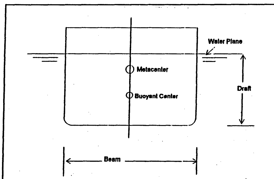
Figure 19: Stability Geometry
