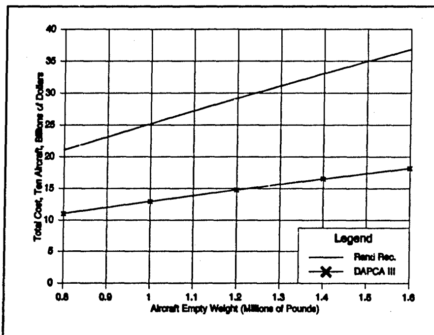
Figure 31: Wingship Cost Versus Empty Weight
