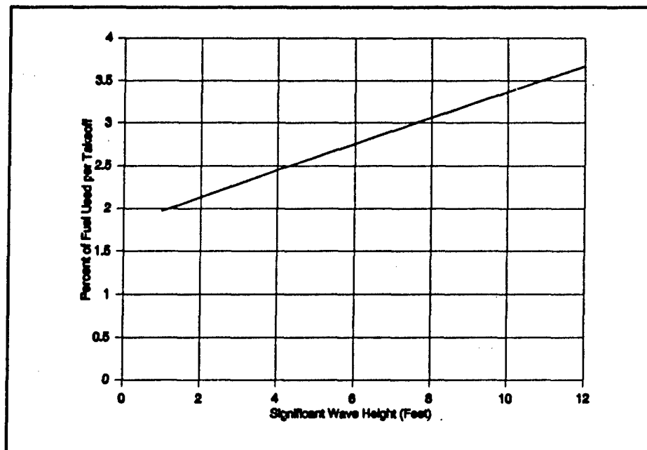
Figure 26: Takeoff Fuel Required
