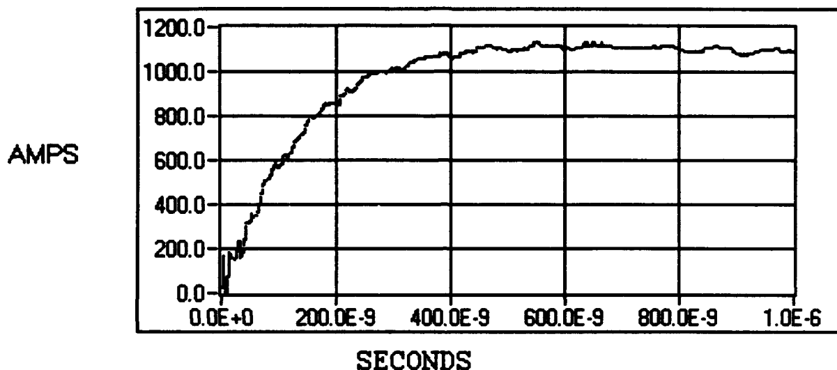
Figure 7. Marx output into 20\ \Omega 100 ns/division sweep.
