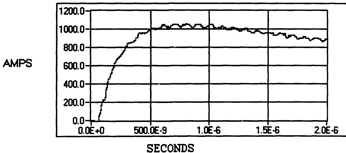
Figure 12. Parallel output into 10 \Omega 200 ns/division sweep.
