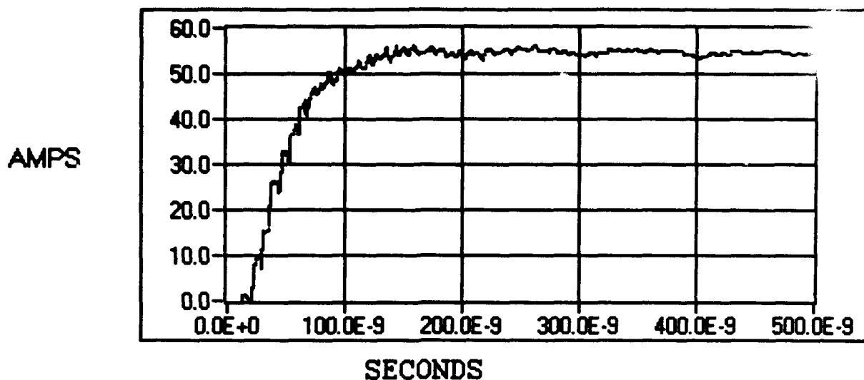
Figure 11. Parallel output into 200 \Omega 50 ns/division sweep.
