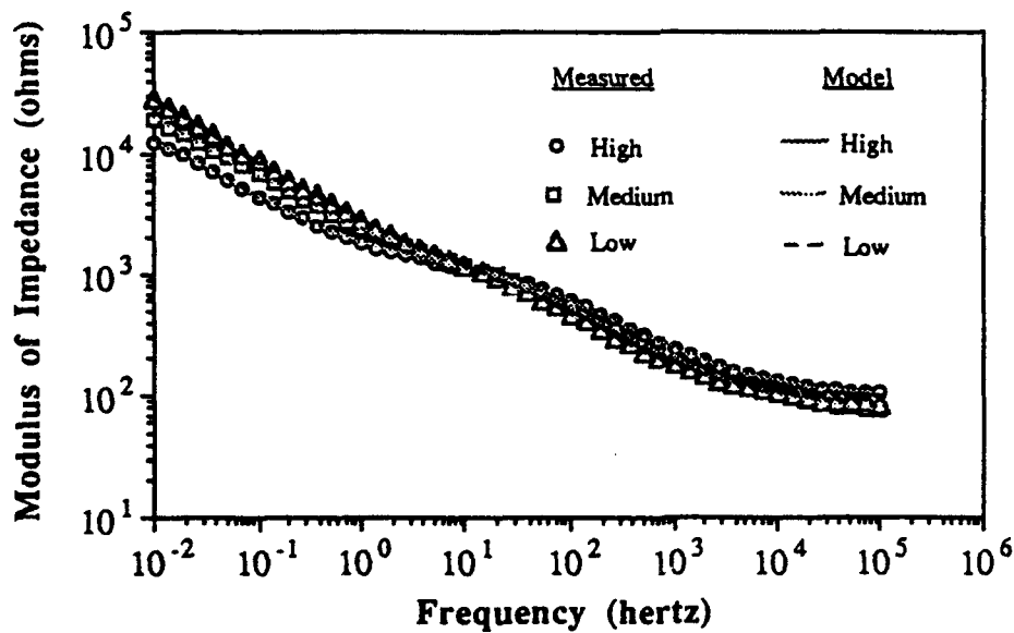
Figure 8a. Bode magnitude data and model fit for high (1atm),
