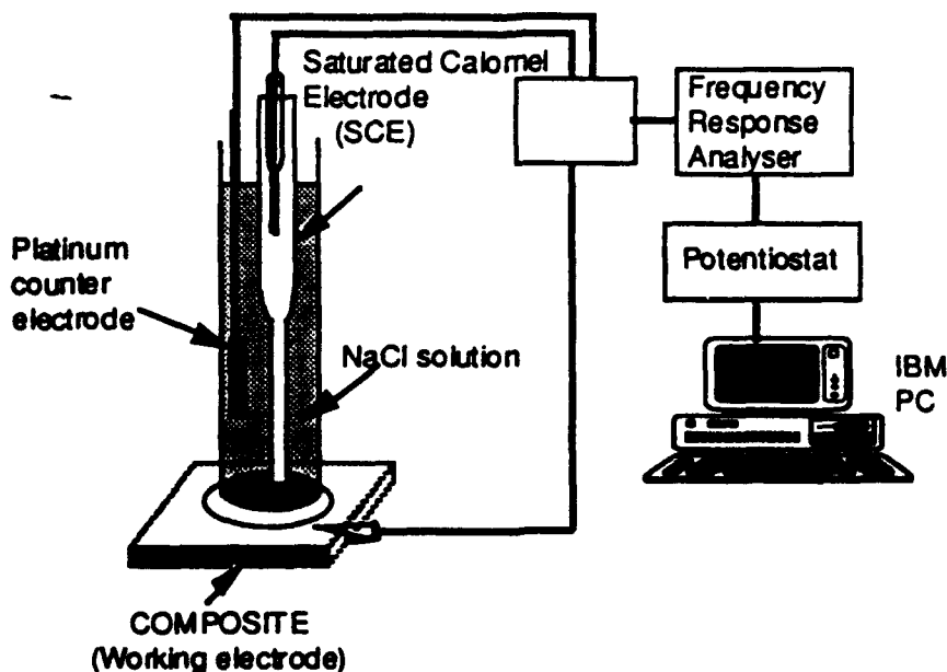
Figure 3. Experimental apparatus for electrochemical testing.
