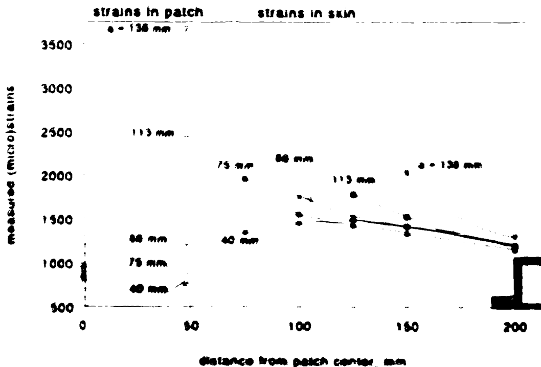
Figure 6.3 Strains in the skin and patch in the central portion of the fairing line of panel #2, various crack lengths. Skin strains are indicated by filled markers, while patch strain markers are unfilled.
