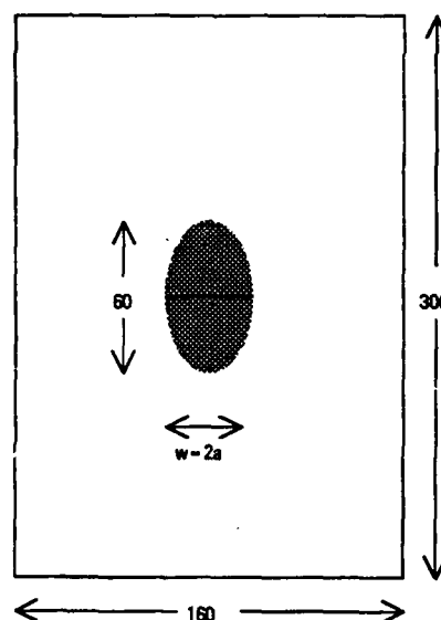
Figure 6.1. Two-sided patch specimen.
