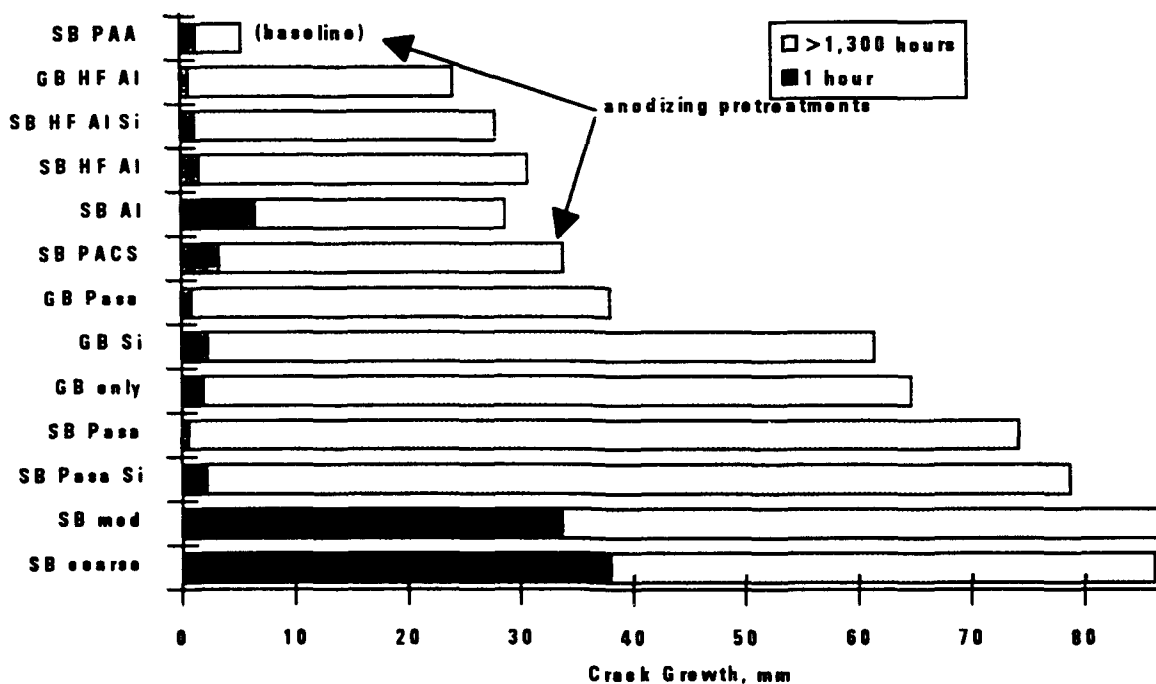
Figure 4.11 Wedge edge test results, 35°C, 99% relative humidity salt spray, no primer. Codes after Table 4.2.
