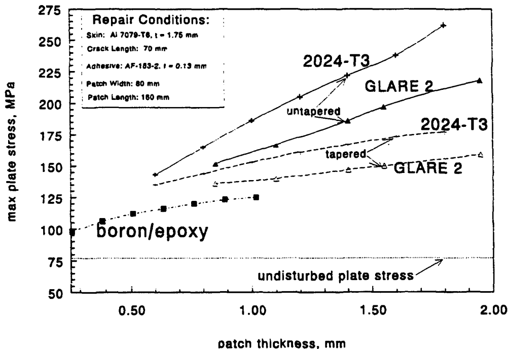
Figure 5.18. Effect of thickness tapering on combined (load attraction plus bending plus thermal) stresses in the plate just outside the patch edge for tapered bonded one-sided patches.
