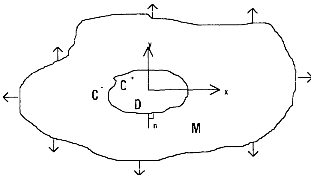
Figure A.4. Inclusion analogy model of patched uncracked plate.
