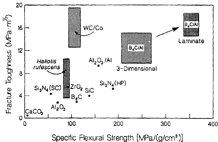
FIGURE 3-1 Fracture toughness versus specific flexural strength for abalone ( Haliotis rufescens ) shell nacre compared with monolithic ceramics and composites. Source: Sarikaya and Aksay, 1992.
