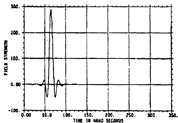
Figure 1. The Time Domain Excitation Pulse
