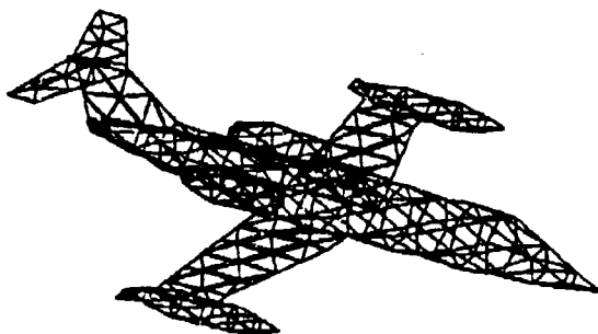
Figure 1. Typical Target of Interest for RCS Calculations
