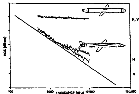
Figure 11. Frequency Dependence of an Aspect Angle Averaged RCS for Cruise Missile Models 9 ( \Delta\theta , 0^\circ - 60^\circ )
