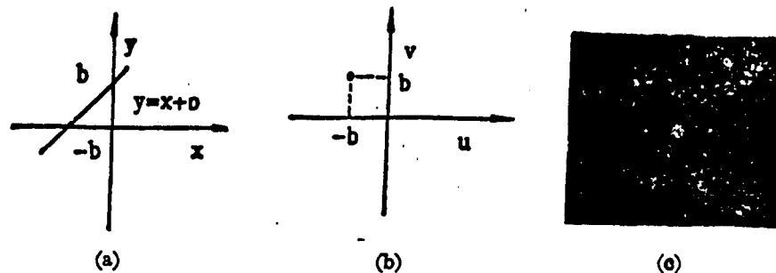
Fig. 4 Line-to-point transformation.
