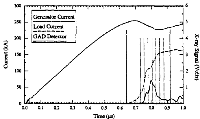
Figure 4-13. The generator current, load current, and signal obtained on a GAD detector for a POS shot at 45 kV and a 25 \mu\text{m} aluminum wire. The diode filter was a 0.5 \mu\text{m} Parylene foil coated with 800 \text{\AA} of aluminum. The dotted vertical lines indicate the timings of the x-ray framing camera and the solid vertical lines indicate the duration of the streaked absorptiongram.
