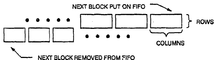
Figure 8. Input port two-dimensional FIFO.
