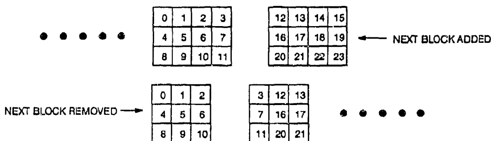
Figure 9. Memory addresses in two-dimensional FIFO.
