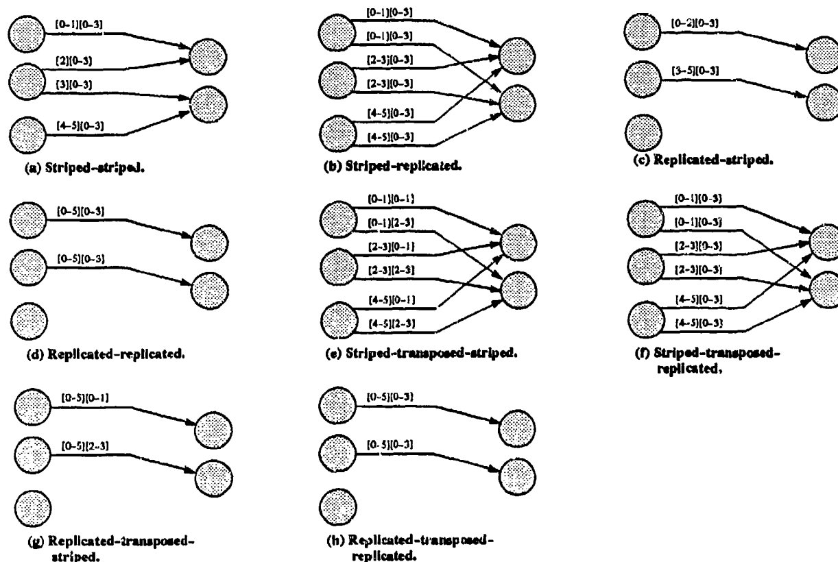
Figure 7. Internal message paths for communicating a 6 \times 4 (6 row by 4 column) array.
