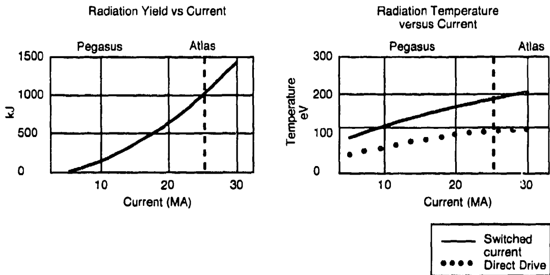
Figure 9-4. Atlas will be used as a radiation source.
