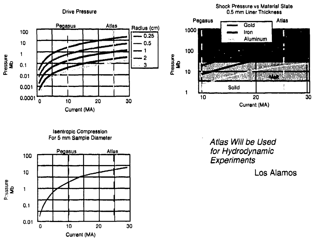
Figure 9-3. Atlas will be used for hydronamic experiments.
