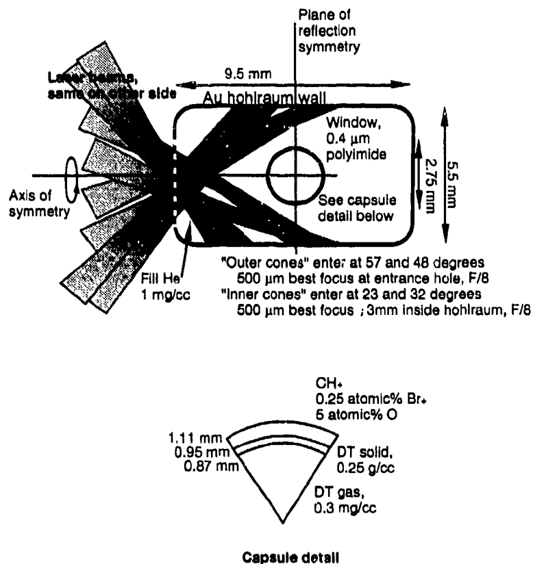
Figure 7-2. This is the point design ignition target for the NIF. The cryogenic capsule is suspended in the gold hohlraum, which is heated by the laser pulse. This design is somewhat smaller than an optimized 1.8 MJ, 4500 TW design, in order to allow margin for uncertainties in the target physics. (From LLNL)
