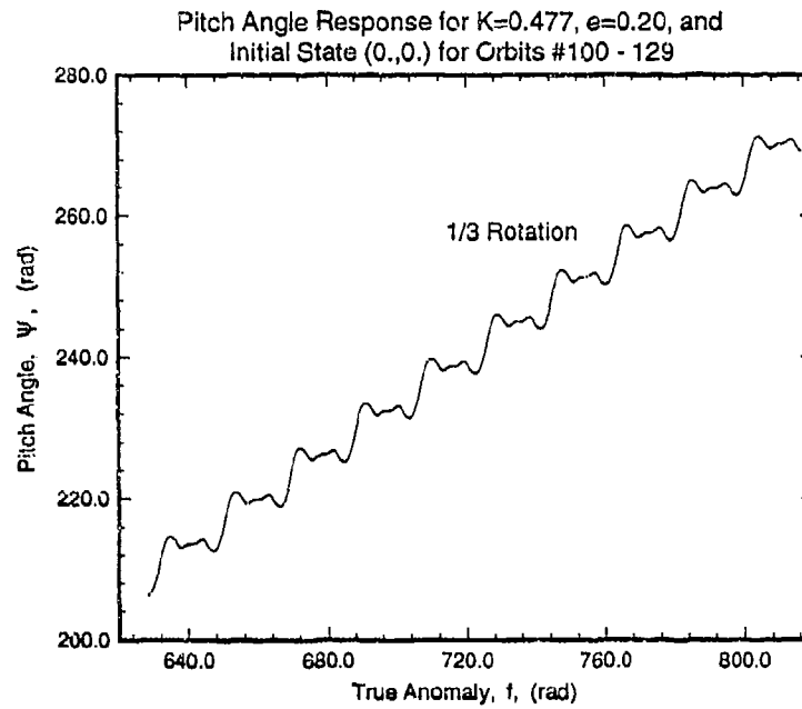
Figure 5.7: Pitch Angle Response for a P = 1/3 Rotational Trajectory: K = 0.477 , e = 0.20 , (0., 0.) for Orbits #100-129.
