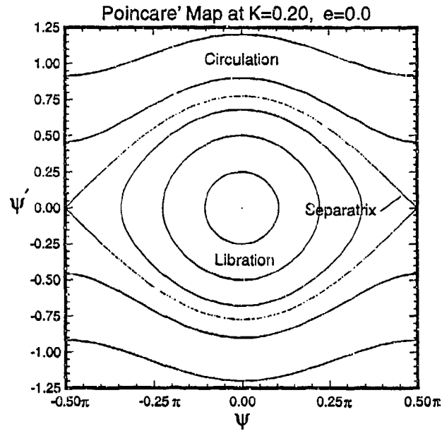
Figure 5.22: Poincaré Map for K = 0.2 and e = 0.0 .
