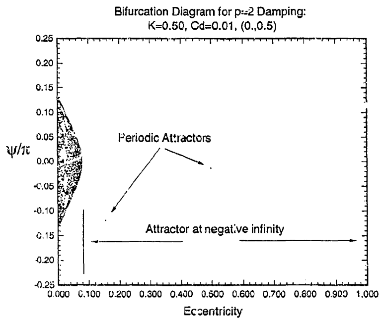
Figure 7.15: Bifurcation Diagram for Nonlinear ( p=2 ) Damping: K = 0.50 , C_D = 0.01 , and (0., 0.50) .
