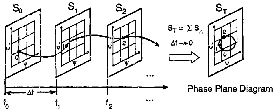
Figure 3.1: Constructing a Phase Plane Diagram from the Solution Space (\psi, \psi', f) .
