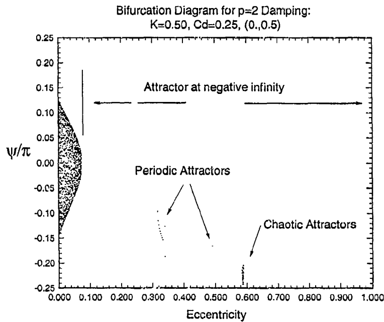
Figure 7.17: Bifurcation Diagram for Nonlinear ( p=2 ) Damping: K = 0.5 , C_D = 0.25 , and (0, 0.5) .
