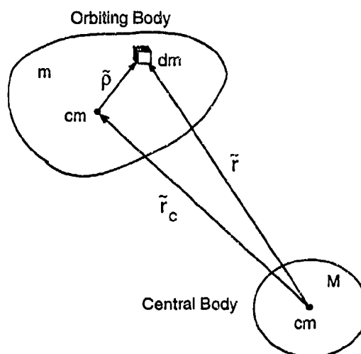
Figure 6.2: Definition of \vec{\rho} .
