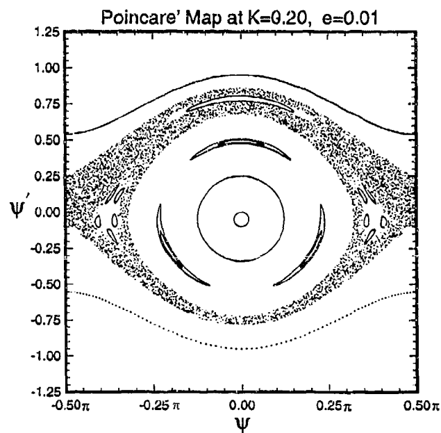
Figure 5.23: Poincaré Map for K = 0.2 and e = .01 .
