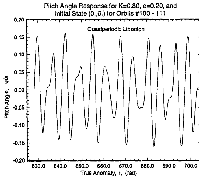
Figure 5.10: Pitch Angle Response for a Quasiperiodic Librational Trajectory: K = 0.80 , e = 0.20 , (0.,0.) for Orbits #100-111.
