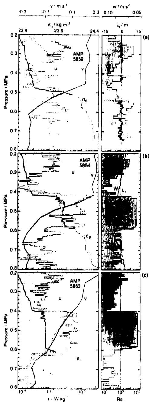
Fig. 4. AMP profiles just upstream of the billows (a, AMP 5852), through the first large billows (b, AMP 5854), and 6 buoyancy periods later (c, AMP 5863). The flow is initially two-layered (a) but develops a 20 m thick unstable and highly dissipative layer where the echosounder reveals billows. This eventually becomes well-mixed (c).
