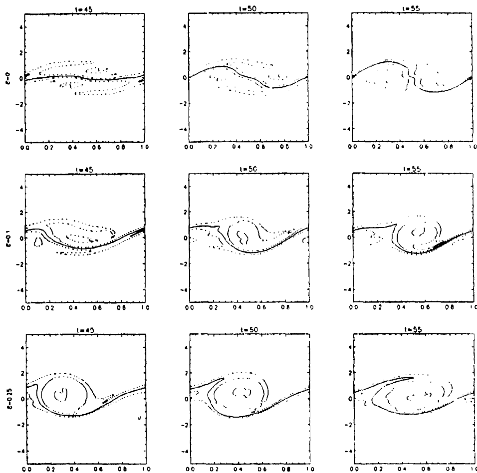
Figure 5: Results of nonlinear simulations with J = 0.12 , R = 6 , Re = 25 , and Pr = 36 for \epsilon = 0, 0.1 and 0.25 . Here contours are of constant density \rho = \rho_a(z) + \rho' in the x - z plane where x has been scaled with respect to its period 2\pi/\alpha^* .
