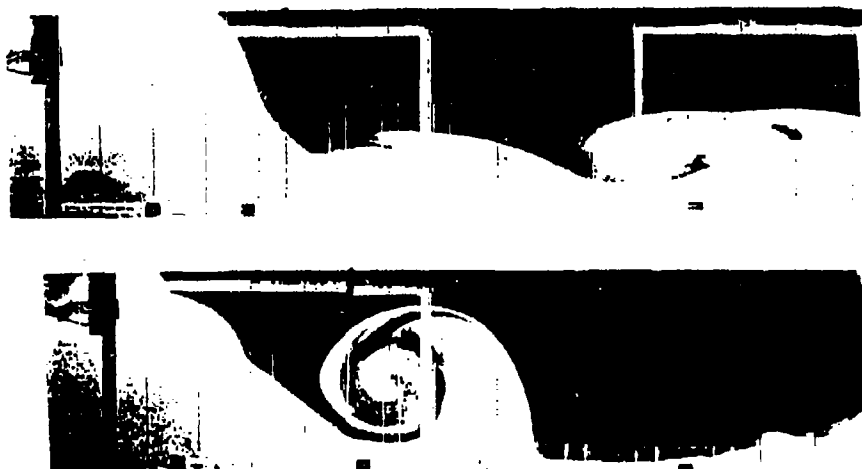
Figure 4 Typical flows in Case I runs for (i, top) \Omega = 0.13 rad s^{-1} (ii, bottom) \Omega = 0.26 rad s^{-1} . Note that the intrusions here originate on the along-channel front of the boundary current (c.f. Figure 1).
