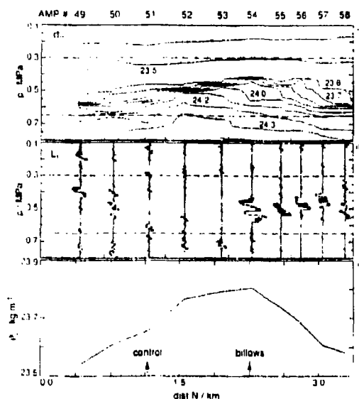
Fig. 5. a) Contours of \sigma_\rho derived from the AMP profile (aliased for scales \leq 300 m); b) Profiles of displacement, L_t ; and c) average density between 0.3 and 0.65 MPa. The pycnocline rises steeply after the control and before billows, then thickens and falls after billows form.
