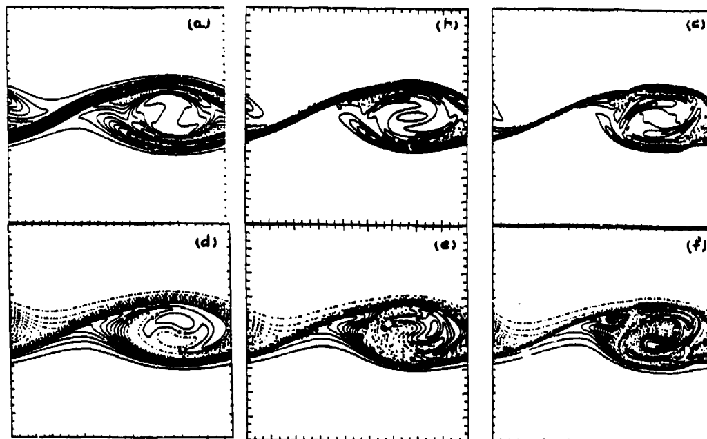
Figure 1: Influence of the initial Reynolds number Re upon the structure of the flow at the time the vorticity reaches an absolute maximum \Omega_{max} (located at the stagnation point of the vorticity layer). d is the distance between contour levels. Contours of constant vorticity. (a) Re=400 , \Omega_{max}=2.3 , d=0.1 ; (b) Re=1000 , \Omega_{max}=3.6 , d=0.3 ; (c) Re=2600 , \Omega_{max}=6. , d=0.5 . Associated contours of constant density: (d) to (f), with d=0.1 .
