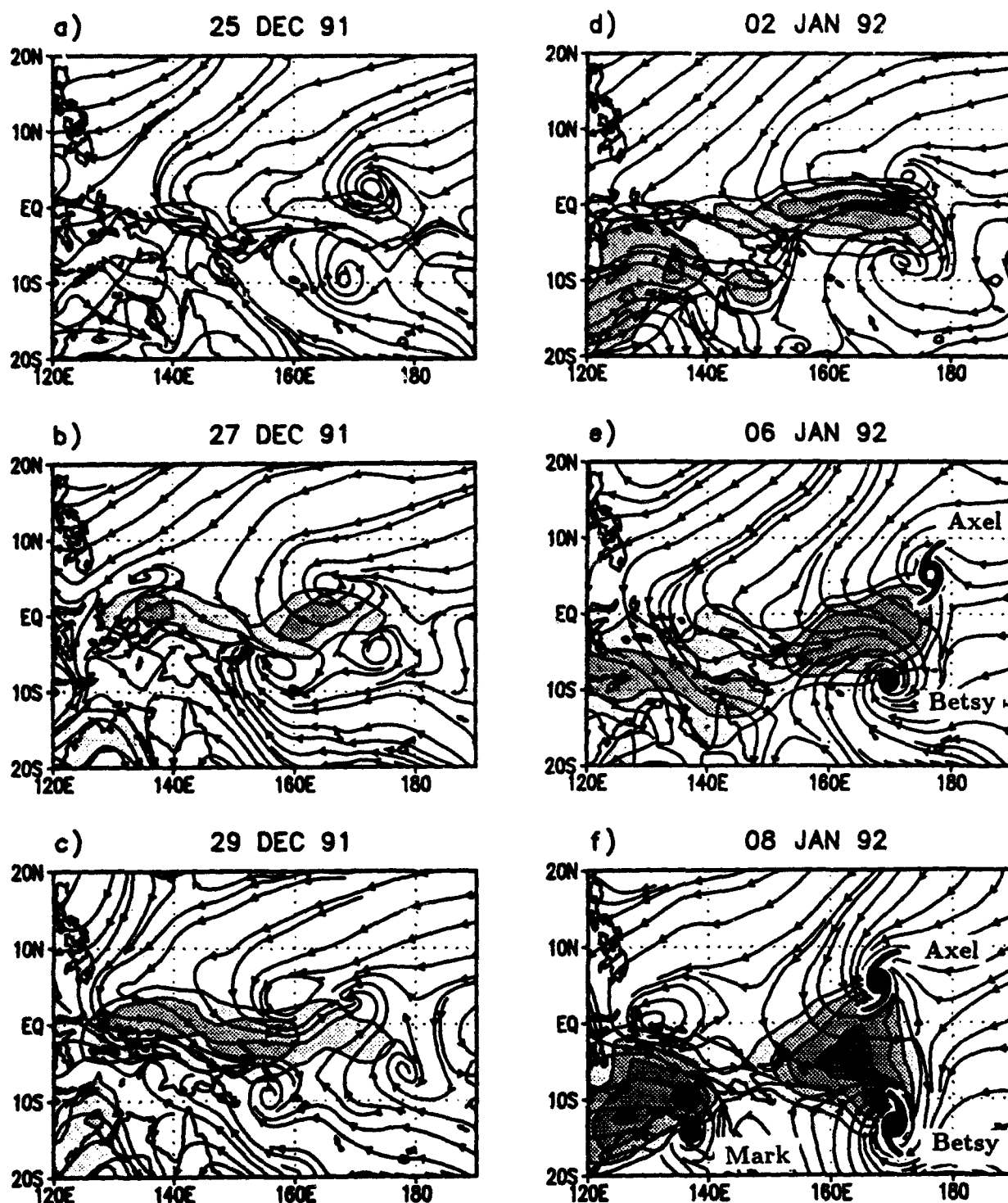
Fig. 21 - Same as Fig. 9, but for a) December 25, 1991, b) December 27, 1991, c) December 29, 1991, d) January 2, 1992, e) January 6, 1992, f) January 8, 1992
