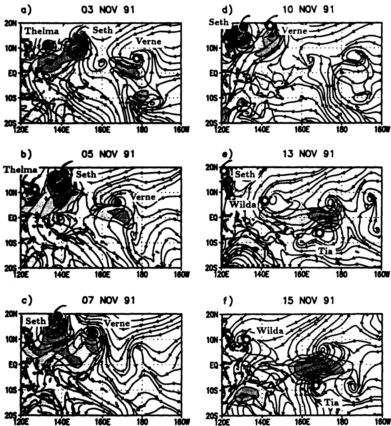
Fig. 16 - Same as Fig. 9, but for a) November 3, 1991, b) November 5, 1991, c) November 7, 1991, d) November 10, 1991, e) November 13, 1991, f) November 15, 1991
