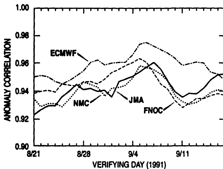
Fig. 3 - Anomaly correlations for the 48-h 500-mb height forecast in the northern mid-latitudes from four different operational centers. The values are 5-day running means comparing forecast fields to self-analyses.
