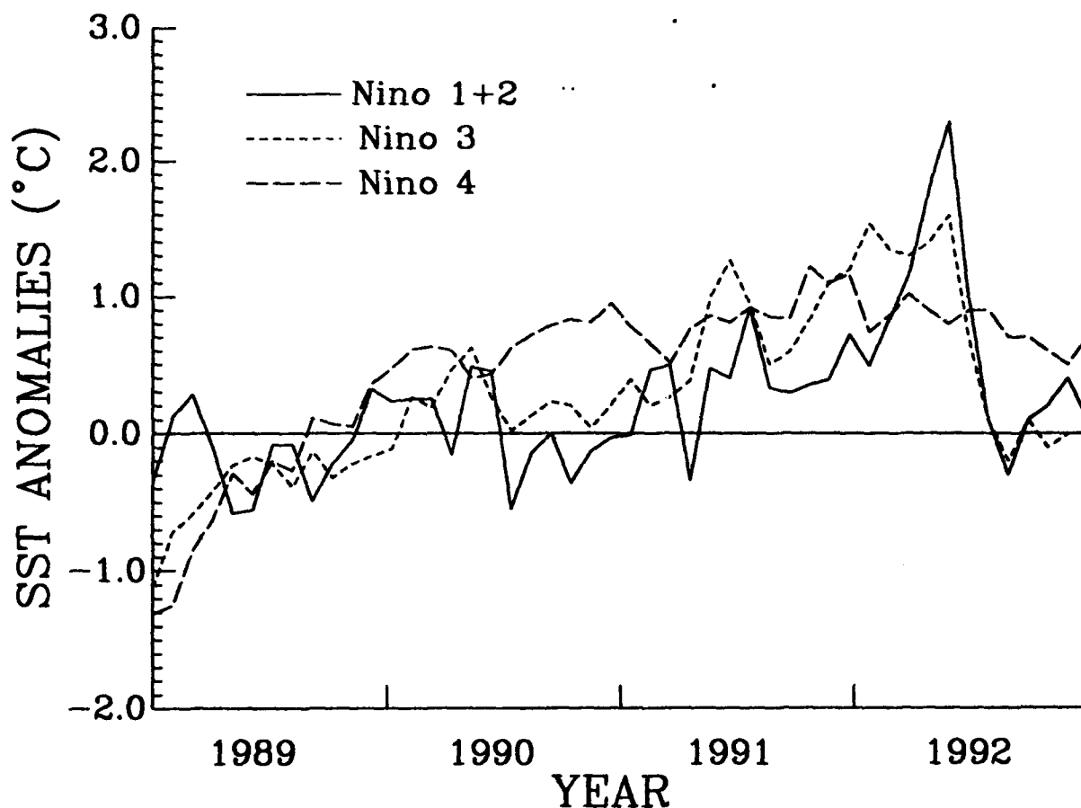
Fig. 5 - Sea-surface temperature anomalies ( ^{\circ}\text{C} ) in three El Niño areas, Nino 1+2 ( 0^{\circ} to 10^{\circ}\text{S} , 90^{\circ}\text{W} to the S. American coast), Nino 3 ( 5^{\circ}\text{S} to 5^{\circ}\text{N} , 150^{\circ}\text{W} to 90^{\circ}\text{W} ), and Nino 4 ( 5^{\circ}\text{S} to 5^{\circ}\text{N} , 160^{\circ}\text{E} to 150^{\circ}\text{W} )
