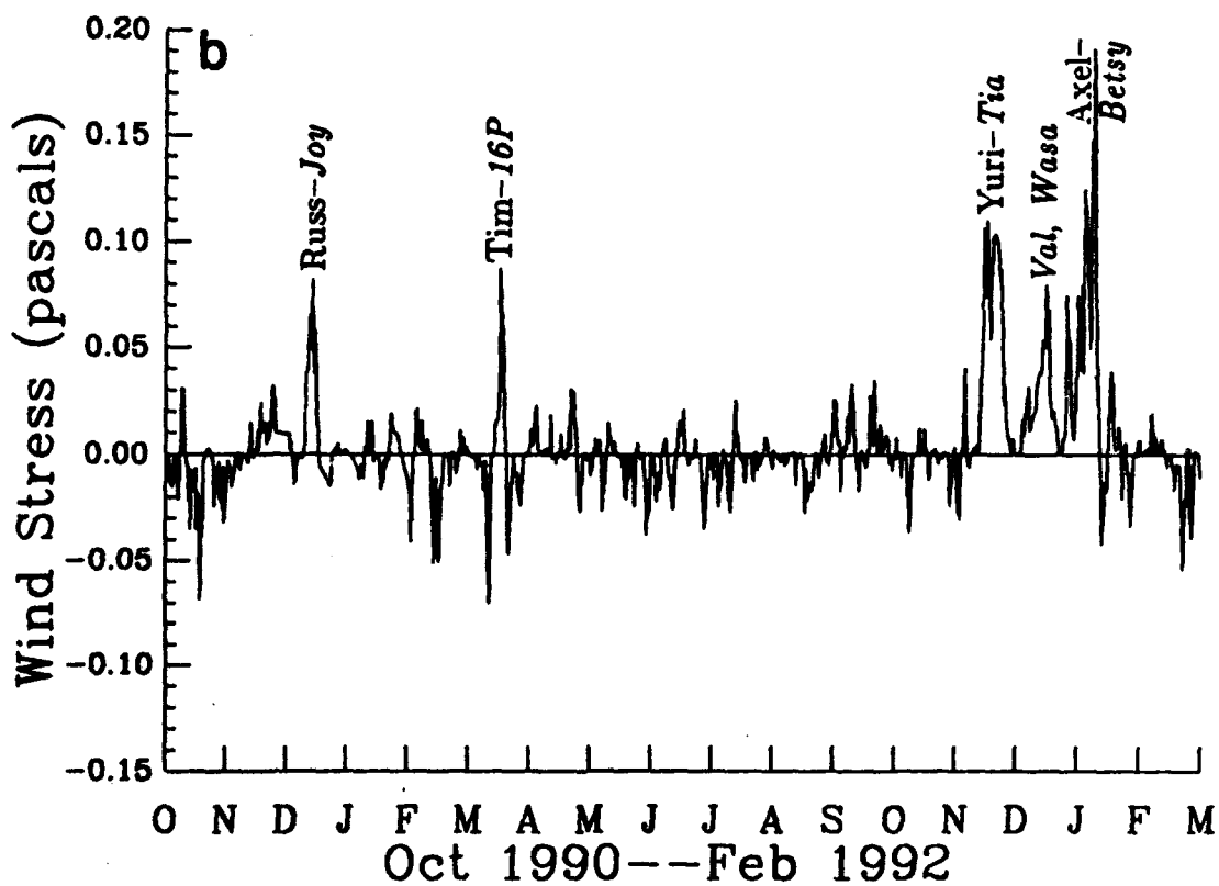
Fig. 24 - Zonal component of the NOGAPS surface wind stress (pascals) at (a) 0°N, 156°E and (b) 0°N, 165°E, with names of associated tropical cyclones noted
