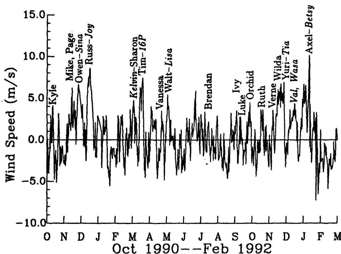
Fig. 23 – NOGAPS 10-m zonal wind component at 0^{\circ}\text{N} , 156^{\circ}\text{E} , with a three-day filter applied. Tropical cyclones associated with particular westerly wind bursts are noted, with Southern Hemisphere storms in italics and dual-hemisphere couplets hyphenated.
