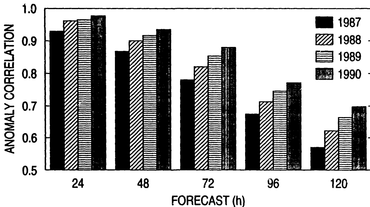
Fig. 2 - NOGAPS mean annual anomaly correlations for the northern mid-latitudes (20° N-80° N)
