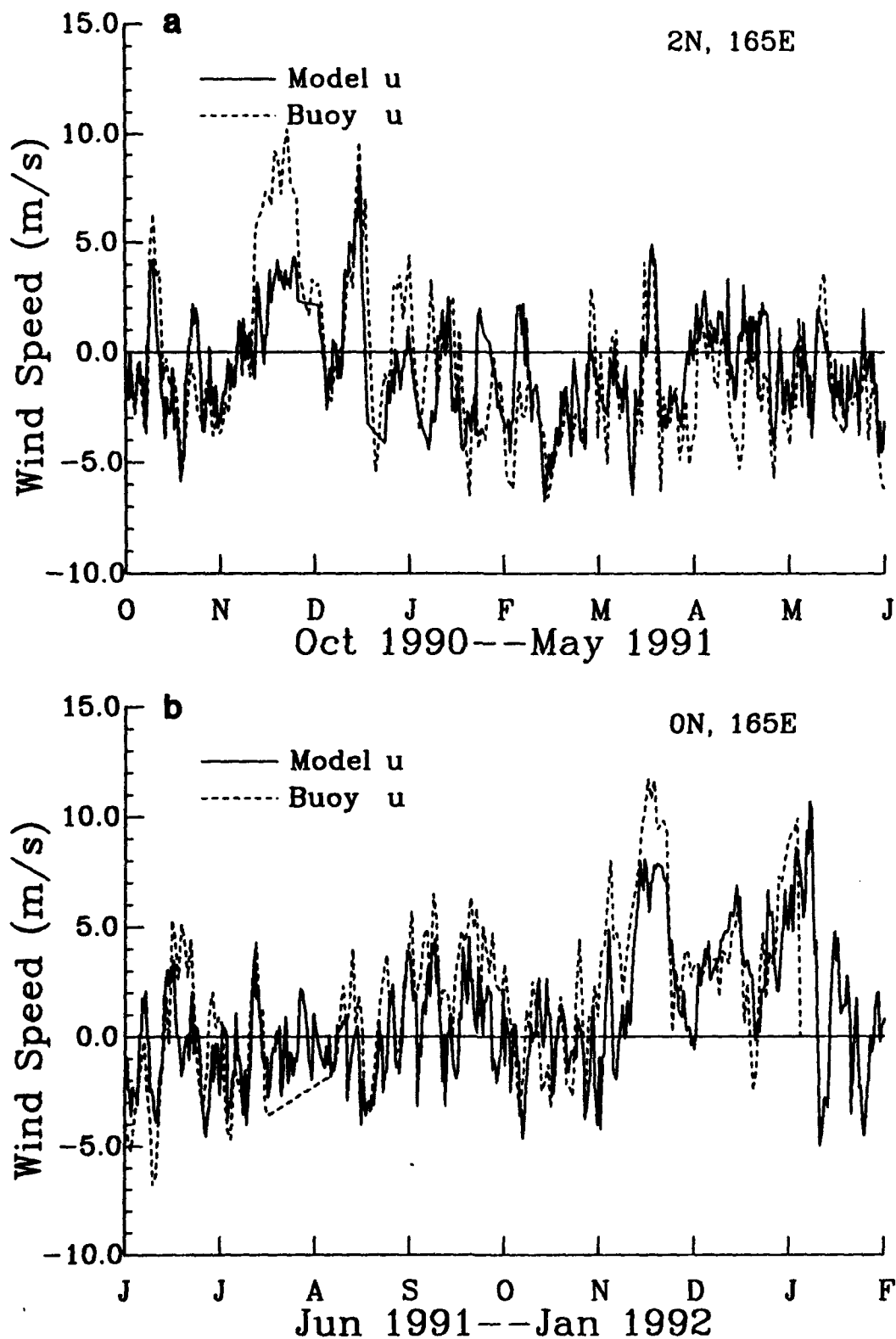
Fig. 8 - A comparison of the NOGAPS 10 m zonal wind component (m/s) to the observed zonal wind component at a) 2°N, 165°E, and b) 0°N, 165°E
