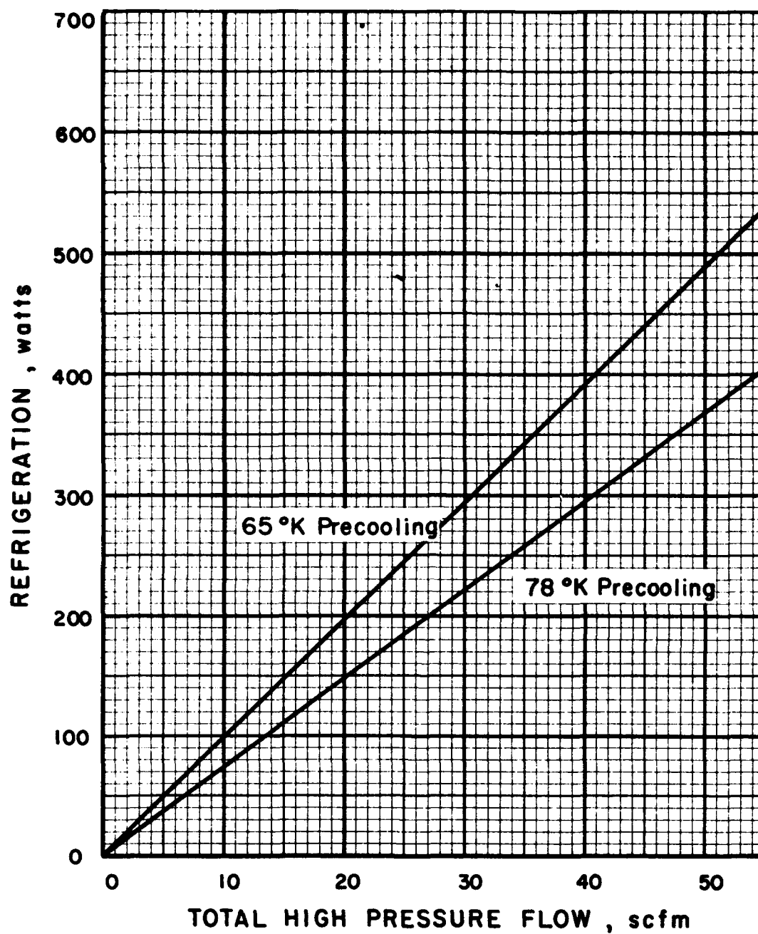
Figure 9. Theoretical Refrigeration
