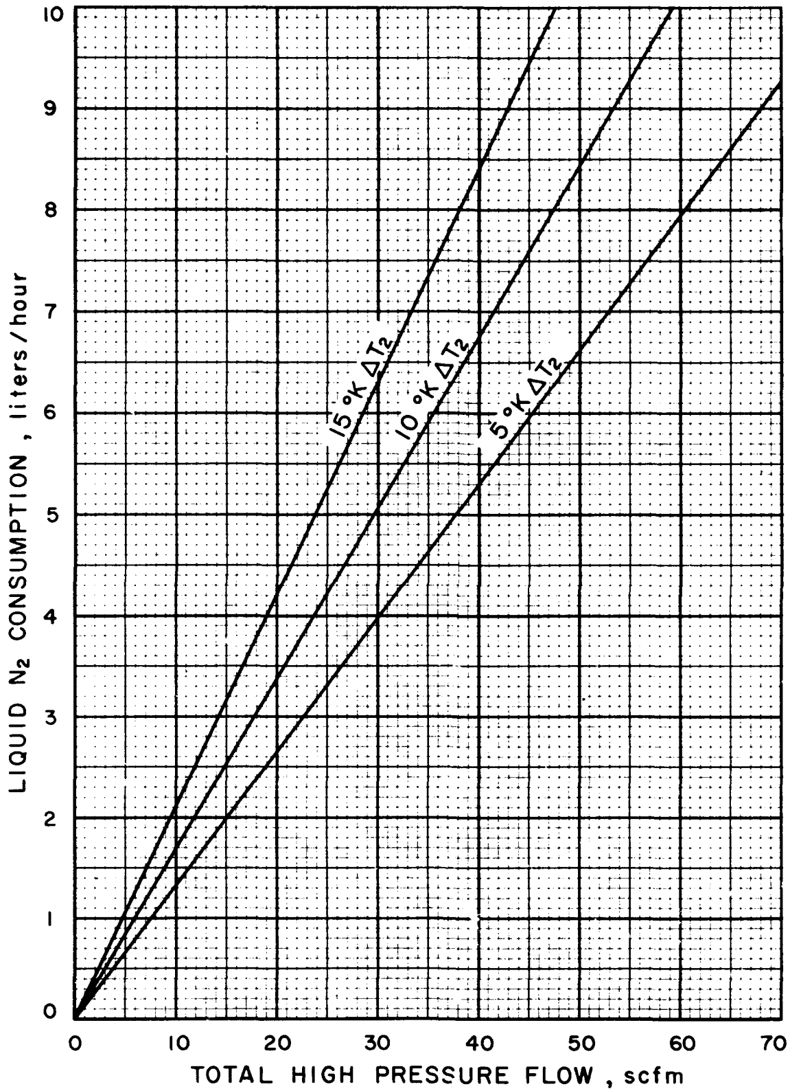
Figure 11. Liquid N 2 Consumption for 78°K Precooled Refrigerator
