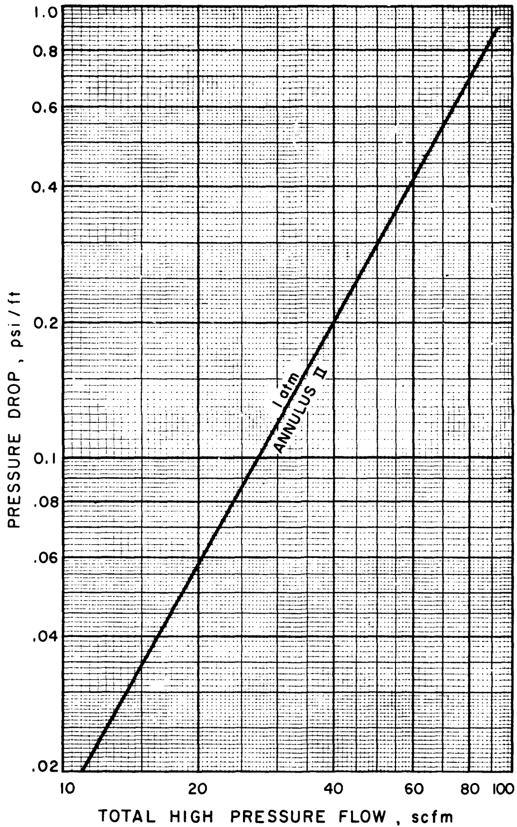
Figure 18. Final Heat Exchanger Pressure Drop
