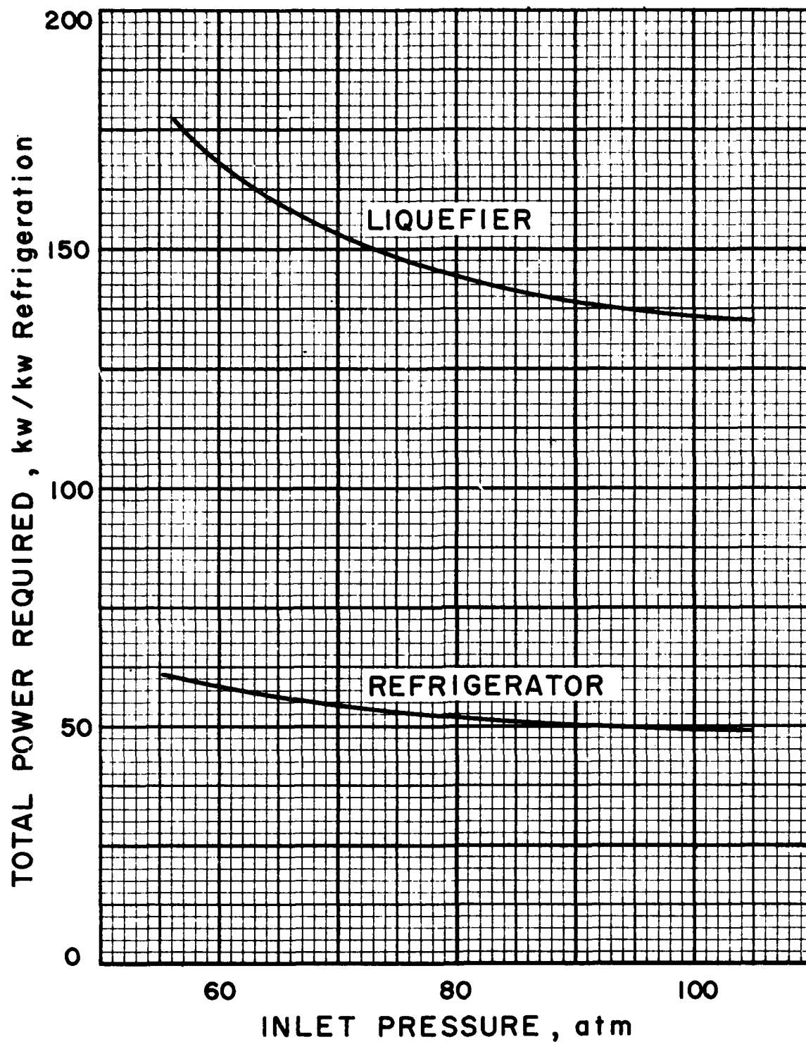
Figure 1. Power Requirements for Refrigerator and Liquefier
