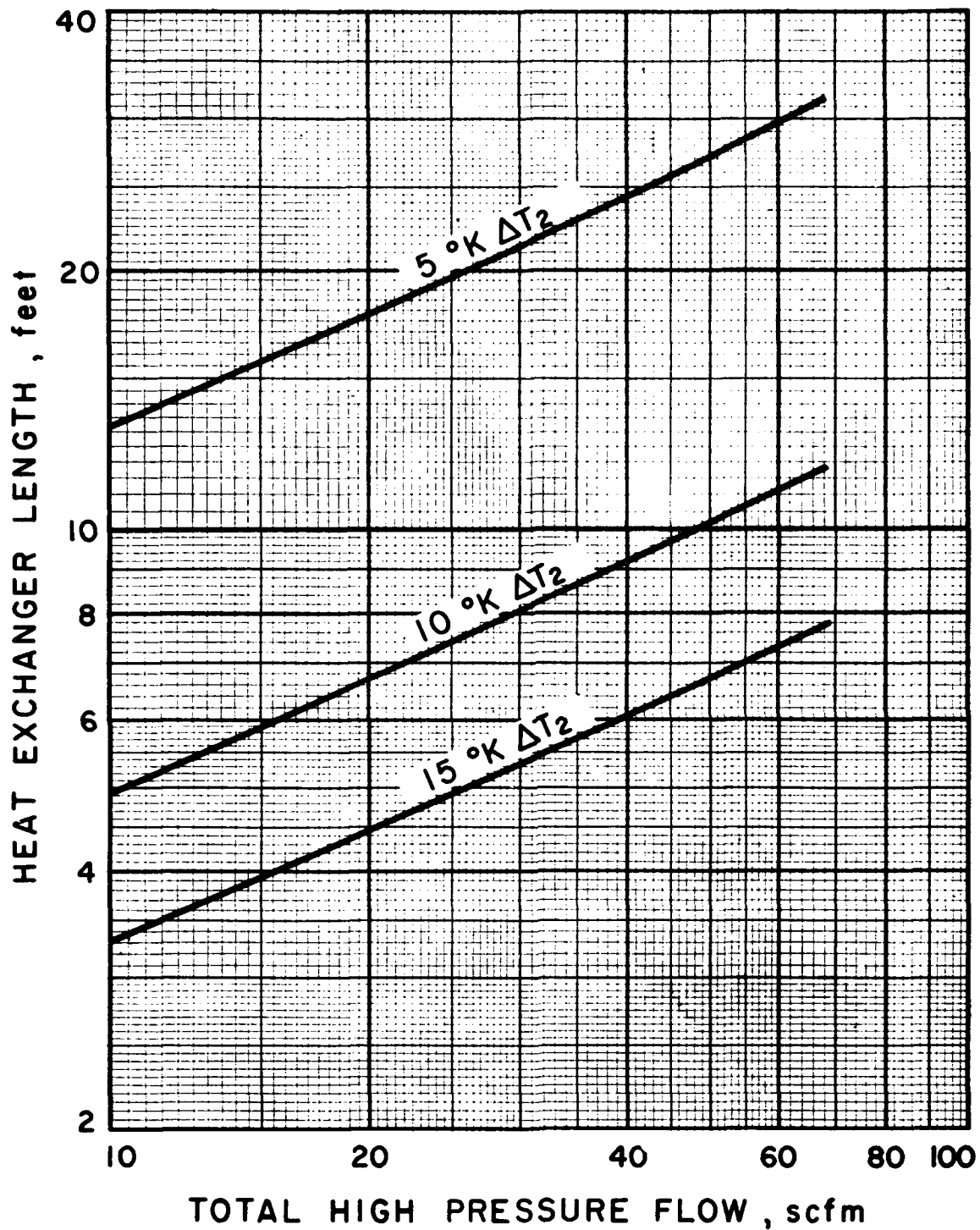
Figure 14. \text{H}_2 - \text{H}_2 - \text{N}_2 Heat Exchanger Length for 65°K Precooled Refrigerator
