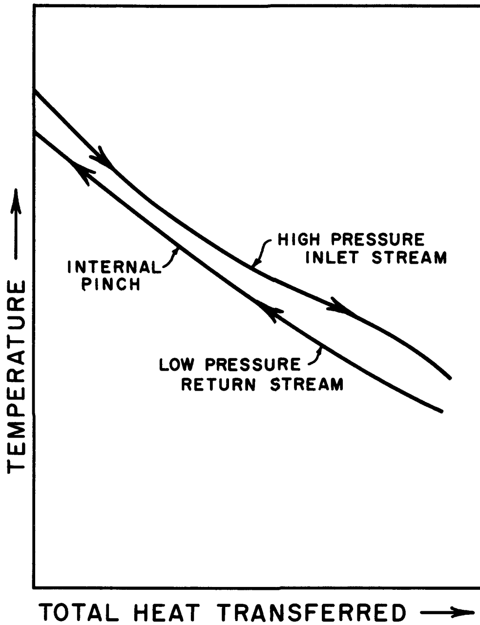
Figure 8. Typical Cooling Curve with Internal Pinch
