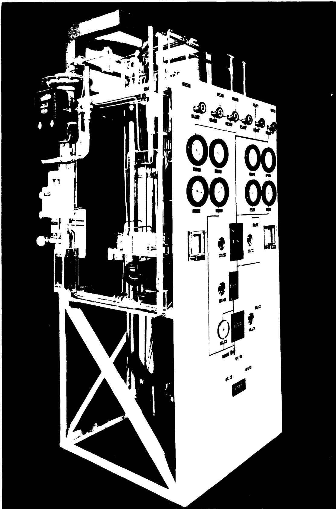
Figure 6. View of Refrigerator Panel Board
