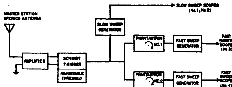
Fig. 26. Block diagram for sweeps (master station only).
