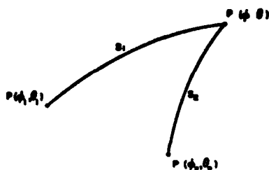
Fig. 32. Points on an oblate sphere.
