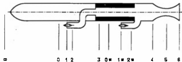
Figure 3.2: SFRJ configuration station numbers
