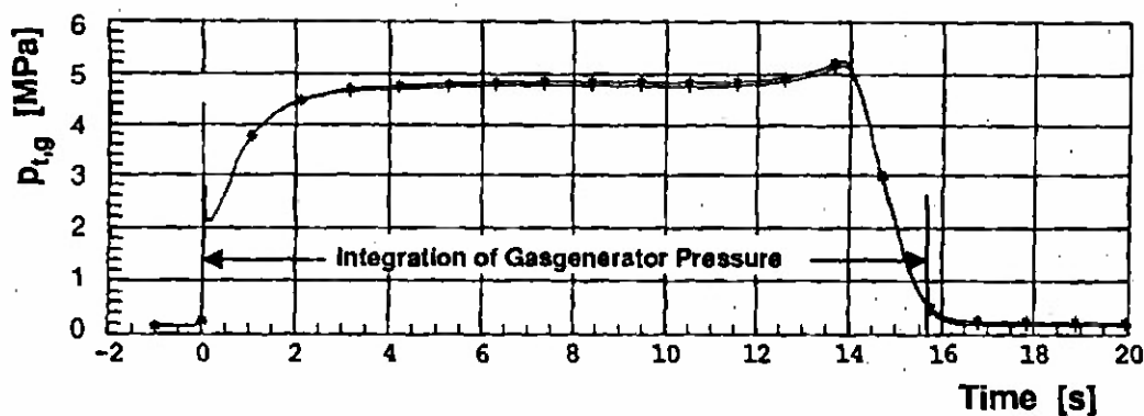
Figure 7.2: Gas generator pressure (Case 3)
