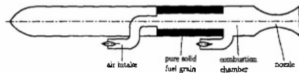
Figure 2.8: Sketch of a solid fuel ramjet
