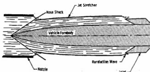
Figure 2.15: Jet stretcher concept
