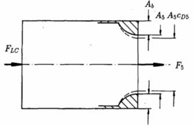
Figure C.1: Definitions for the derivation of the momentum equation
