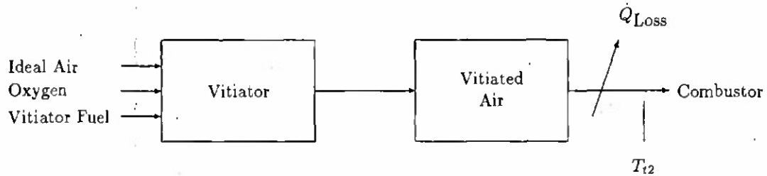
Figure 4.1: Schematic of vitiator test setup
