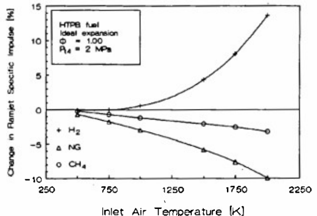
Figure 8.6: Effect of vitiator fuel on SFRJ specific impulse when comparing vitiated air with ideal hot air [34]
