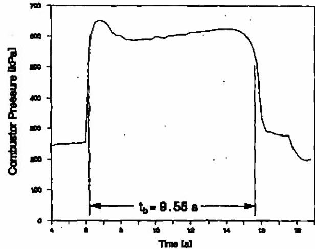
Figure 7.5: SFRJ burn time determination (Case 4)
