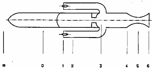
Figure 3.3: Ducted rocket configuration station numbers
