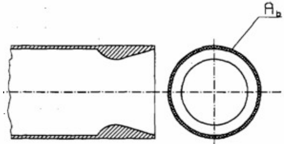
Figure 5.1: Base area for a convergent-divergent nozzle
