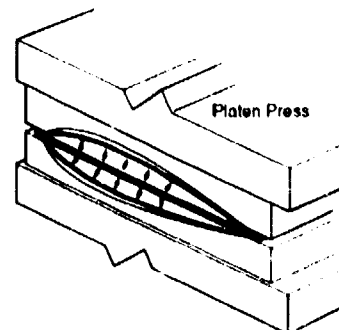
Outer skin forms first under gas pressure to limits of tool cavity
