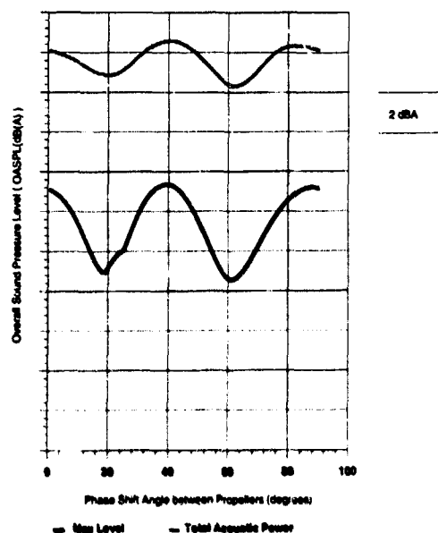
Figure 3: Variation in noise with synchrophase angle.
