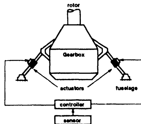
Figure 21. Functional Scheme of an Active Gearbox Strut
