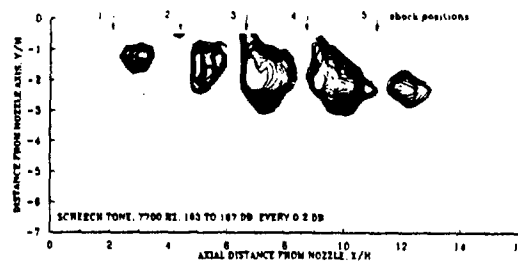
Figure 7: Acoustic sources. Numbers indicate shock cell locations.
