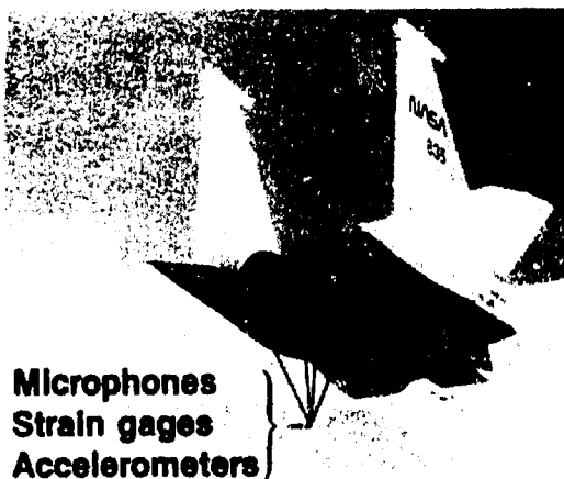
Figure 8. Ames-Dryden F-15 flight test vehicle.
