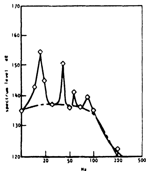
Fig 4 Full scale B-1A weapons bay acoustic levels for Mach number 0.7 at 20,000 feet
