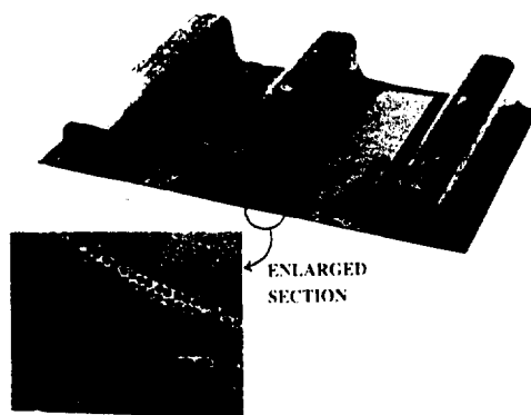
Fig. 4 Titanium metal matrix prototype wing skin panel. The silicon carbide fibers in the Ti-3V-3Cr titanium matrix are 0.006 in. (0.15 mm) in diameter.
