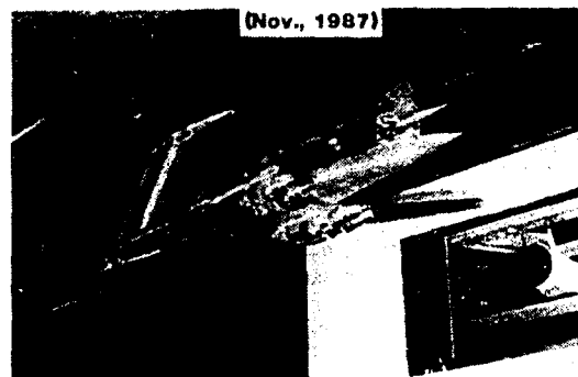
Figure 17. B-1B 6% full span model in 16 ft. tunnel.
