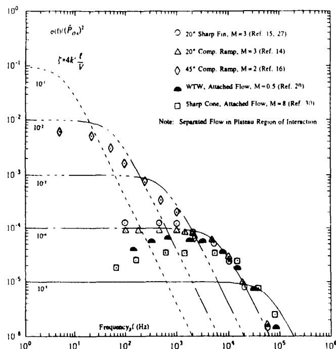
Figure 7. Normalized PSD for attached and separated flow conditions
