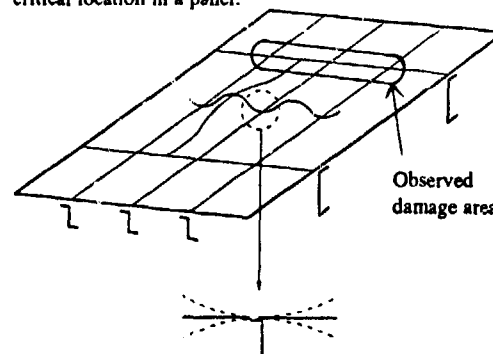
Figure 8 : Classical critical location in a stiffened panel and observed damage area for the CFRP panels.
