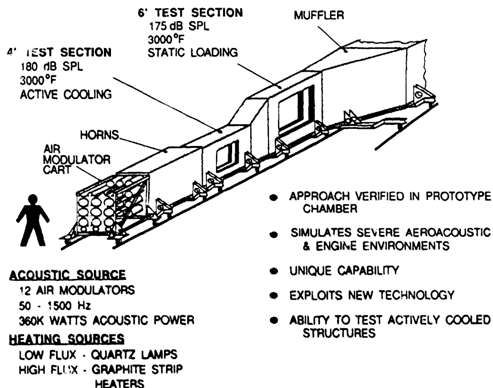
Figure 7 - Combined Environment Acoustic Chamber
