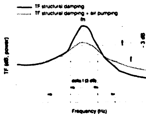
Fig. 8: Transfer function strain to input acceleration
