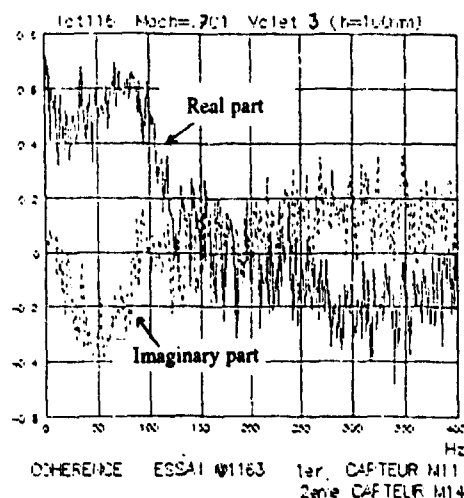
Figure 11 : Wind-Tunnel tests : Typical Correlation Factors (selected pair of microphones) vs Frequency
