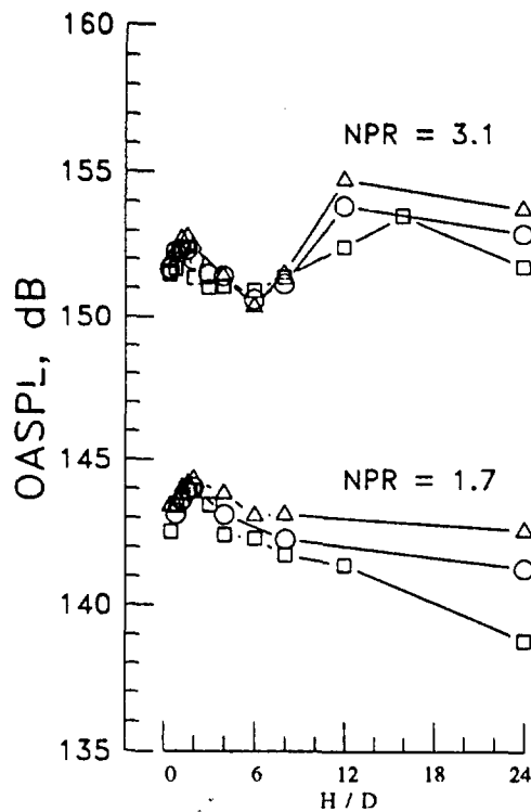
Figure 28. Dynamic pressure loads on Canard.
