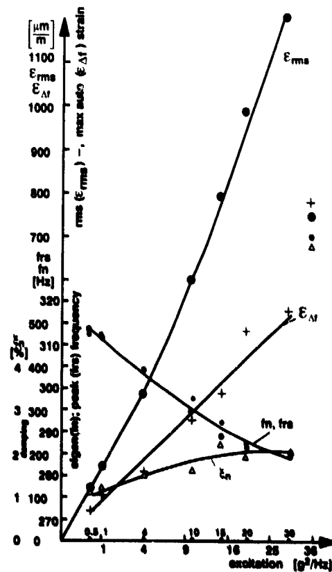
Fig. 4-3 INFLUENCE OF EXCITATION LEVEL ON TEST RESULTS (VP 4.1; skin; f_0 - f_e = 100 Hz )
