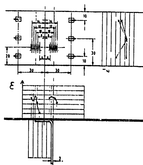
Figure 7 : Measured strain distribution for L-shaped HTA / 6376 coupon without landing
