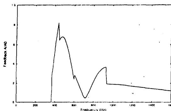
Figure 8: M_\infty = .4 , Shear layer growth rate = .05.
