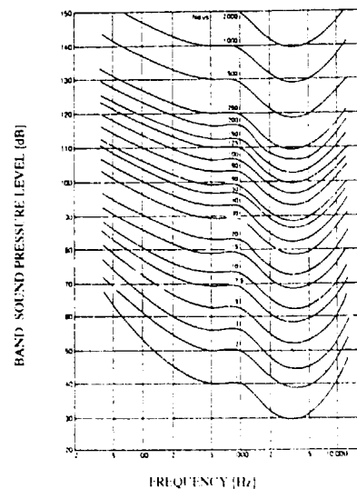
Figure 20-5 - Human response to sound loudness accounting for annoyance
