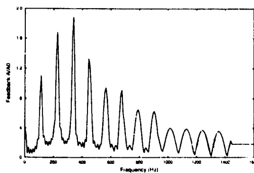
Figure 10: M_\infty = .85 , Shear layer growth rate = .05.
