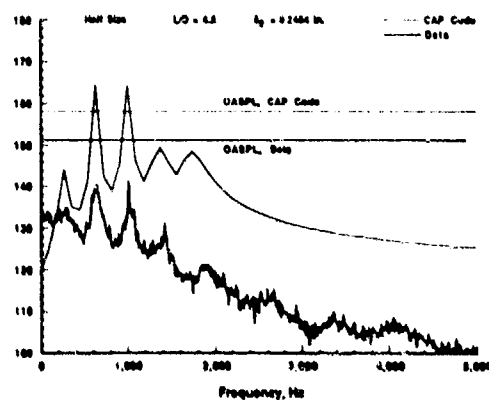
Fig 8 Comparison of cavity Acoustic Pressure (CAP) code with Mach 0.6 Data (Ref 16)
