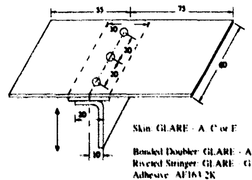
Fig. 4 Riveted-stringer specimen
