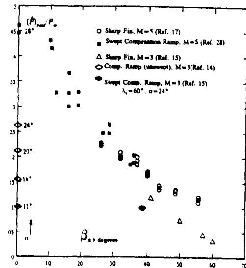
Figure 6. Normalized peak rms pressure with sweep angle for 2D and 3D interactions
