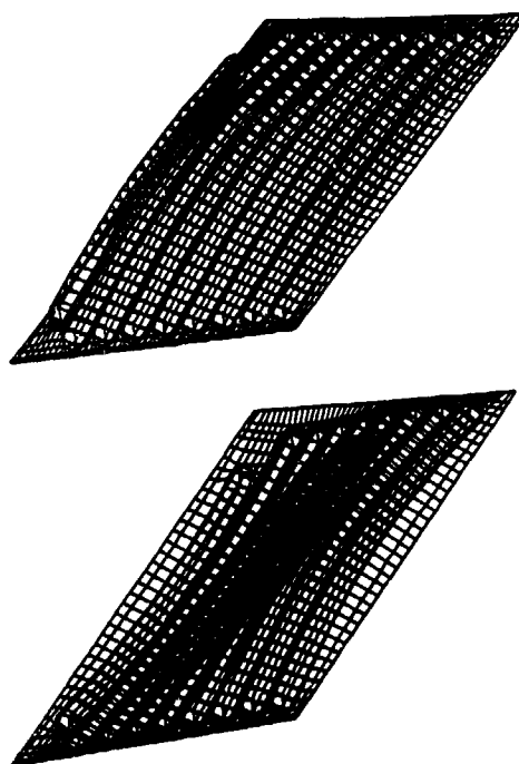
Figure 7: Keel Beam Normal Modes 1 and 2
