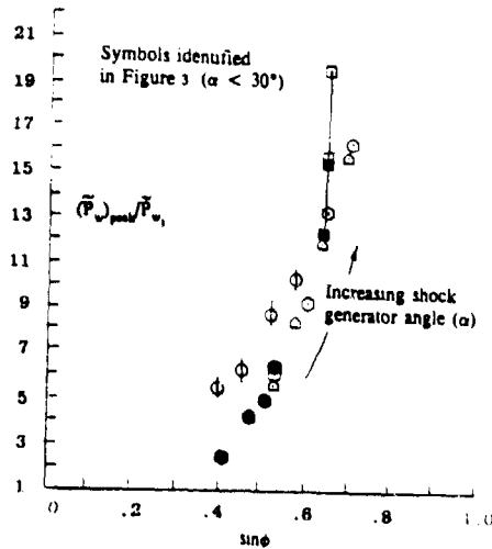
Figure 4. Correlation of peak rms pressure with modified inviscid shock angle (Ref. 1)
