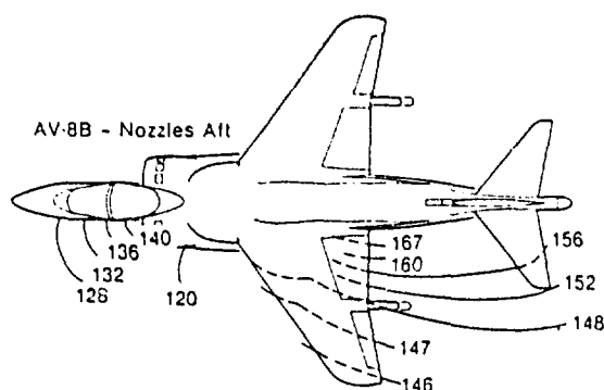
Figure 26. AV-8B cruise dynamic pressure load levels.
