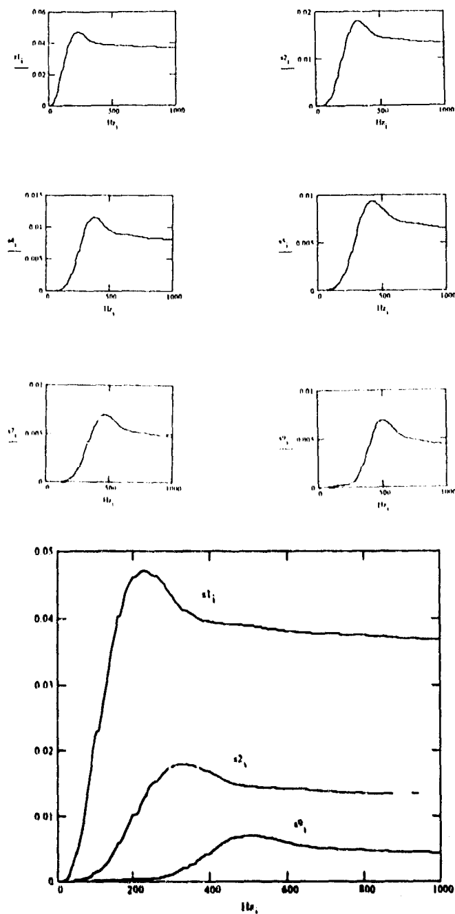
Fig.5 Non dimensional diagonal elements for the matrix C_0 .
