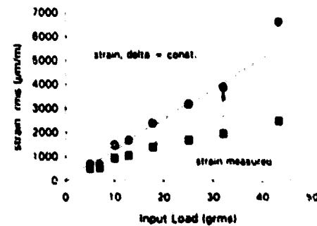
Fig. 11: Strain versus input load (over all values) at constant damping
