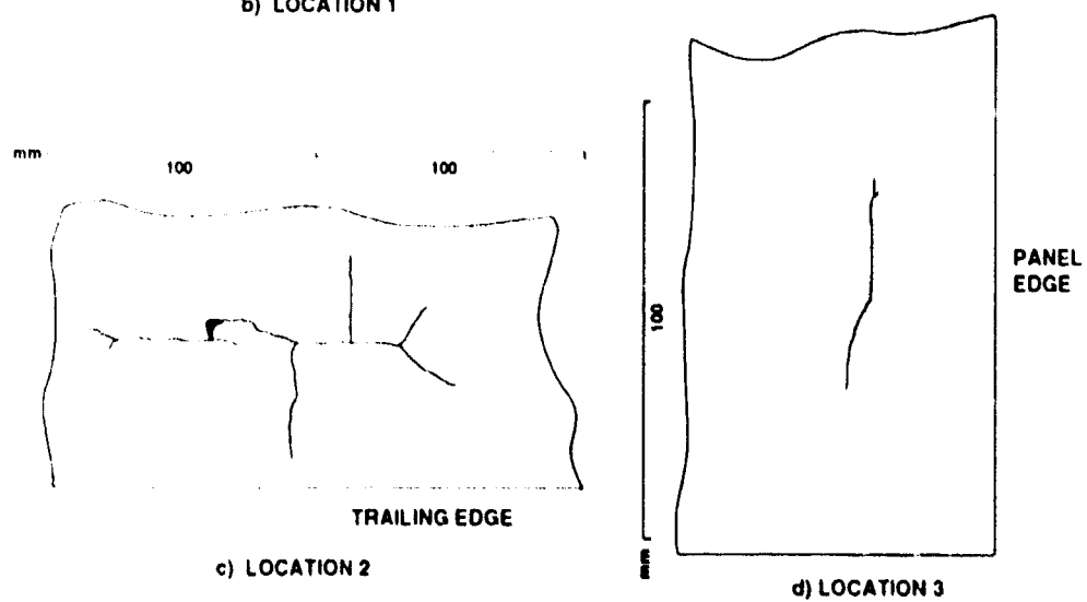
FIGURE 7 DAMAGE LOCATIONS FOR SPOILER PANEL
