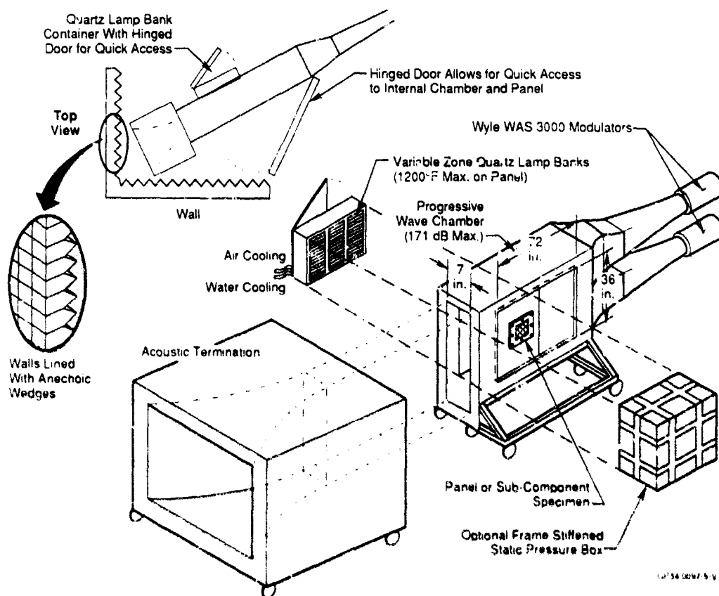
Figure 3A. Thermal/Acoustic Test Facility Facility Is Capable of 171 dB Acoustic Loading With Simultaneous Cross Flow
