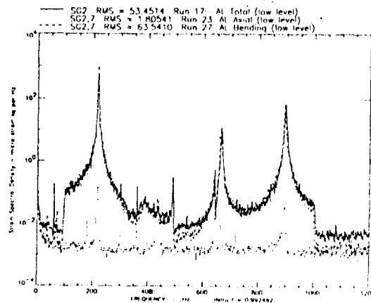
Fig 9 Strain Spectral Densities, SG 2, Total, Axial, Bending, Low Level, Random, Aluminum Plate
