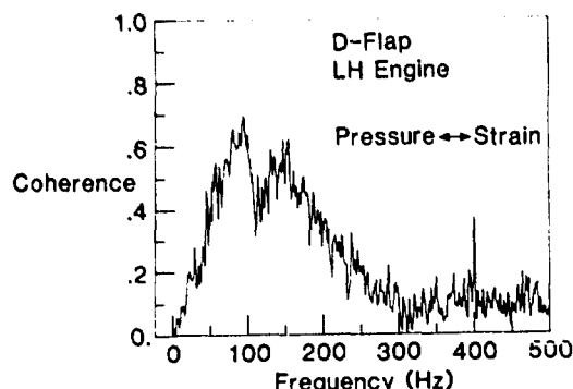
Figure 11. F-15 full scale coherence between applied dynamic load and flap strain field.
