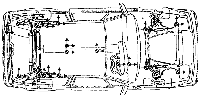
Figure 1 Structure-borne sound paths in a car
