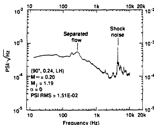
Figure 18. Characteristic spectrum showing competing mechanisms.
