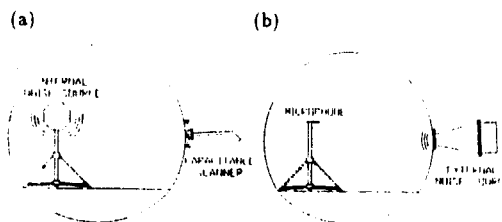
Figure 2: Schematic of reciprocal (a) and direct (b) measurement arrangement.
