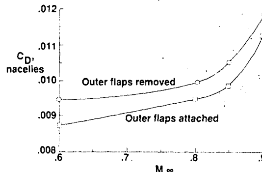
Figure 21. Performance penalty associated with removal of outer flaps on B-1B (Ref. 2).
