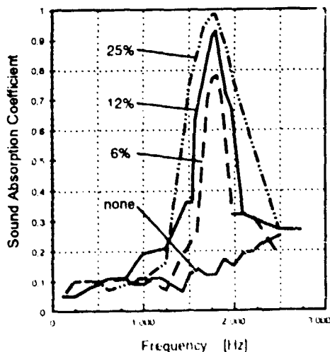
Figure 14: Absorption of the Honeycomb Plate with Different Number of Cores Converted to Resonators (6%, 12%, 25%)
