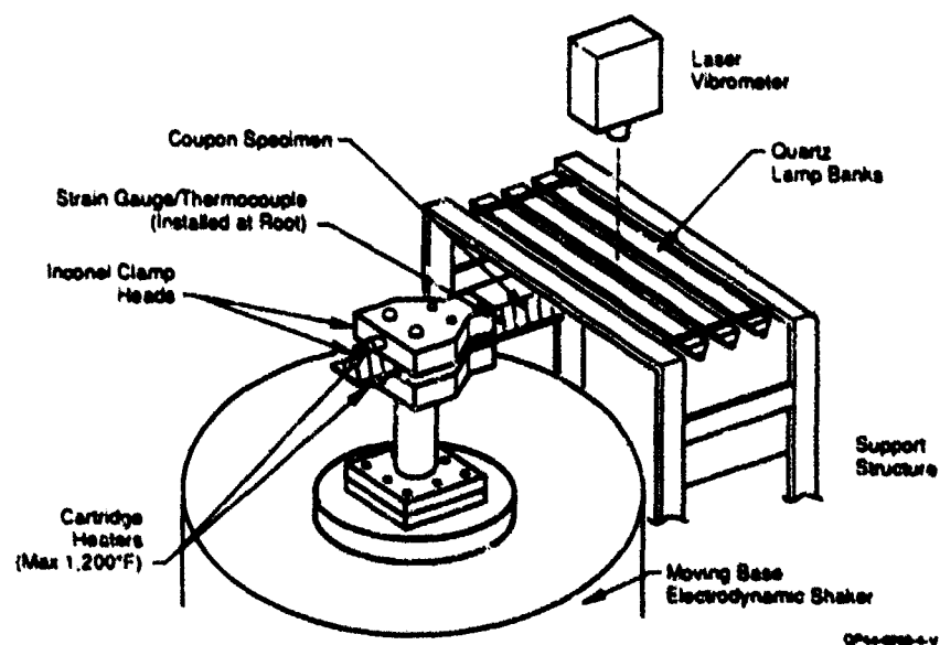
Figure 3b. General Set up of High Temperature Beam Fatigue Test Facility
