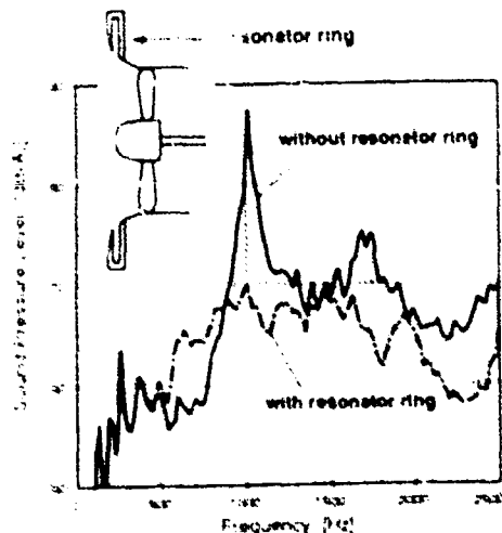
Figure 15: Noise Reduction by a Resonators Ring on an Oil-cooling Fan
