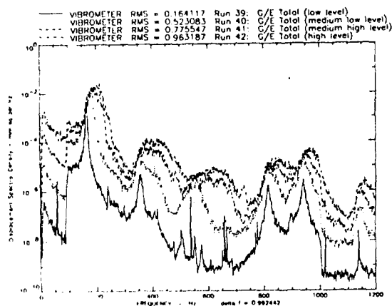
Fig 20 Displacement Spectral Densities, Random, CFRP Plate
