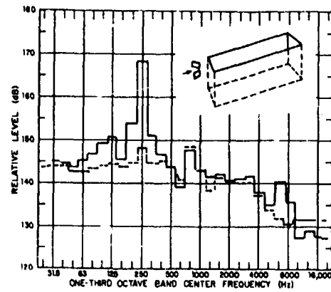
Fig 10 Example suppression of leading edge spoilers (Ref 6)
