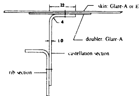
Fig. 23 Rib-castellation details in the initial design
