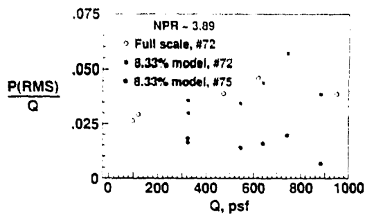
Figure 14. Model and full scale dynamic loads scaling with aircraft dynamic pressure.
