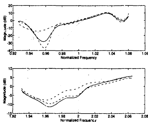
Figure 15: Normalized internal noise prediction using fewer elements. Using all information (solid), only those elements with at least 15 dB below the peak pressure on 2 cm (dashed), only elements with 10 dB (dash-dot) and only those with 7.5 dB (dotted). Data is for location 1, at 1×BPF (upper) and 2×BPF (lower).
