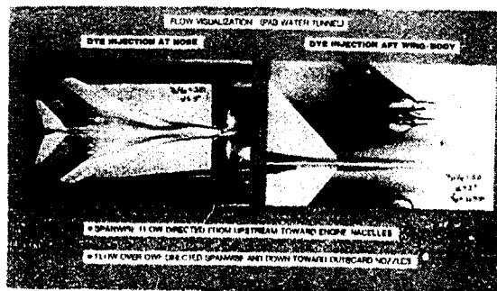
Figure 7. Flow visualization of 1/72 scale B-1B full span model with flow through inlet and exhaust.
