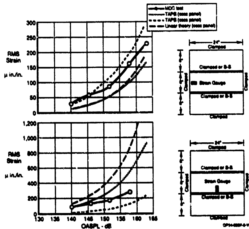
Figure 7. Strain Response Under Acoustic Excitation of Clamped 3-Bay G/E Panel
