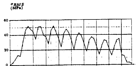
Figure 9: Theoretical stress output at clamped edge
