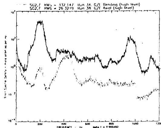
Fig 19 Strain Spectral Densities, Bending, Axial, High Level, Random, CFRP Plate
