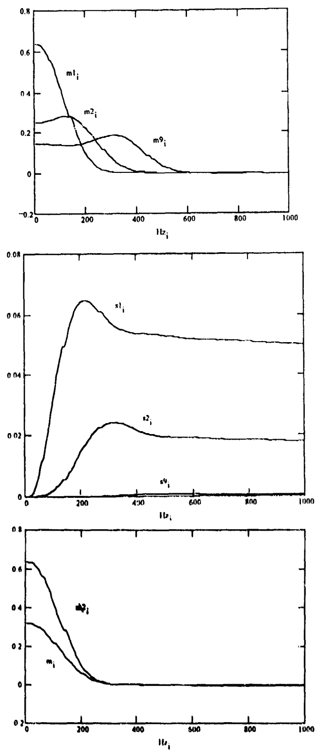
Fig. 6 Effects of weight on mass and damping
