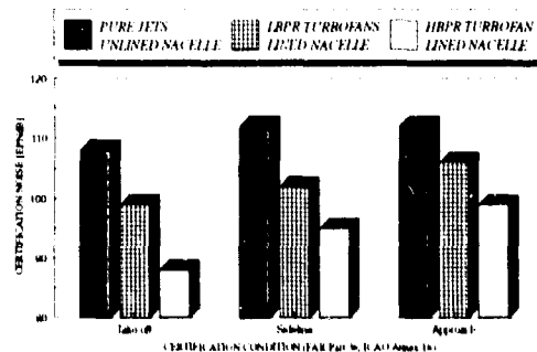
Figure 5.3 - Noise progress related to jet engine evolution and nacelle improvement
