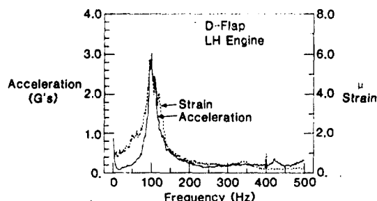
Figure 10. F-15 full scale acceleration and strain spectrum.
