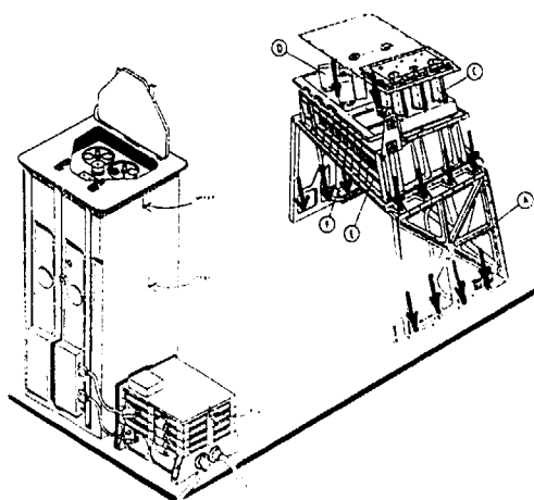
Figure 9 Equipment/base substructures in a space microgravity experiment set-up
