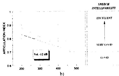
Figure 20-16 - ANR effects on AI vs. indicated air speed (rear cockpit), a) UHF/VHF radio communication, b) interphone communication
