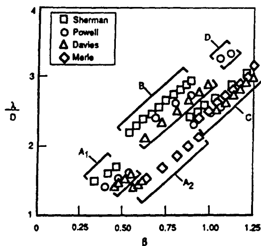
Figure 3: Screech modes for an axisymmetric sonic nozzle.
