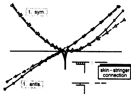
Fig. 4-1 TYPICAL MODE SHAPES OF COUPON 1-I influence of rivet modeling
