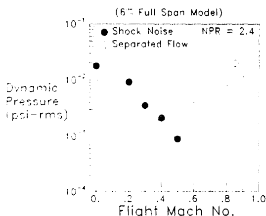
Figure 19. Dependence of flight on peak dynamic pressure amplitudes.
