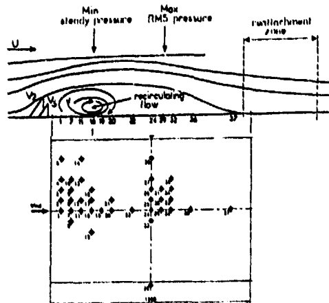
Figure 9 : Location of pressure measurements
