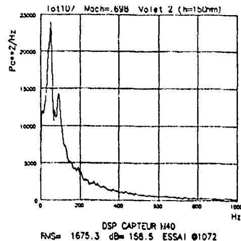
Figure 10 : Wind-Tunnel tests : Typical Pressure Spectral Densities ( \text{Pa}^2/\text{Hz} ) vs Frequency (Hz)
