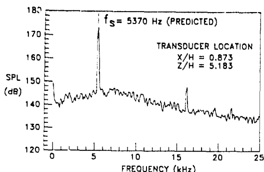
Figure 31. Dynamic loads in cruise mode from model scale ASTOVL studies.
