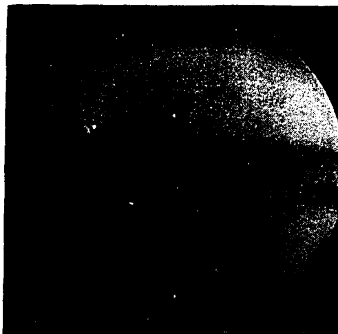
b. phase averaged schlieren of suppressed mode
