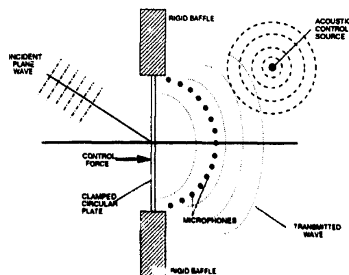
Figure 5: Active noise/vibration control systems.
