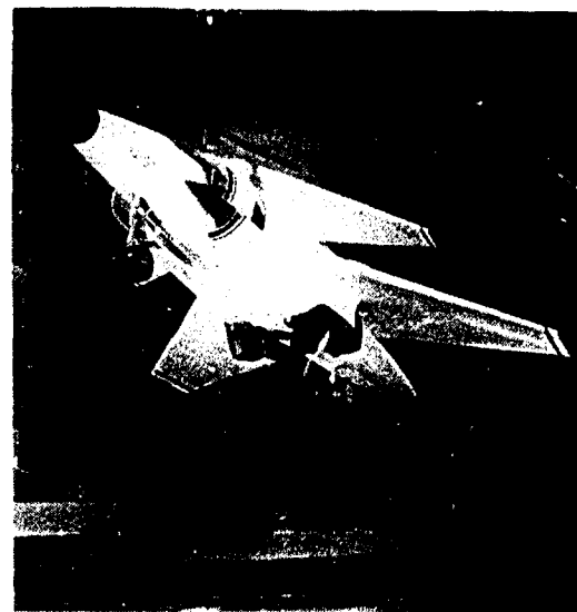
Figure 27. ASTOVL 9.2% model in NASA Lewis 9X15 Wind Tunnel. (from Ref. 24)
