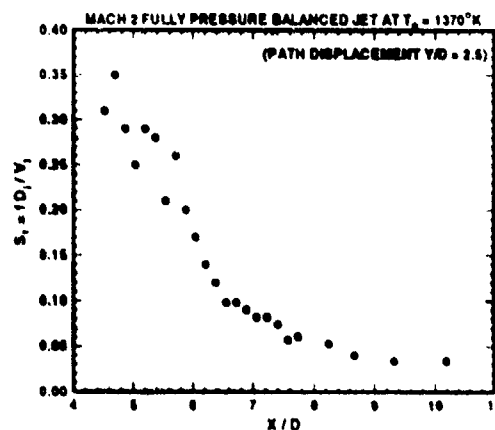
Figure 2 Strouhal frequency of peak acoustic energy along co-linear path to jet axis at Y/D = 2.5
