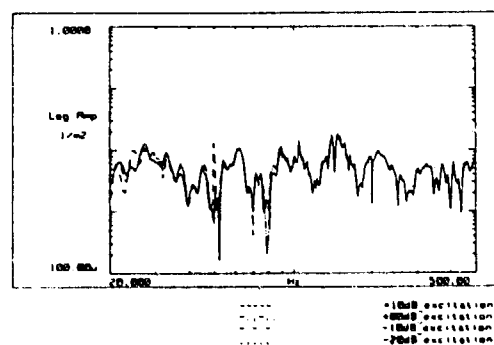
Figure 5 FRF linearity with reciprocal excitation
