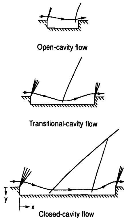
Fig 1 Three types of cavity flow
