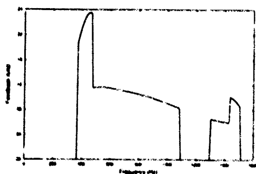
Figure 12: M_\infty = .1 , Shear layer growth rate = .1.
