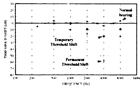
Figure 20.1 - Typical pure tone audiograms
