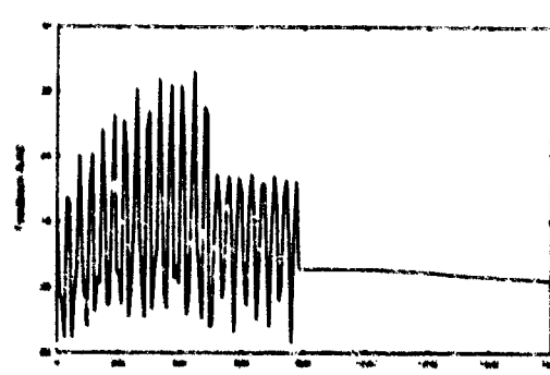
Figure 15: M_\infty = .95 , Shear layer growth rate = .1.
