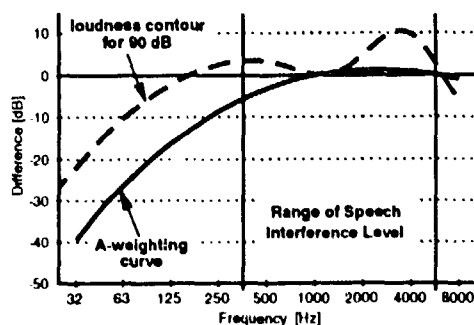
Figure 4: Comparison of A-weighted Curve with Loudness Sensitivity Curve for 90 dB(A)
