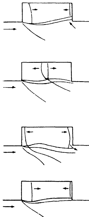
Fig 3 Sketch of basic cavity phenomenon
