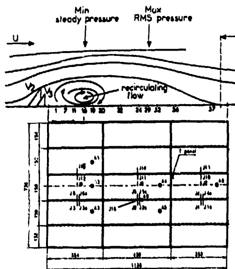
Figure 12 : Location of strain gauges on test box
