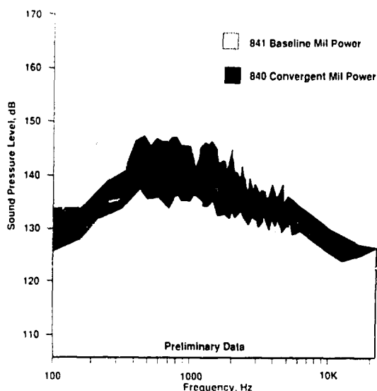
Figure 23. F-18 HARV aircraft inter-nozzle spectra.
