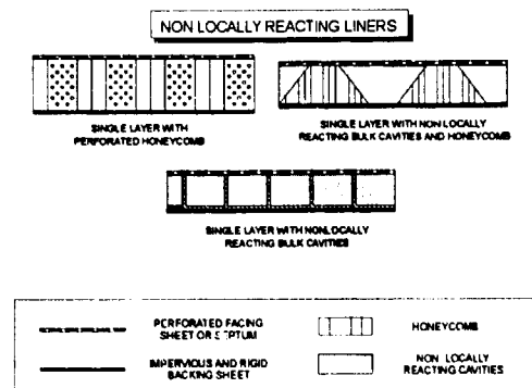
Figure 5.14 - Typical configurations of circumferential non locally reacting liners currently under investigation inside a CEC research
