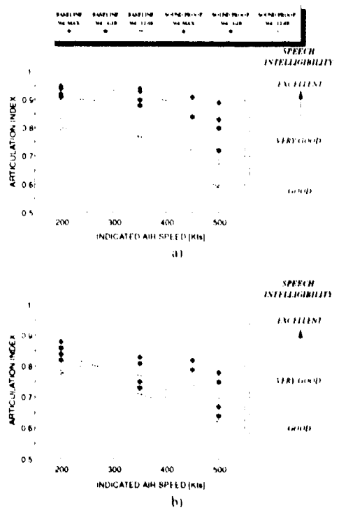
Figure 20.13 - Noise insulation kit effects on AI vs. indicated air speed (rear cockpit): a) UHF-VHF radio communication; b) interphone communication
