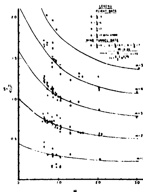
Fig 6 Non-dimensional resonant frequencies as a function of Mach number
