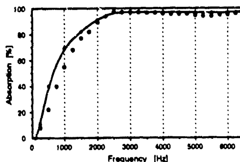
Figure 8: Comparison of Measured (●) and Calculated (*) Absorption Coefficients
