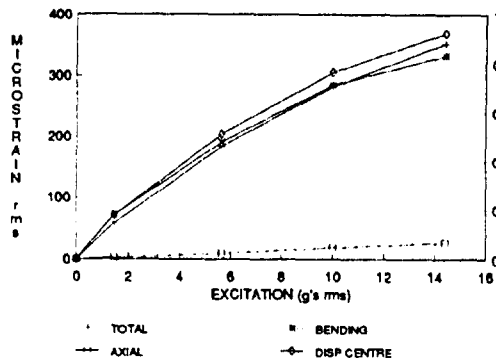
Fig 6 Total, Axial, Bending Strains, SG 2, Random, Aluminum Plate
