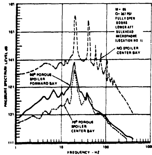
Fig 11 Forward and center bay acoustic levels (Ref 24)
