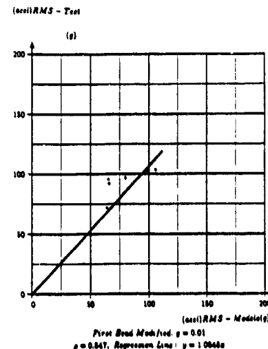
Figure 12: Predicted vs Test Stress and Acceleration Correlation
