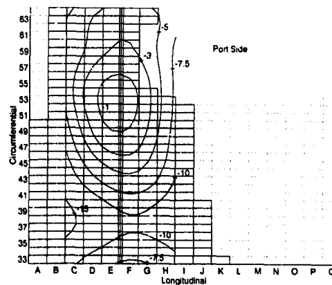
Figure 13: Propeller pressure field magnitude, dB with respect to peak, on port side of aircraft, 1x BPF. The area under the wing-box shroud is left blank. Elements shown dotted were not scanned.
