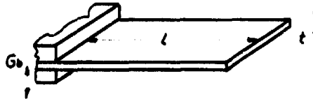
Fig. 9: Model cantilever beam acceleration excited
