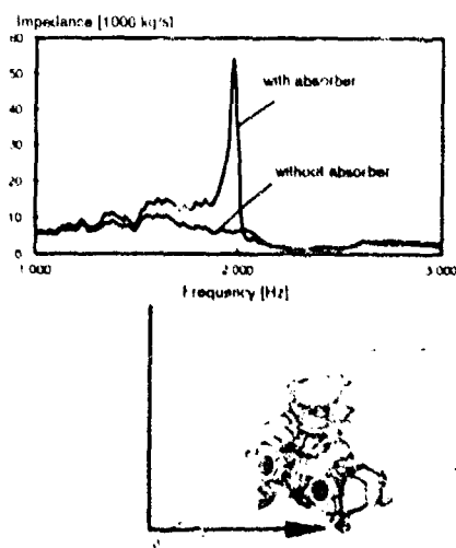
Figure 17: Impedance Measurements on one of the Four Vertical Gearbox Levers With and Without Absorbers
