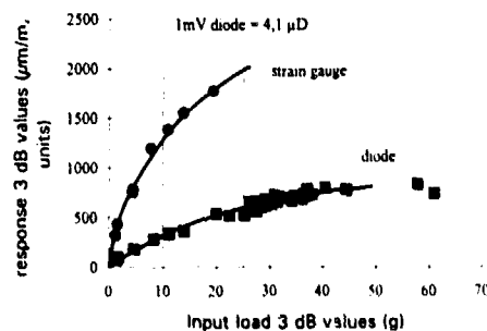
Fig. 5: Example of the calibration of the diode using strain gauge results (3dB-values)
