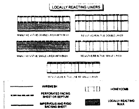
Figure 5.12 Typical configurations of locally reacting liners
