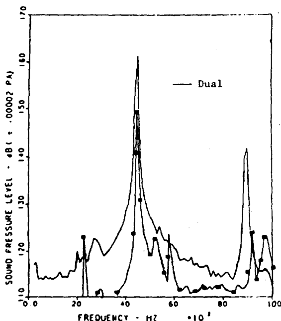
Figure 4: Single vs twin jet sound pressure levels.
