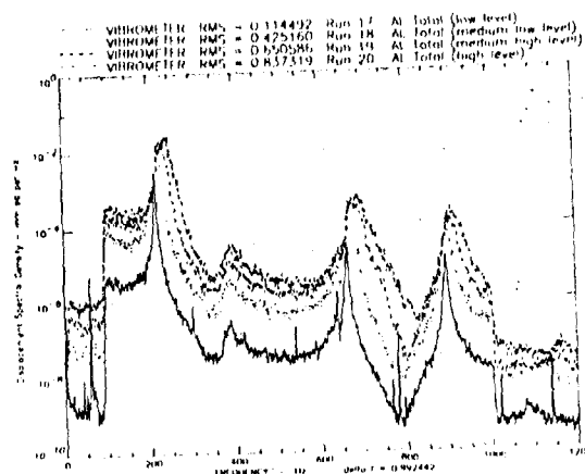
Fig 11 Displacement Spectral Densities, Random, Aluminum Plate
