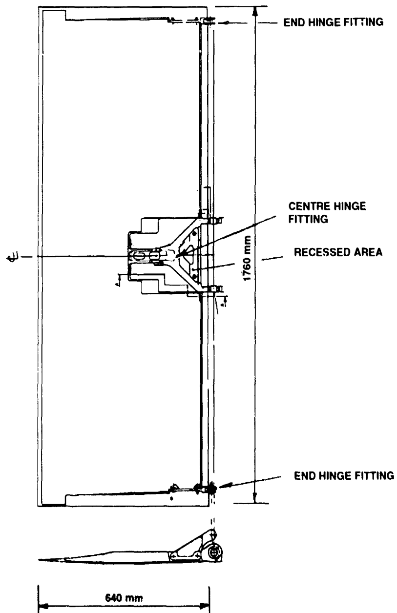
FIGURE 4 GENERAL ARRANGEMENT OF THE SPFDB TITANIUM SPOILER (BOTTOM SURFACE SHOWN)
