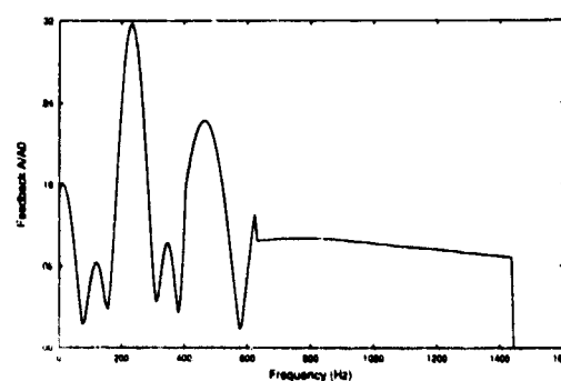
Figure 13: M_\infty = .7 , Shear layer growth rate = .1.
