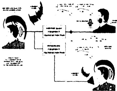
Figure 20.3 - Articulation Index calculation procedure
