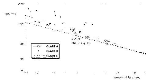
Fig. 13 Endurance plots: influence of lay-up configuration - plain specimens
