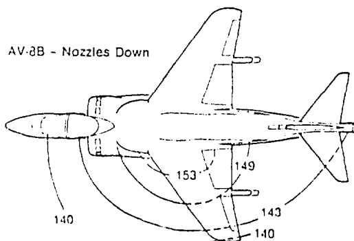
Figure 25. AV-8B take-off dynamic pressure load levels.
