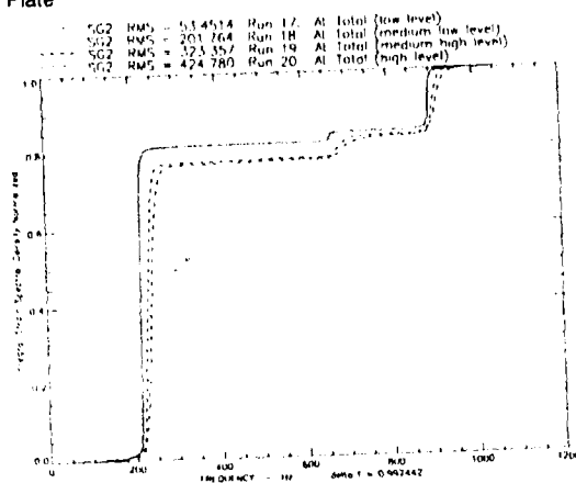
Fig 12 Integral Strain Spectral Density, SG 2, Random, Aluminum Plate
