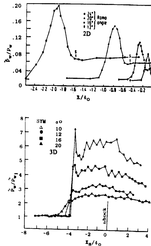
Figure 2. Normalized rms pressure distribution with 2D (Ref. 14) and 3D (Ref. 15) shock strength
