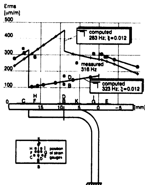
Fig. 4-2 STRAIN DISTRIBUTION IN SKIN (coupon 1-I, 1g^2/Hz ; 100-1000 Hz)
