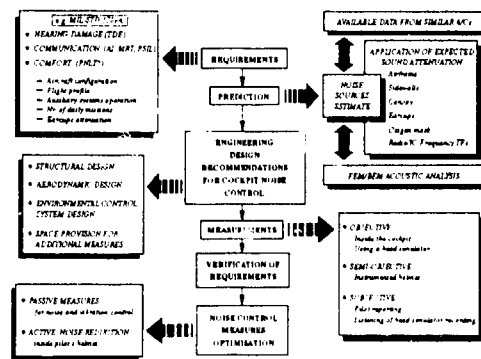
Figure 20-2 - Cockpit noise design and verification
