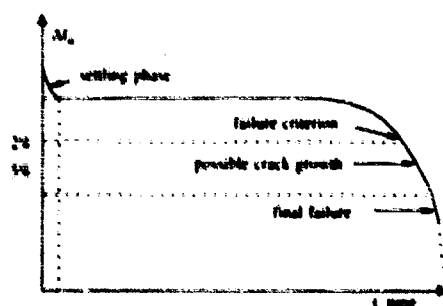
Fig. 7 Failure criterion for shaker specimens
