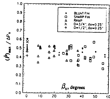
Figure 5. Normalized peak rms pressure with pressure rise across separation shock (Ref. 13)
