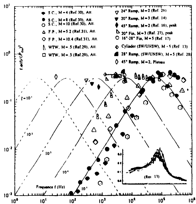
Figure 8. First moment of PSD for attached and separated flow conditions
