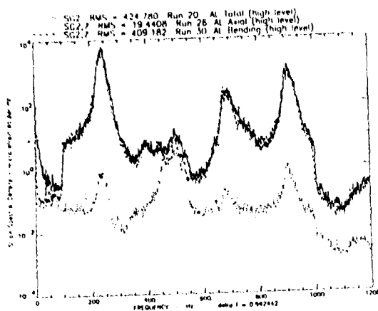
Fig 10 Strain Spectral Densities, SG 2, Total, Axial, Bending, High Level, Random, Aluminum Plate
