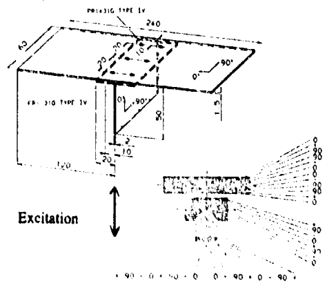
Figure 1 : Typical coupons
