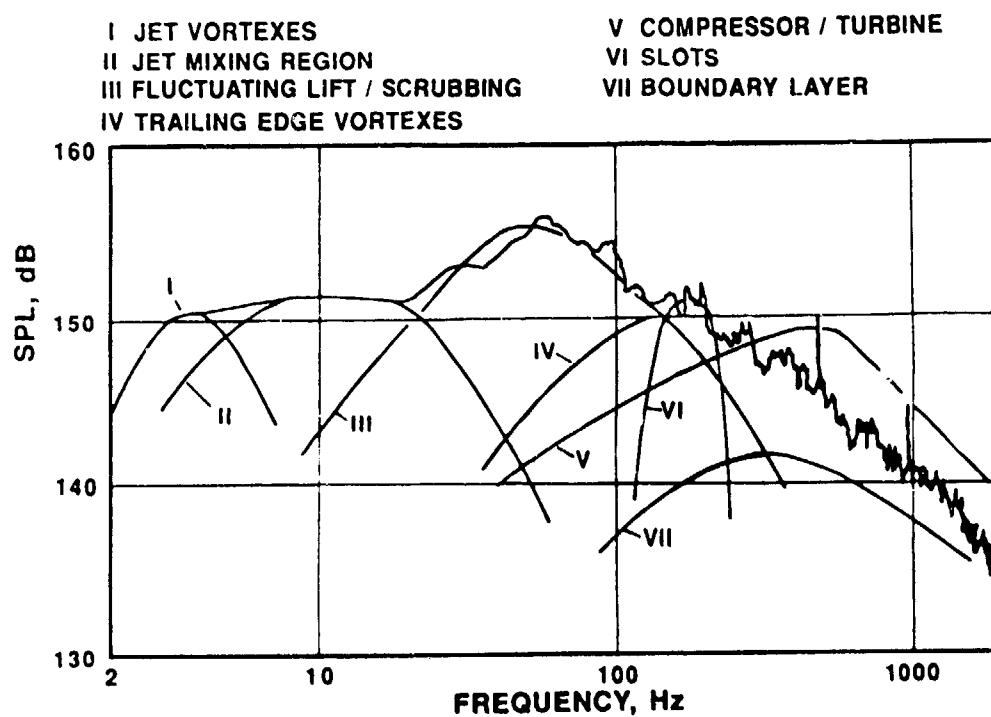
Figure 1. Acoustic Environments Experienced by Jet Aircraft
