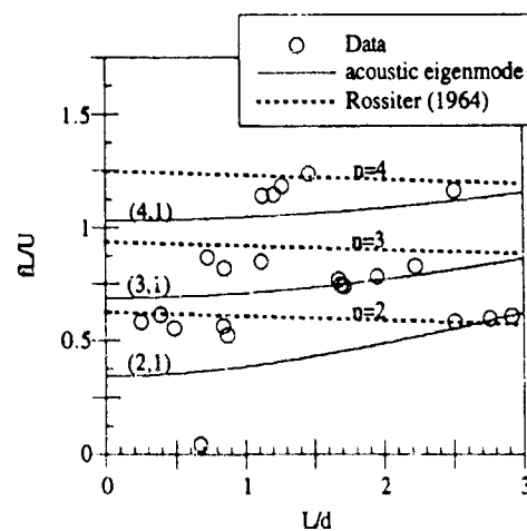
Fig 7 Comparison of cavity acoustic modes and Rossiter's equation (Ref 14)
