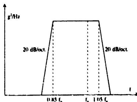
Fig. 6 Shaker narrow-band loading
