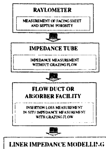
Figure 5.15 - Locally reacting liners development tools
