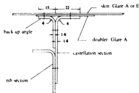
Fig. 24 Rib-castellation details after repairs
