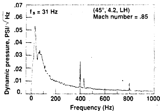
Figure 16. Typical engine outer divergent flap dynamic loads spectrum from B-1B flight test program (from Ref. 2).
