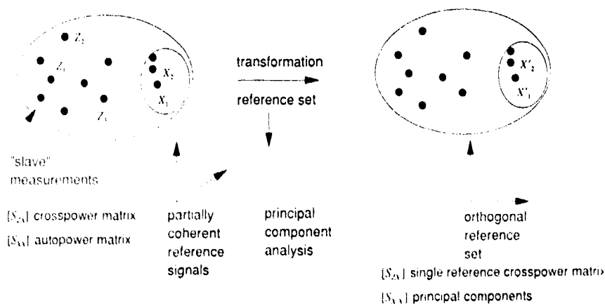
Figure 2 Decomposition of multi-reference problem into set of single reference problems
