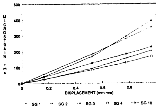
Fig 16 Displacement vs Strain, Random, CFRP Plate
