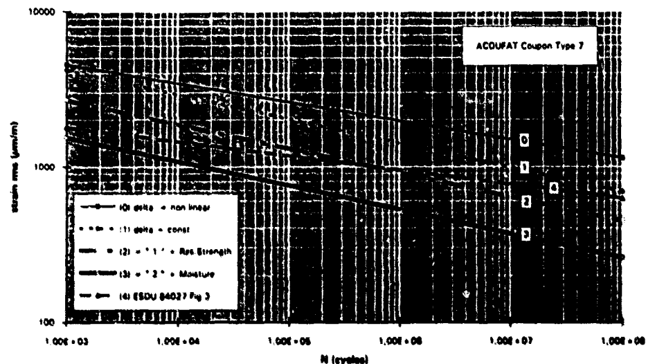
Fig 16: \epsilon_{rms}/N curve for coupon type 7 "ACOUFAT" determined with constant damping, covering the influence of residual strength and moisture / temperature. Additional with ESDU 84027 Fig. 3 (CFRP) for comparison.
