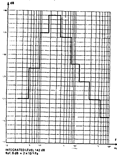
Fig.2 Acoustic spectrum at firing for Ariane 4 (from Arianespace, 1983)
