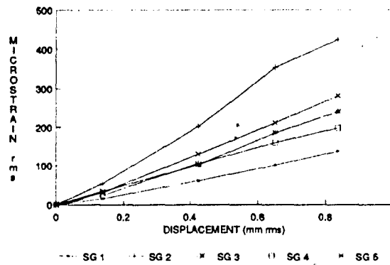
Fig 7 Displacement vs Strain, Random, Aluminum Plate
