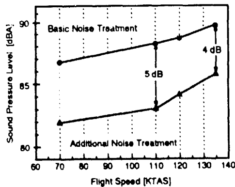
Figure 20. BK 117 Measurement Results Before and After Additional Passive Noise Treatment
