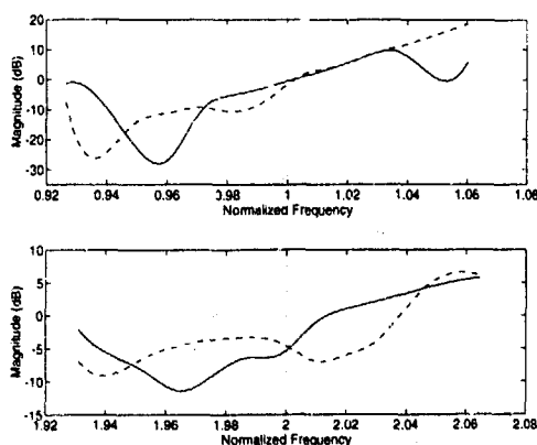
Figure 14: Normalized internal noise prediction at location 1 (solid) and location 2 (dashed). At 1×BPF (upper) and 2×BPF (lower). The frequency of interest is shown by the dotted line.
