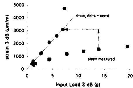
Fig. 10: Strain versus input load (3 dB values) at constant damping
