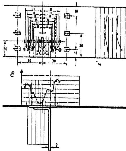
Figure 6 : Measured strain distribution for L-shaped HTA / 6376 coupon with landing
