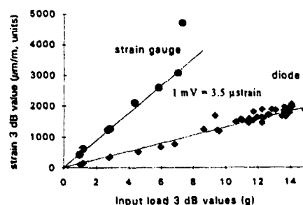
Fig. 12: Calibration of the diode using the 3dB-values ( \delta = \text{constant} )
