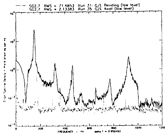
Fig 18 Strain Spectral Densities, Bending, Axial, Low Level, Random, CFRP Plate
