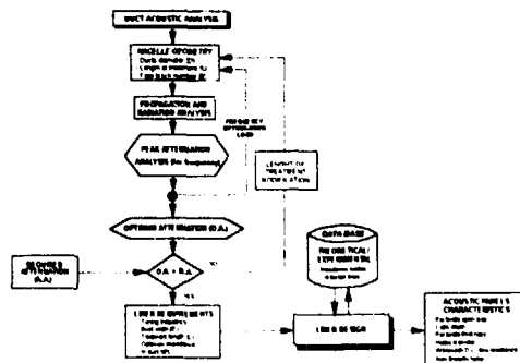
Figure 5-9 - Duct-acoustic analysis and liner design procedure
