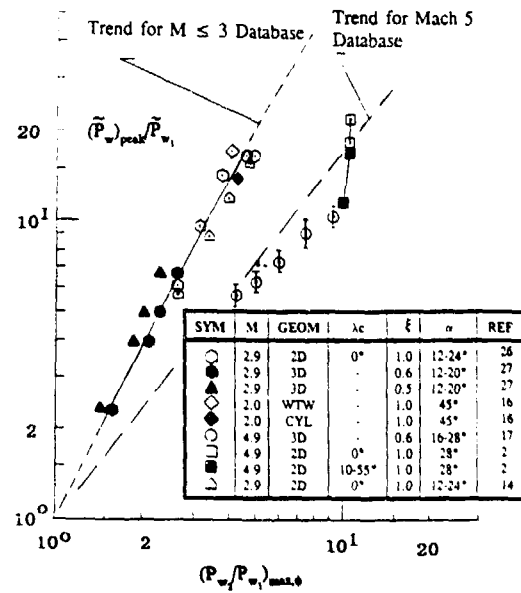
Figure 3. Correlation of peak rms pressure with modified oblique shock relationship (Ref. 1)
