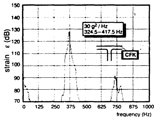
Fig. 3-1 AUTOSPECTRUM OF STRAIN IN SKIN (coupon 8-IV; two different bandwidths of excitation; \Delta f=2.5 Hz)
