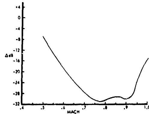
Fig 13 Optimized Suppression of Maximum Oscillation (Ref 24)
