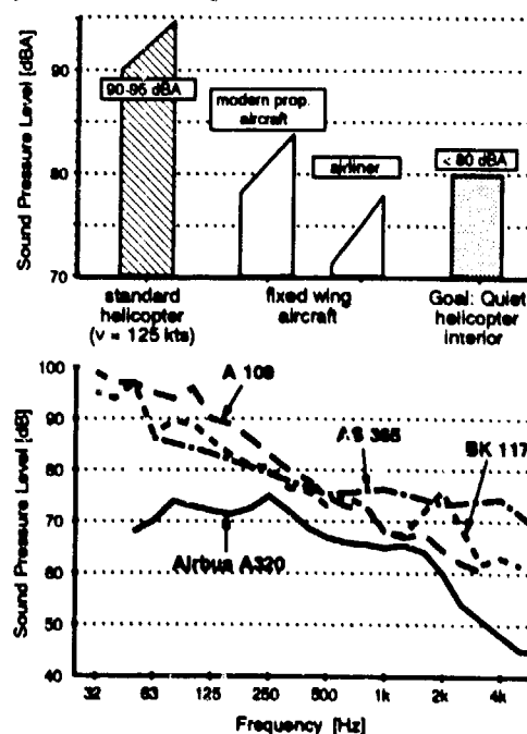
Figure 1: Interior Noise Levels of VIP-sound-proofed Helicopters Compared to Fixed Wing Aircraft
