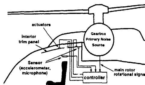
Figure 22: Principle Scheme of Active Panel Control
