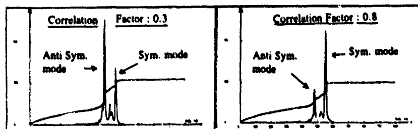
Figure 19 : Finite Element simulation of the influence of the correlation factor on the structural response : Comparison of the PSD response of strain gauge 1, for
