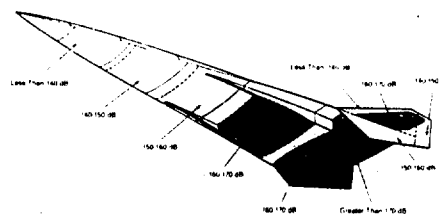
Figure 8 Overall Sound Pressure Levels relative to 20 micro Pa due to engine noise at takeoff.
