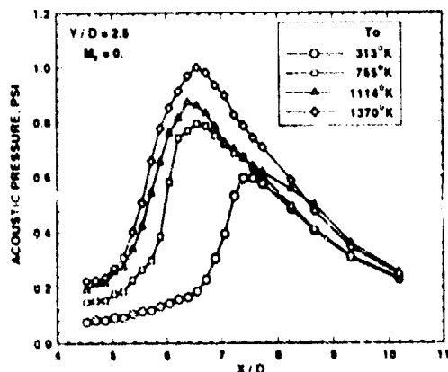
Figure 1 Near Field Acoustic Pressure Along Co-linear Path to the Jet Axis
