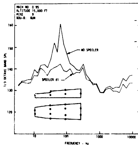
Fig 5 Full scale F-111 weapons bay spectra
