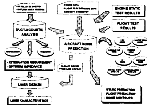
Figure 5.19 - Structure of Alenia Noise Integrated Software (ALNOIS) package
