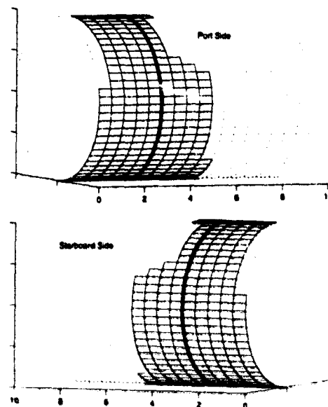
Figure 6: Fuselage scan elements for which noise transmission is measured. The area under the wing-box shroud is left blank. Elements shown dotted were not scanned. The propeller plane is marked with a solid line.
