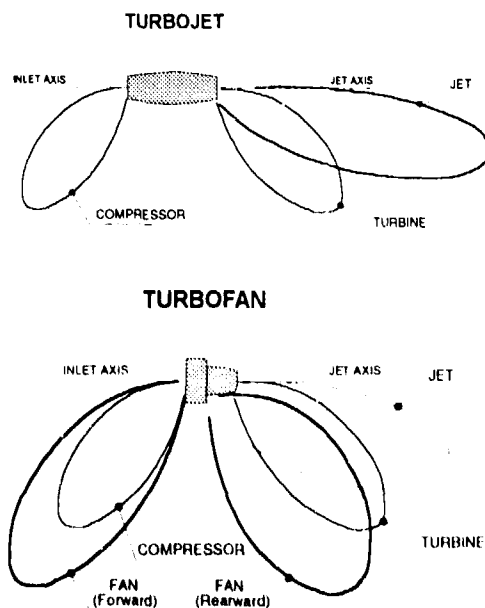
Figure 5.1 - Noise sources directivity of turbojet and turbofan engines
