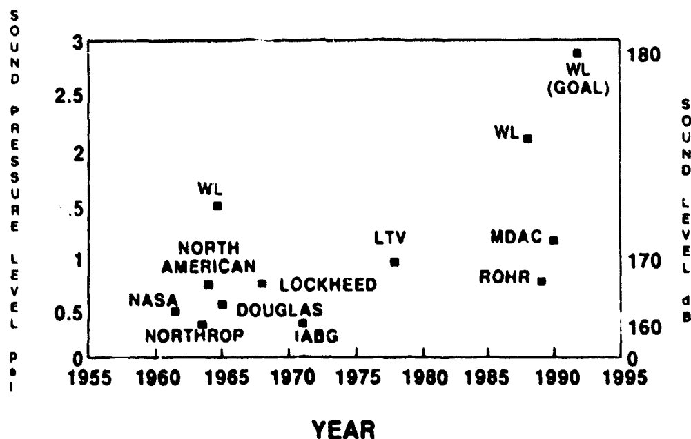
Figure 8 - High Intensity Acoustic Testing Capabilities
