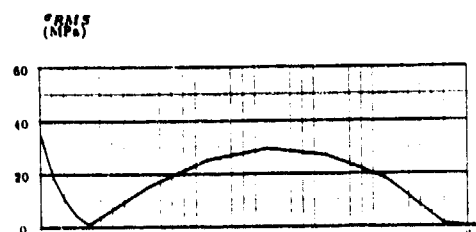
Figure 11: Theoretical stress output at central line elements
