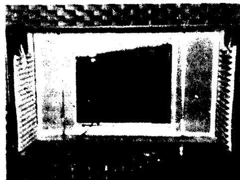
Figure 10: Test Set-up for Improvement of Cabin Door Transmission Loss
