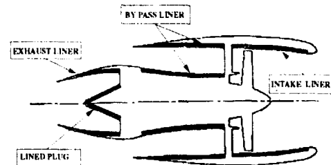
Figure 5.2 - Typical acoustic liner installation in a current HBPR turbofan engine
