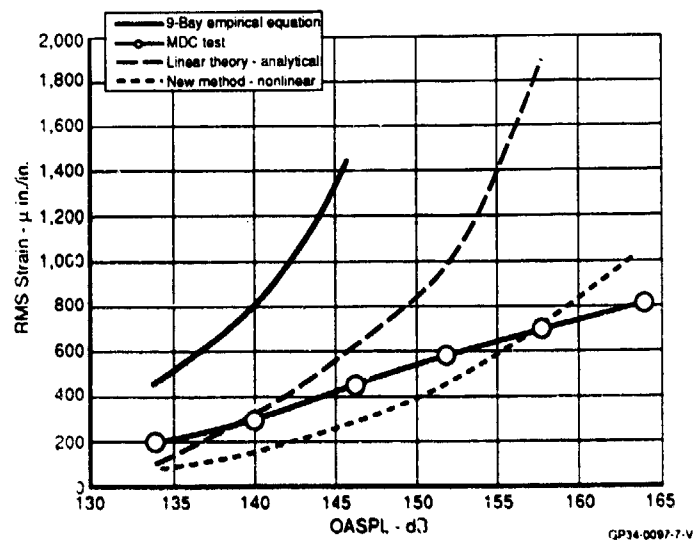
Figure 6. Strain Response Under Acoustic Excitation of Clamped Aluminum Panel 10 in. x 20 in. x 0.063 in. 7075-T6 Panel, Narrow Band Random Excitation
