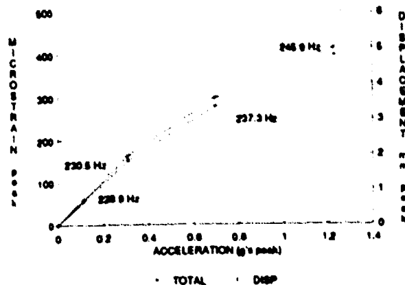
Fig 3 Acceleration vs Strain and Displacement, Sine Dwell Aluminum Plate
