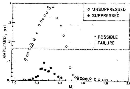
Figure 6. Magnitude of inter-nozzle dynamic pressures in unsuppressed and suppressed modes.
