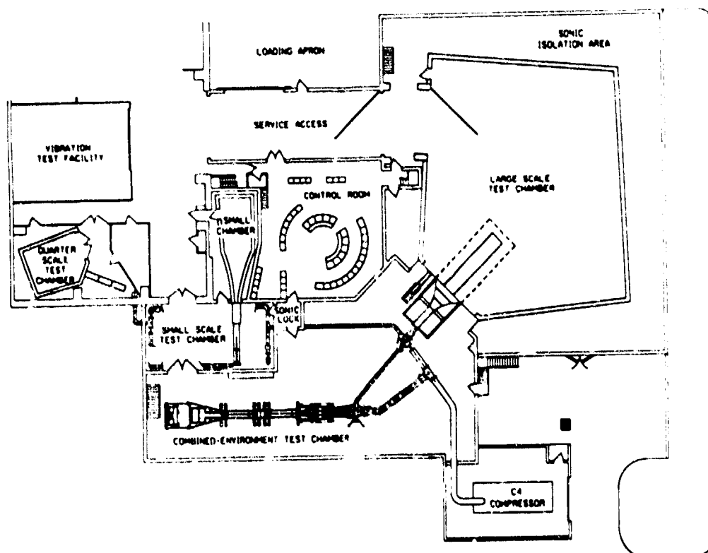
Figure 2. The Wright Laboratory Structural Dynamics Facility
