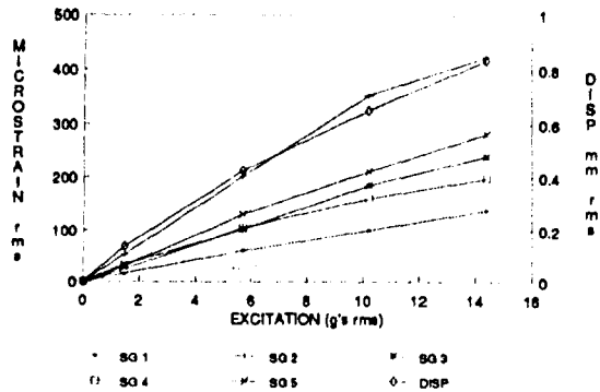
Fig 5 Excitation vs Strain and Displacement, Random, Aluminum Plate
