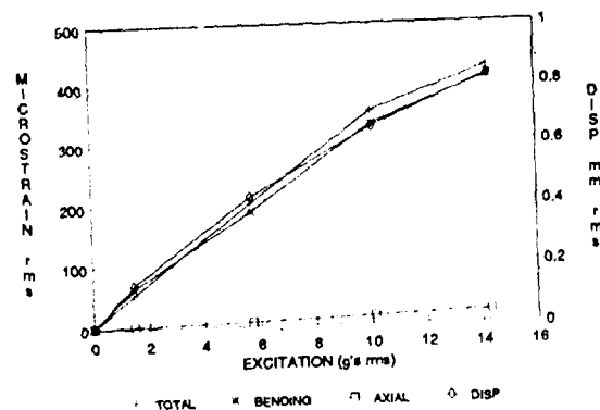
Fig 15 Total, Axial, Bending Strain, SG 2, Random, CFRP Plate
