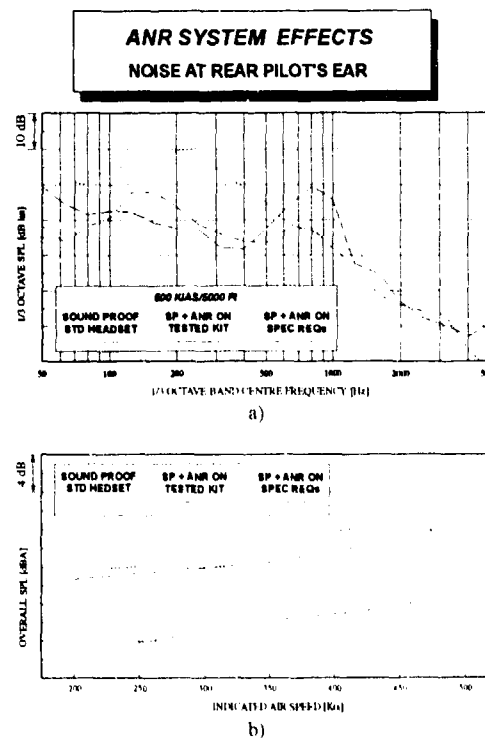
Figure 20 14 - ANR benefits at rear pilot's ear. a) typical spectrum shape modification. b) dBA OASPL reduction
