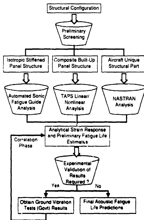
Figure 4. Acoustic Fatigue Design Approach
