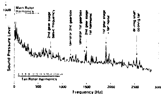
Figure 6: Typical Interior Noise Spectrum in an Untreated Small Size Helicopter
