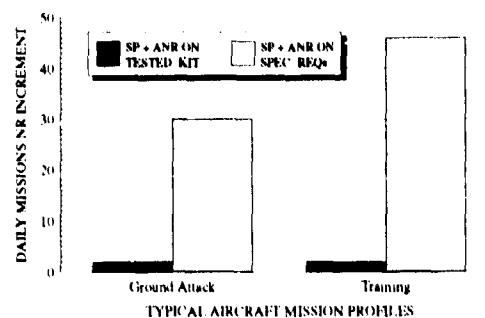
Figure 20 15 - ANR benefits in terms of daily missions number increment (rear cockpit)
