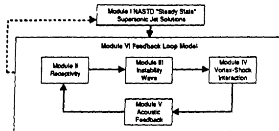
Figure 5: Screech prediction tool flowchart.
