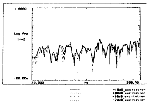
Figure 4 FRF linearity with direct (structural) excitation
