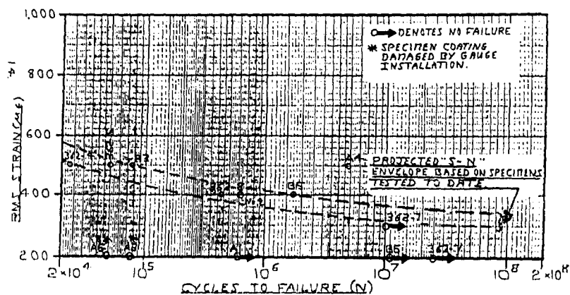
Figure 12 Random fatigue shaker test data for carbon-carbon coupons at 1800 F (980 C).
