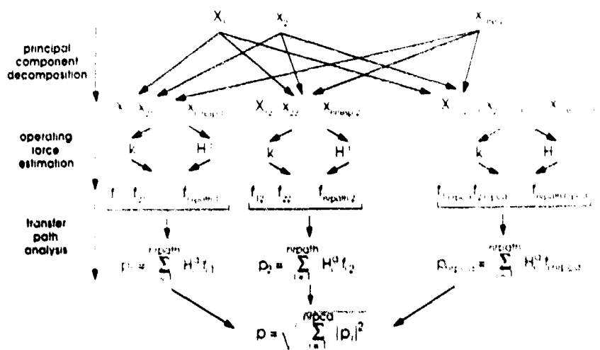
Figure 3 Schematic presentation of multireference transmission path analysis
