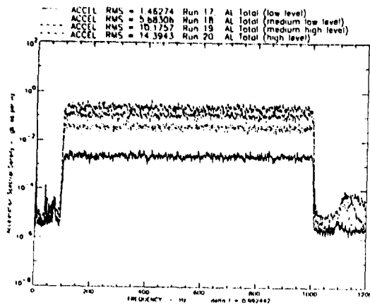
Fig 4 Acceleration Spectral Density
