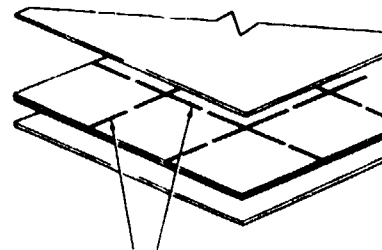
Four Sheet SPF/DB The Core Sheets* are joined at the locations where internal stiffeners are required
