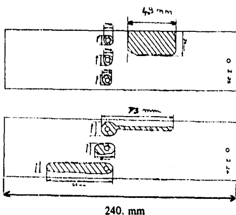
Figure 2 : Typical delamination areas, with CFRP T800/924 coupons
