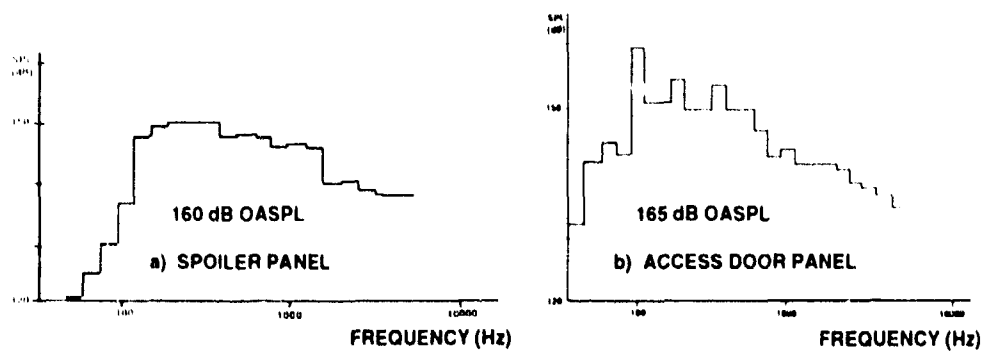
FIGURE 6 ACOUSTIC EXCITATION : 1/3 OCTAVE BAND SPECTRUM
