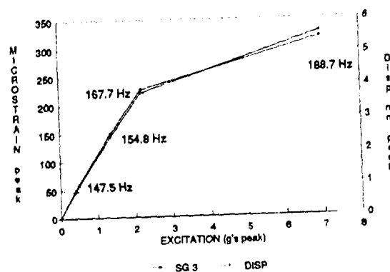
Fig 13 Acceleration vs Strain and Displacement, Sine Dwell, CFRP Plate
