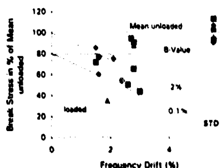
Fig. 15: Results of compression tests of loaded and unloaded (type 7 coupons)
