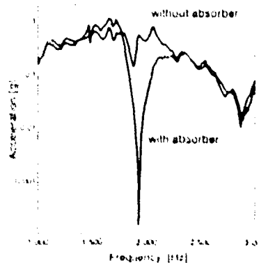
Figure 19: Vibration Transmission Frequency Response of a Gearbox Strut With and Without Absorber
