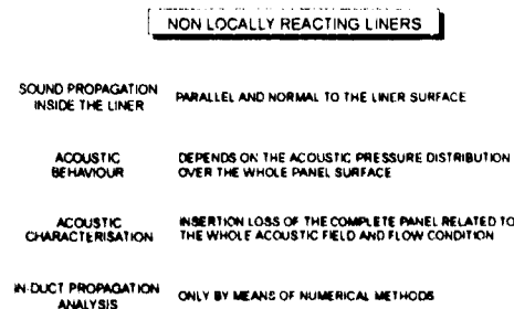
Figure 5.13 - Non locally reacting liners properties
