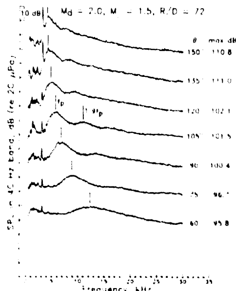
Figure 1 Example shock noise spectrum showing broadband and screech components
