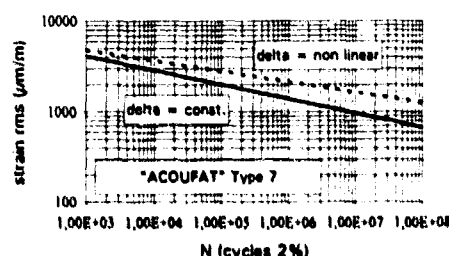
Fig. 13: \epsilon_{rms}/N curve of coupon type 7 with and without linear calibration
