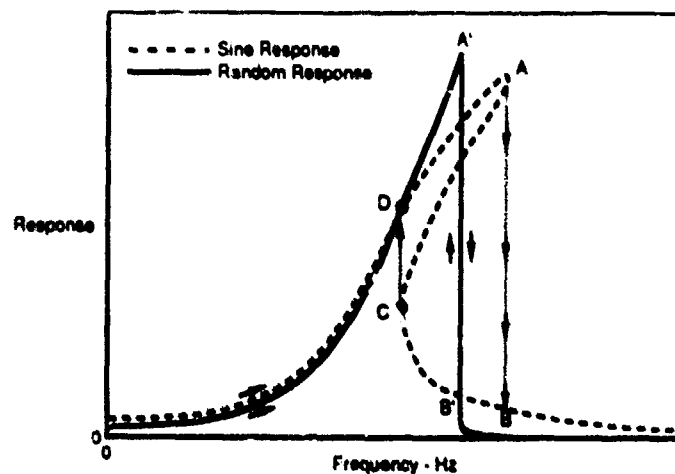
Figure 2. Sine and Random Nonlinear Response Functions
