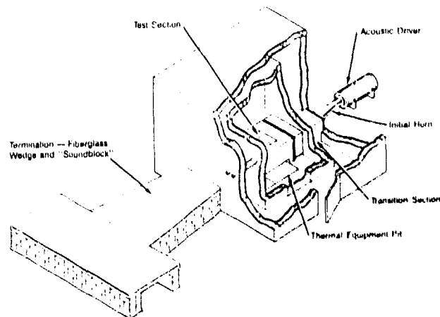
Figure 11 Thermal Acoustic Progressive wave tube.
