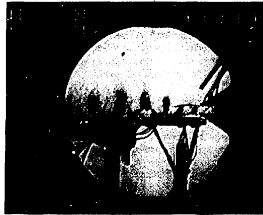
Figure 30. Schlieren image of supersonic jet plume scrubbing in ASTOVL cruise mode.
