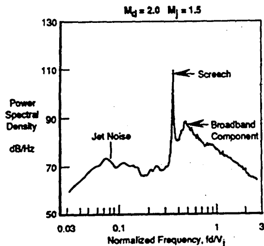
Figure 2: Power spectral densities for jet mixing noise, broadband shock associated noise and screech.
