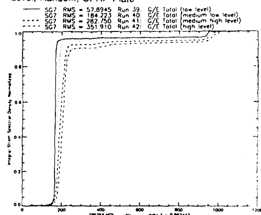
Fig 21 Integral Strain Spectral Density, SG 7, Random, CFRP Plate
