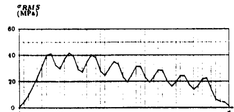
Figure 10: Theoretical stress output at elements adjacent to clamped edge
