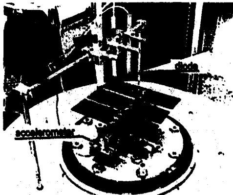
Fig. 2: Coupons mounted on the excitation table
