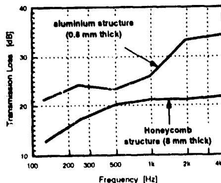
Figure 3: Transmission Loss of Pure Aluminium Structure and Honeycomb Structure (8 mm)
