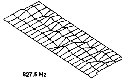
b) TYPICAL SPOILER RESPONSE MODE IN HIGHER FREQUENCY RANGE
