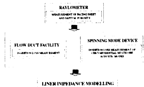
Figure 5.17 - Non locally reacting liners development tools
