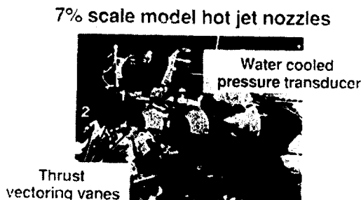
Figure 22. HARV 7% scale model nozzle afterbody.
