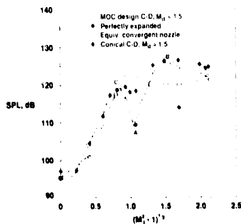
Figure 4 Shock noise amplitude behavior of convergent and convergent-divergent nozzles
