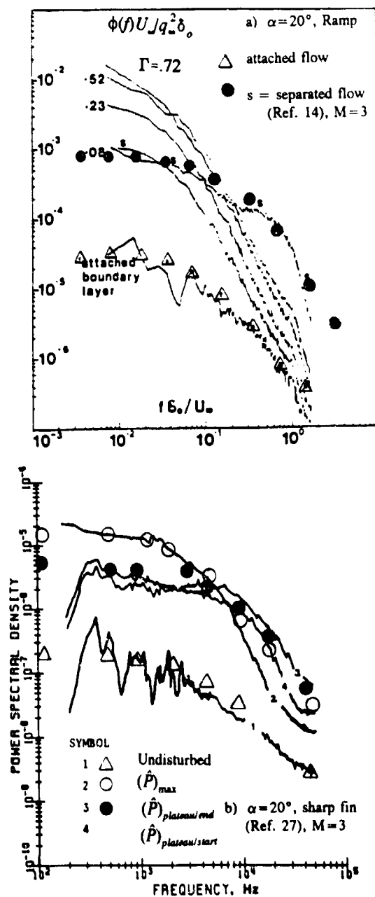
Figure 9. Comparison of the PSD prediction technique to 2D(a) and 3D(b) interactions
