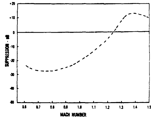
Fig 12 Variation of suppressor effectiveness with Mach number (Ref 23)
