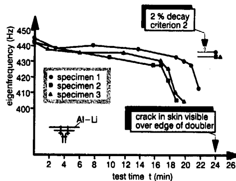
Fig. 3-2 DECAY OF EIGENFREQUENCY coupon 5-II
