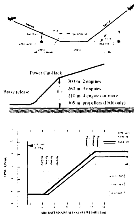
Figure 5.8 - Exemplification of certification requirements for Stage 3 aircrafts
