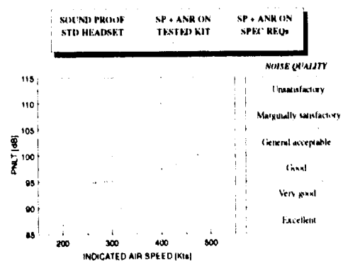
Figure 20-17 - ANR benefits on noise quality
