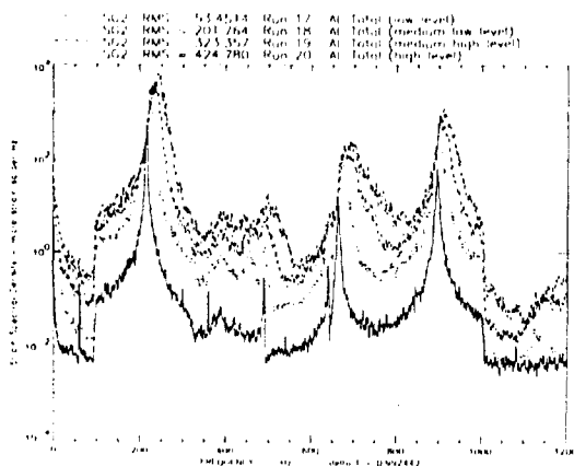
Fig 8 Strain Spectral Densities, SG 2, Random, Aluminum Plate
