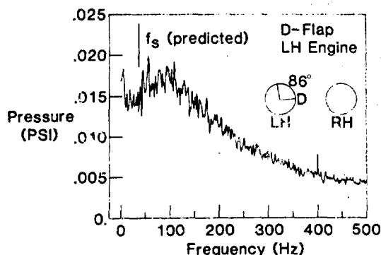
Figure 9. F-15 full scale aircraft outer flap dynamic loads spectrum.
