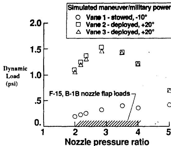
Figure 24. Dynamic pressure loads on thrust vectoring vanes of HARV 7% model.
