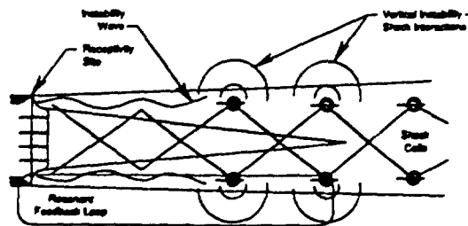
Figure 1: Screech feedback loop.
