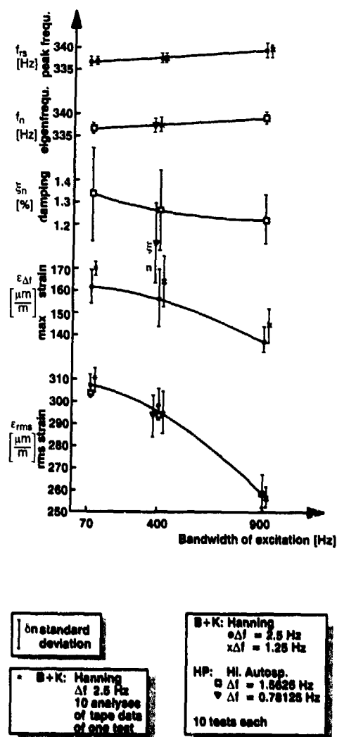
Fig. 4-4 SCATTER AND INFLUENCE OF DIFFERENT TEST CONDITIONS ON TEST RESULTS (VP2 1.6mm; 1g 2 /Hz; skin; averages of 10)
