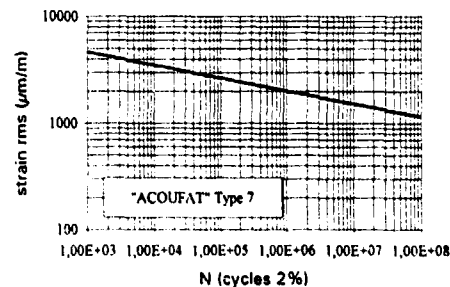
Fig. 7: Calculated \epsilon_{rms}/N curve of coupon type 7 (L - Stringer with landing)
