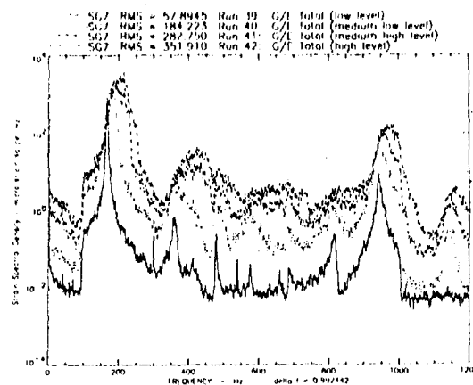
Fig 17 Strain Spectral Densities, SG 7, Random, CFRP Plate
