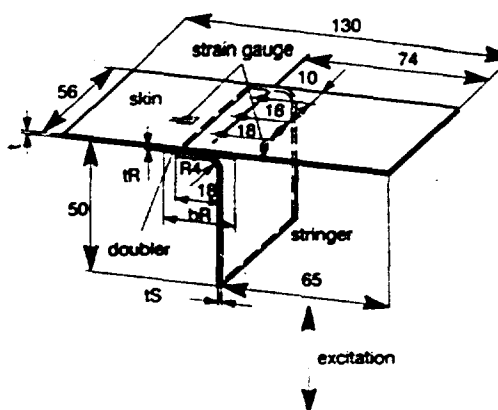
Fig. 2-1 DESIGN OF COUPON
