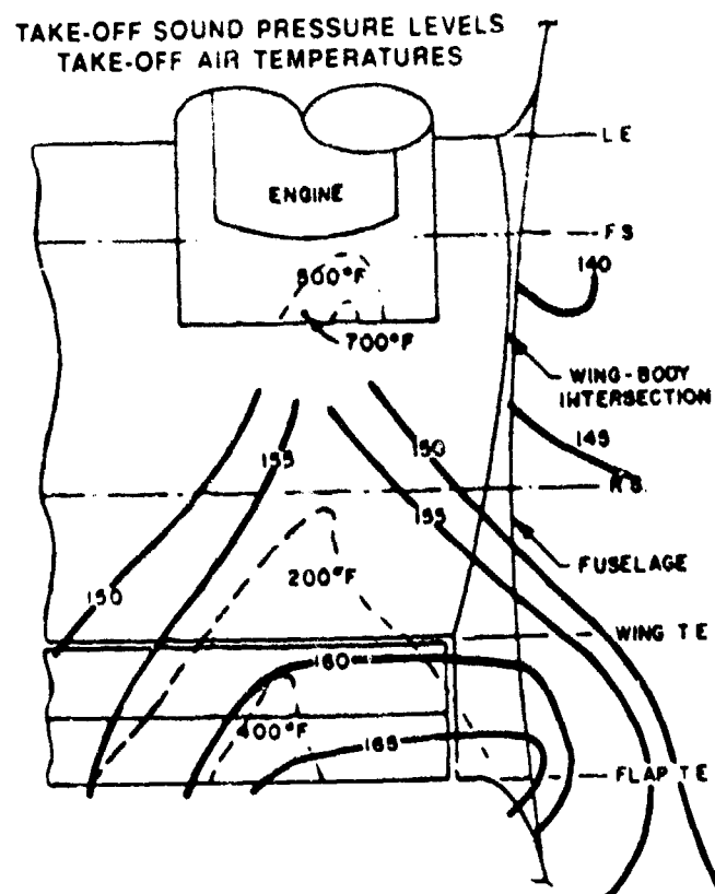
Figure 4. Acoustic and Thermal Environment of High-Lift Devices
