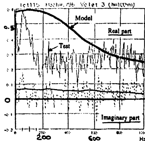
Figure 14 : Comparison Test/Model of the normalized Cross-Spectral densities of fluctuating pressures in WT
