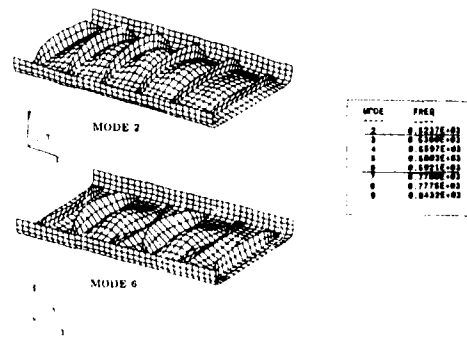
Figure 9 Forebody panel in-phase and out-of-phase vibration modes.
