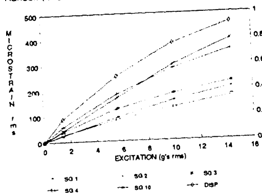
Fig 14 Excitation vs Strain and Displacement, Random, CFRP Plate
