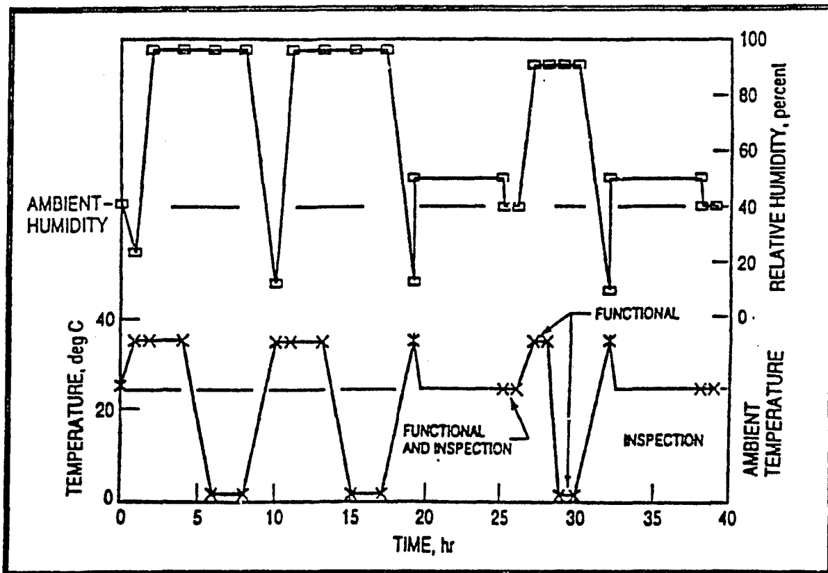
FIGURE 2. Humidity Test Time Line.
