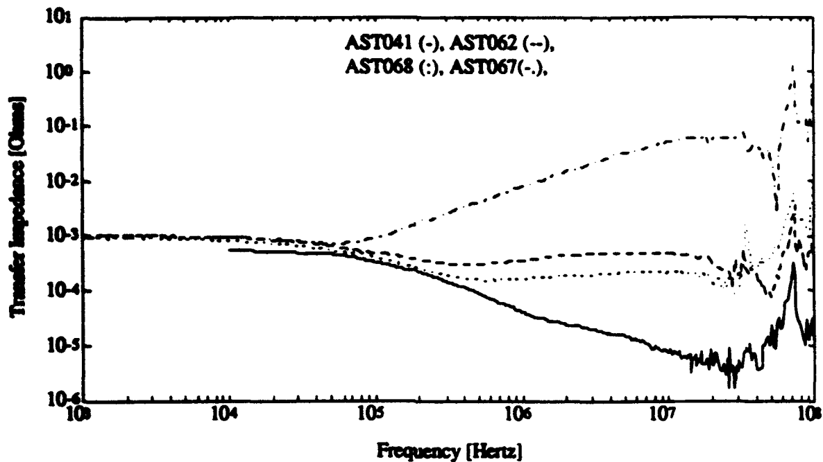
Figure 38. Using trace wire, braid only (AST041), with connector pair (AST062), with connector and 1/2-in fault (AST068), and with connector and 50% fault (AST067).
