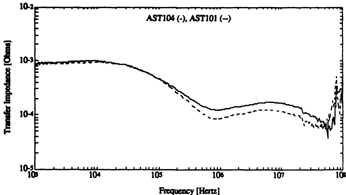
Figure 35. Response of overbraid with brass fixture, baseline (AST101) and with outer layer of overbraid pulled back (AST104).
