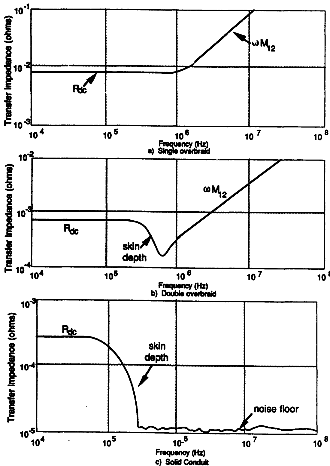
Figure 1. Typical transfer impedance curves.
