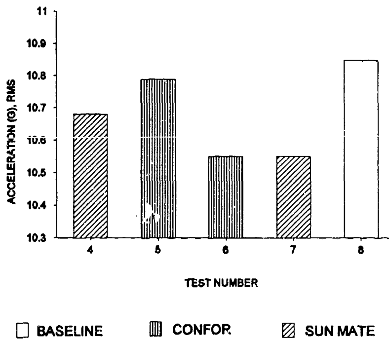
Figure 16. Root mean square pelvic acceleration, z-axis.
