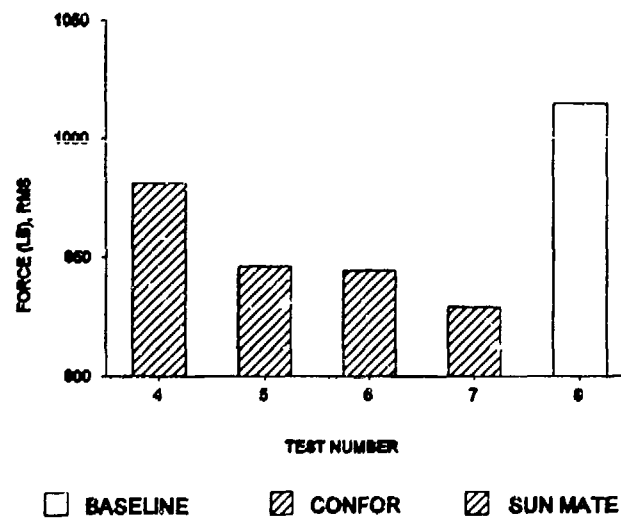
Figure 18. Root mean square lumbar load, z-axis.
