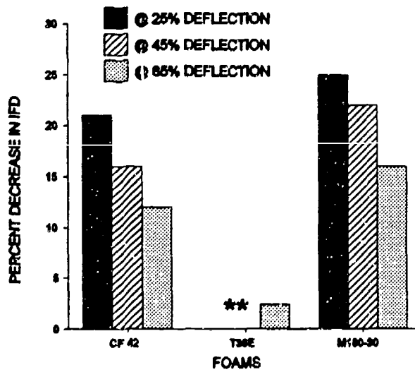
Figure 10. Percent loss in IFD following heat aging and roller shear.
