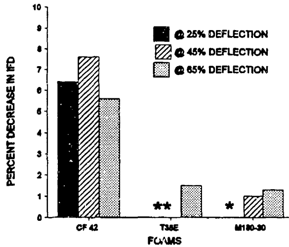
Figure 9. Percent loss in IFD following heat aging.
