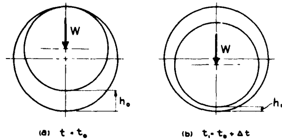
Fig. 14 Film thickness definition
