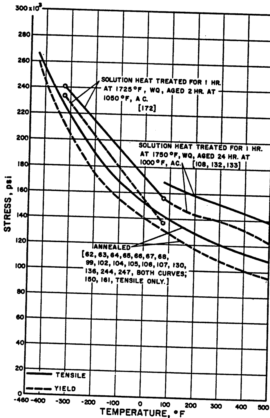
STRENGTH OF C-120-AV TITANIUM
