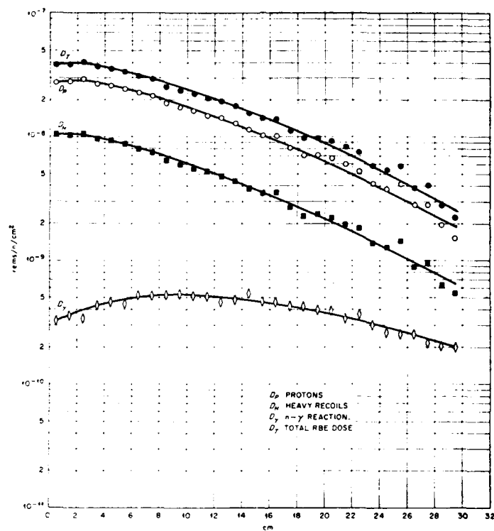
FIGURE 4B. RBE dose (rem) from 5-Mev neutron beam.
