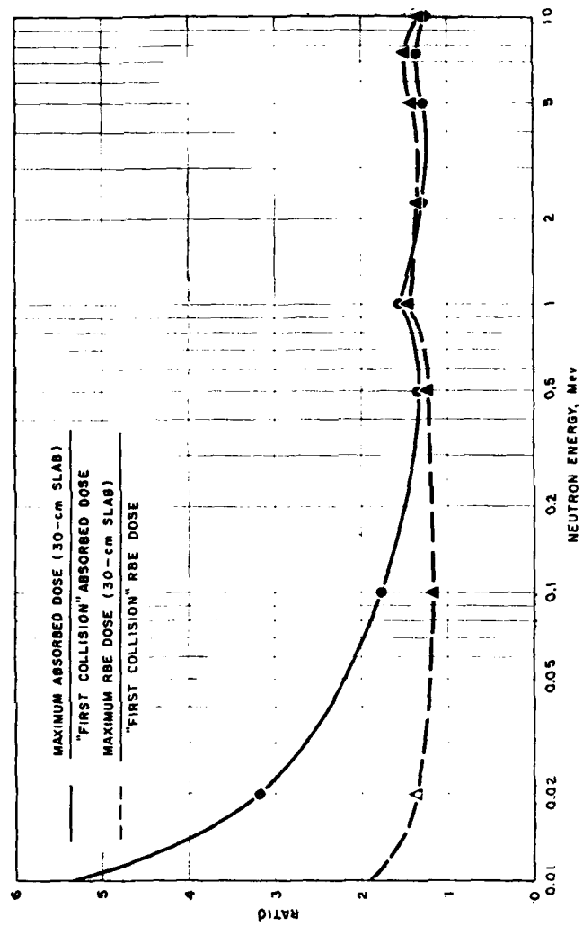
FIGURE 15. Effect of buildup on neutron dose.
