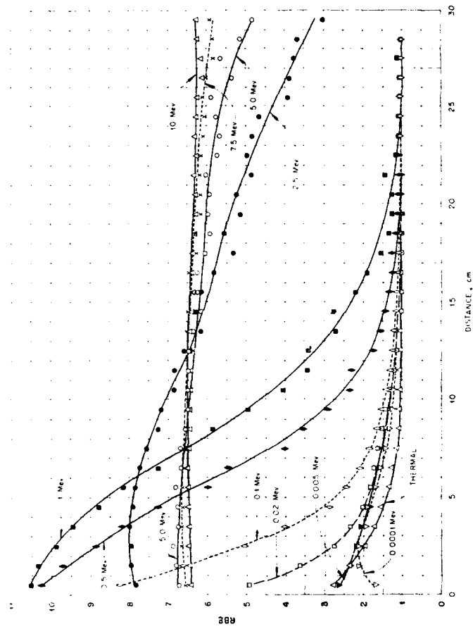
FIGURE 14. RBE ( \approx D_0/E_T ) as a function of depth and neutron energy.
