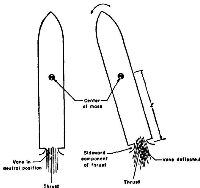
Fig.1 — Jet-vane control
