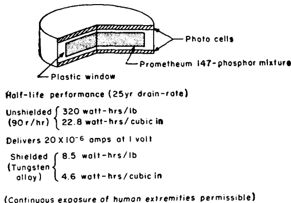
Fig.3 — Promethium battery
