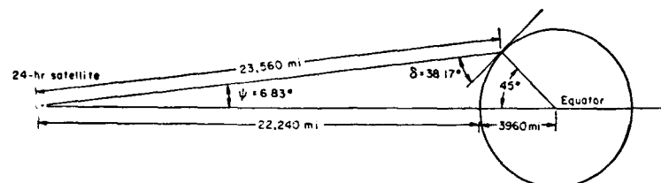
Fig. 5—Viewing an area on the earth at 45° latitude from the "24 hour" satellite
