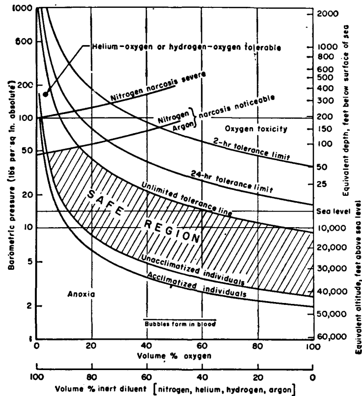
Fig. 3 — Human tolerances—atmospheric composition and pressure
