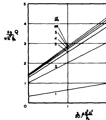
Fig. 6 Variation of flow rate parameter with inertia parameter. r_0' = 0.05 . r_1' = 0.5
