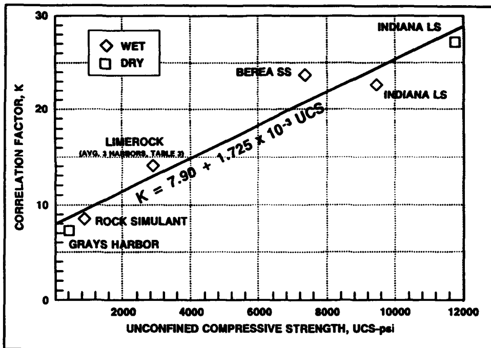
Figure 22. Variations of UCS to I_{sp(NX)} correlation factor for low strength rock
