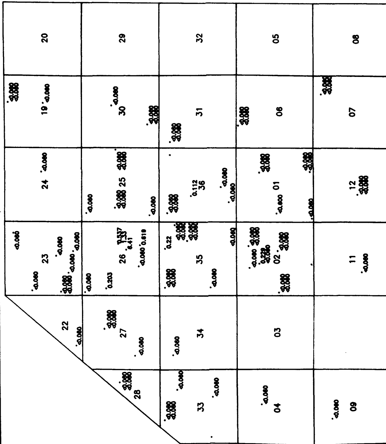
Figure C-18 DIELDRIN CONCENTRATIONS (ug/l) TASK 4 3rd QUARTER DENVER AQUIFER SOURCE: ESE, 1987
