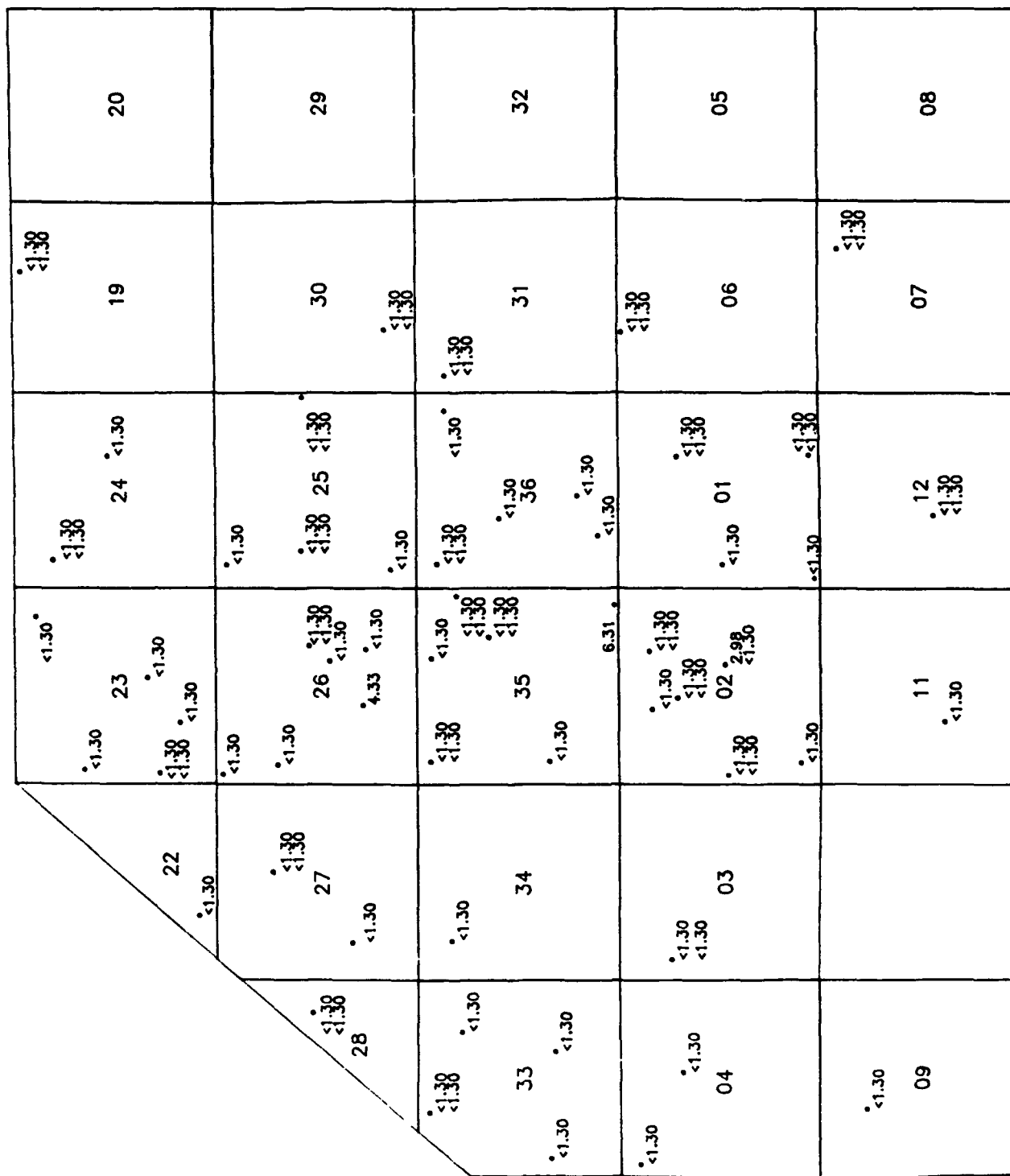
Figure C-136 TCLEE CONCENTRATIONS (ug/l) TASK 4, 4th QUARTER DENVER AQUIFER CALIBRE, ECE 11007
