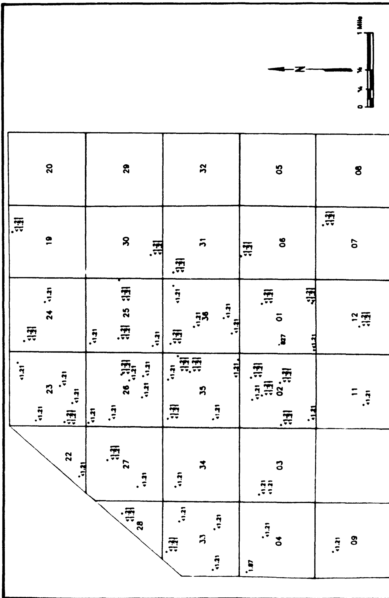
Figure C-80 TOLUENE CONCENTRATIONS (ug/l) TASK 4 4th QUARTER DENVER AQUIFER SOURCE: ESE, 1987
