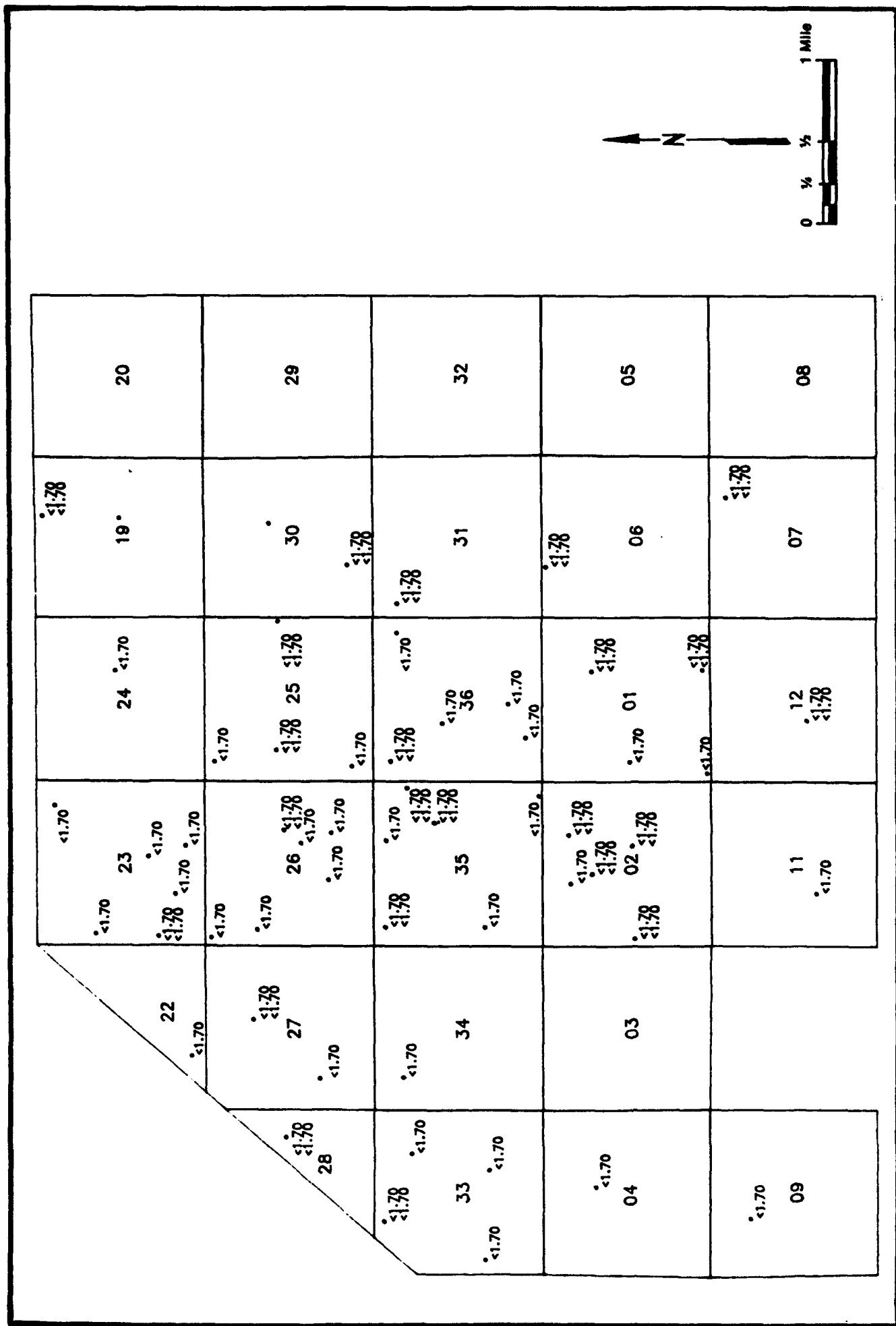
Figure C-118 111TCE CONCENTRATIONS (ug/l) TASK 4, 3rd QUARTER DENVER AQUIFER SOURCE: ESE, 1987
