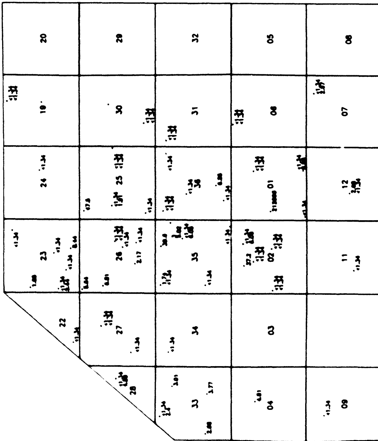
Figure C-74 BENZENE CONCENTRATIONS (ug/l) TASK 4 3rd QUARTER DENVER AQUIFER SOURCE ESE, 1987
