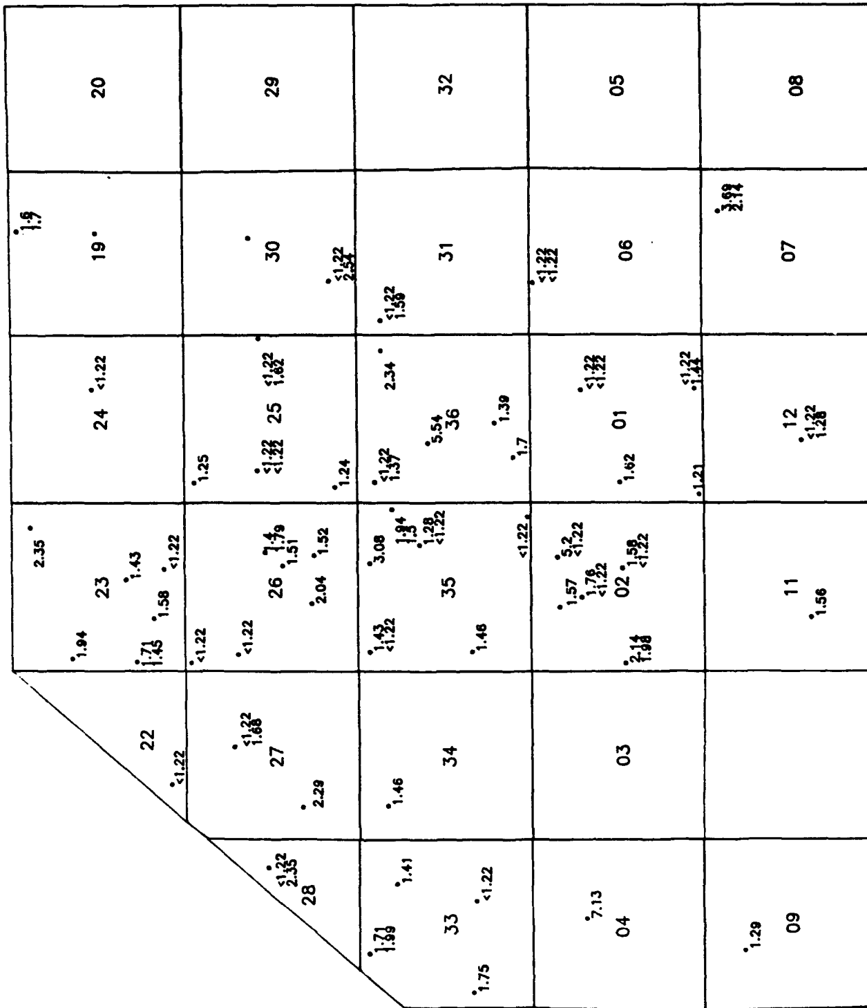
Figure C-146 FLUORIDE CONCENTRATIONS (mg/l) TASK 4, 3rd QUARTER DENVER AQUIFER SOURCE: ESE, 1987
