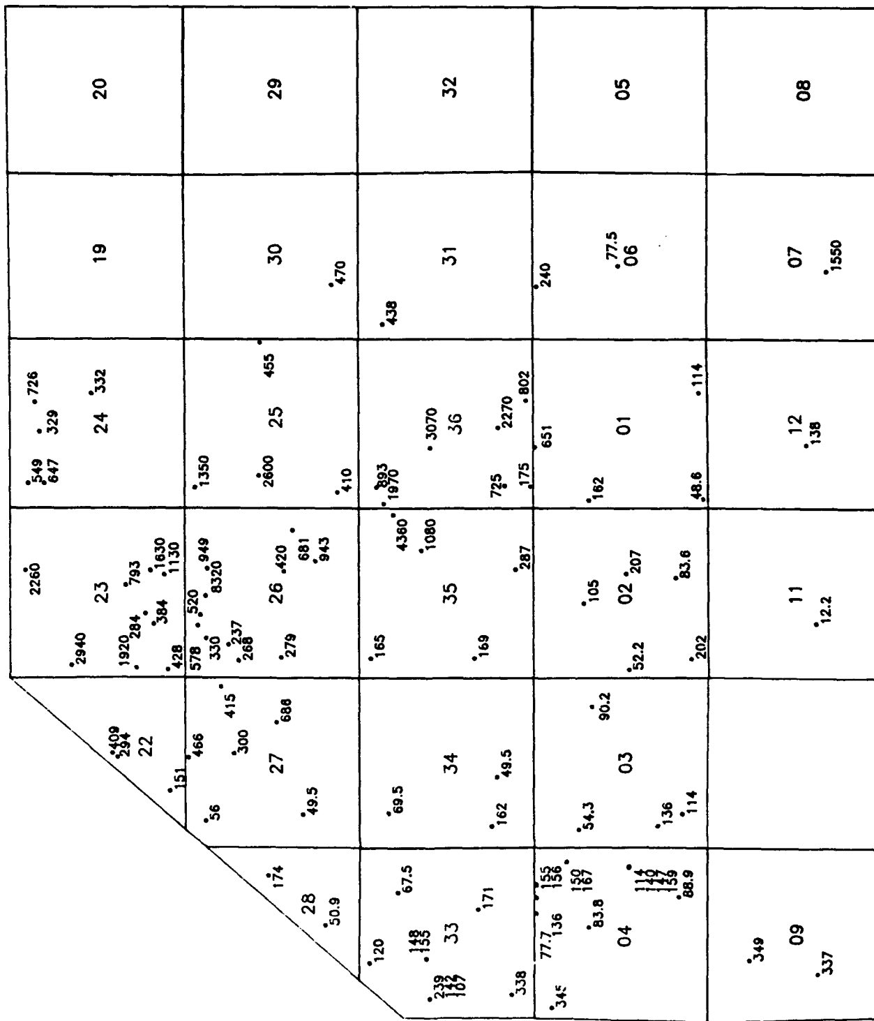
Figure C-151 SULFATE CONCENTRATIONS (mg/l) TASK 4, 4th QUARTER ALLUVIAL AQUIFER
