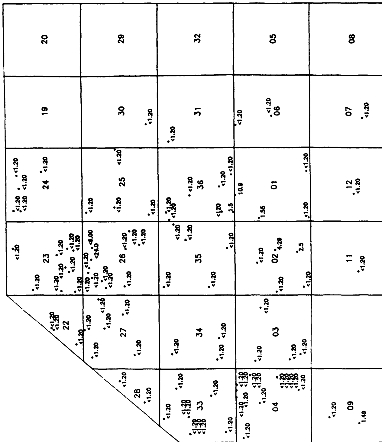
Figure C-103 11D/CLE CONCENTRATIONS (ug/l) TASK 4, 4th QUARTER ALLUVIAL AQUIFER SOURCE: ESE, 1987
