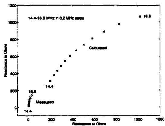
Fig. 4. Measured and NEC-computed impedances.
