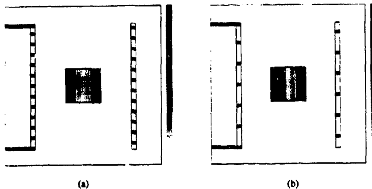
Fig. 7. FDTD results illustrating the fact that changing the coil pitch from 2" to 4" helped improve the uniformity of heating. Results are shown at 2 MHz. (a) Results for 2" pitch; (b) results for 4" pitch.
