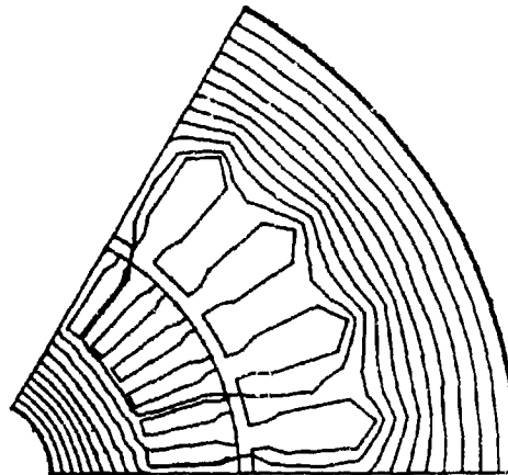
Figure 3. One-third pole (60°) model of Figure 1, showing computed instantaneous fluxlines.
