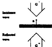
Figure 3: Incidence and reflected waves at a p.e.c. surface
