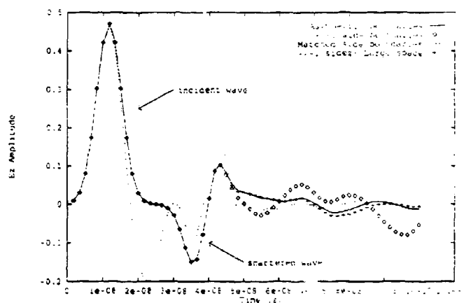
Figure 3: Comparison of Gaussian pulse plane wave in the different meshes with scattering object.
