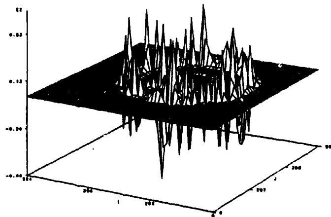
Figure 4a: Actual computed data for total field due to cylindrical pulse, t = 250 .
