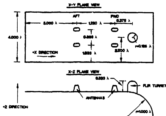
Figure 2. 1/4 Scale Model
