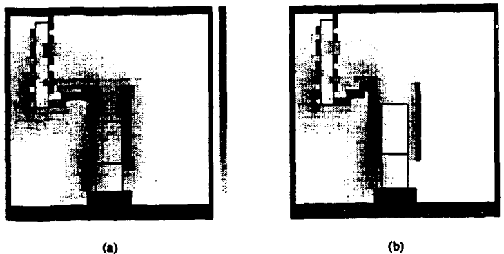
Fig. 4. Field distribution around the electrodes and the stubs (coils) for two different separation distances. Stubs are often used to improve field distribution along electrodes. (a) Electrode separation 12"; (b) electrode separation 15".
