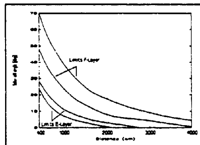
Figure 6. Composite of expected take-off angles for single hop ionospheric propagation predicted using HFMUFES4 - all frequencies, times of day, seasons and solar activity.
