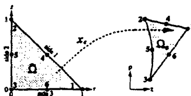
Figure 2. The map x_e from the master element \tilde{\Omega} to the e th element \Omega_e is quadratic in the local coordinates r and s . The map is defined by coordinates (z, \rho) of six nodes.
