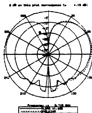
Figure 3 Radiation pattern of a monopole on a sphere radius 1.5915\lambda compared with Byelkina [8].
