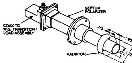
Figure 1: The GE baseline design of the Mars Observer low gain antenna showing the feed portion as a choked circular waveguide
