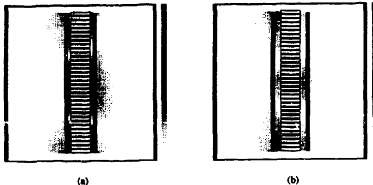
Fig. 3. Field distribution along the axis of the dryer for two separation distances between the electrodes. Dielectric properties were varied from \epsilon' = 25 , \sigma = 0.04 (wet ware) to \epsilon' = 5 , \sigma = 0.00 (dry ware) along the dryer. (a) Electrode separation 12"; (b) electrode separation 15".
