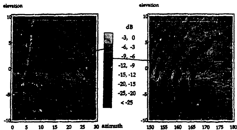
Fig. 8 Combined coverage pattern for the three antennas at positions A1, A5, and A9 (fig. 1) analysed with NEW-AIR at UHF-band Azimuth 0^\circ , elevation 0^\circ corresponds to the forward direction.
