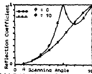
Fig(4-b) Reflection Coefficient V.S. Scan Angles
