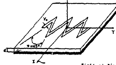
Fig(6-a) Zigzag of total length 1.29\lambda_n
