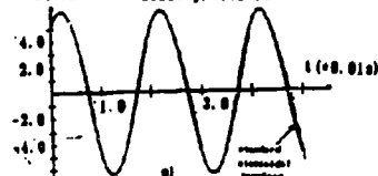
Fig. 13 Waveform of magnetic flux densities inside steel plate at prescribed positions Note: Fig. 13-(a, b, c) show the waveforms of magnetic flux densities inside steel plate which were measured by the "interlinked-coil". Positions P7, P8, P9, see Fig. 13-(a, b).
