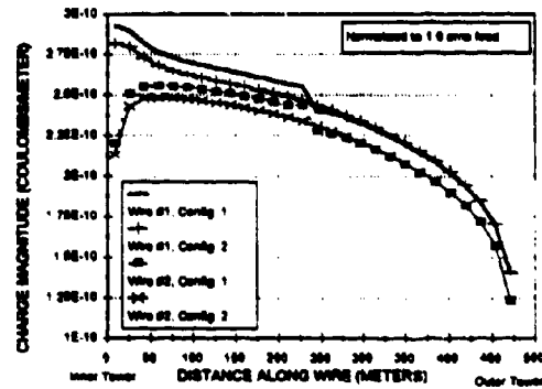
Figure 4. Calculated charge density for top-hat wires 1 and 2 at 17.5 kHz.
