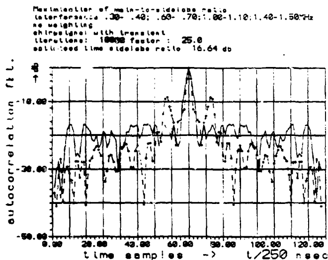
Fig. 6 a Autocorrelation function of shaped signal after 10000 iterations \delta = 25 .
