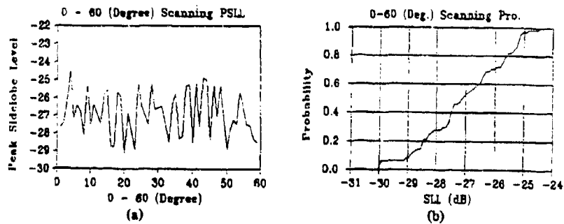
Fig.1 For rounding to the nearest bits, (a) PSL distribution in region 0^{\circ} \sim 60^{\circ} , (b) probability curve of PSL
