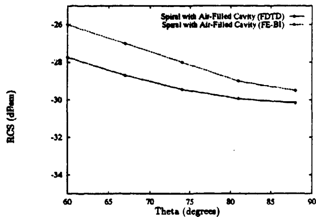
Figure 4: FDTD and FE-BI RCS versus Incidence Angle for square spiral antenna with air-filled cavity backing in \phi = 45 plane at 4.5 GHz. The incident plane wave was a \theta -polarized, modulated Gaussian pulse.
