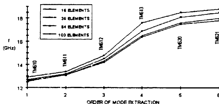
Figure 1. Convergence curves of the finite element frequencies for the first six modes of the hollow cavity with r_c = 6 .
