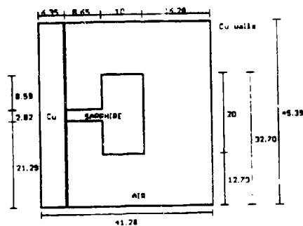
Figure 5. Dimensions (in mm) of sapphire resonator.
