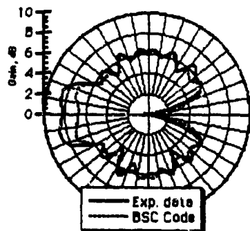
Fig. 11 Horizontally polarized Loop-fed Slot, at f_c with large plate scatterer
