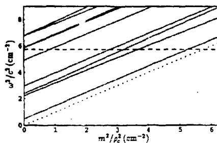
Figure 9. Dispersion diagram of a curved guide with radius of curvature \rho_c . The dashed line is the drive frequency, and the dotted line corresponds to the speed of light along the center of the guide.
