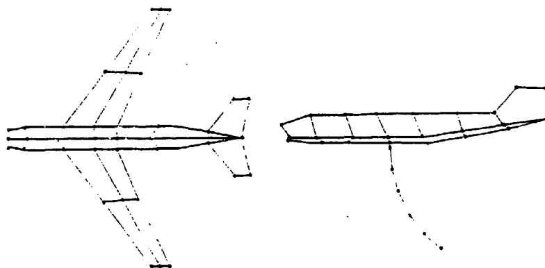
Fig. 3. Top and profile views of wire-grid model used in NEC-2 analysis.
