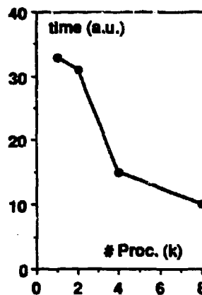
Fig. 2: Execution time of fully parallelized loop for interior grid points on various machine sizes. Time is measured in arbitrary units, the number of processors is in multiples of 1,024.
