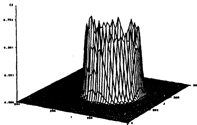
Figure 3b: Smoothed data at t = 150 .
