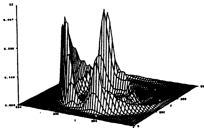
Figure 5b: Smoothed data at t = 400 .
