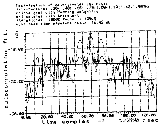
Fig.11 Autocorrelation function of Hamming weighted chirp after 10000 iterations \delta = 100 .
