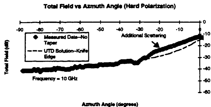
Figure 5. Comparison of UTD and Measured Results From the Knife Edge, showing additional scattering when the observation was less than 30^\circ into the shadowed region.
