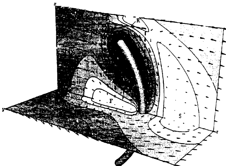
Figure 2 The banana shaped object (ideal conductor in air, half a wavelength ( \lambda ) long and 0.027\lambda thick, bent along a quarter of a full circle) is illuminated by an x -polarized plane wave traveling in x -direction. The picture shows the time mean value of the Poynting vector of the total near field. There is a shadow region S with low field values and a 'standing wave area' F where the fields are high but only the time mean value of the power flux is low. See also fig. 4 for more details of the field in the rectangle R .
