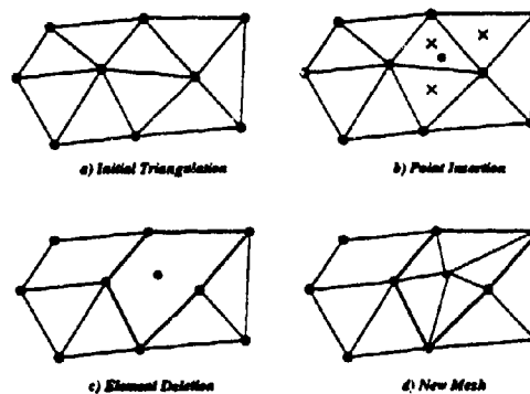
Figure 2: Watson's algorithm
