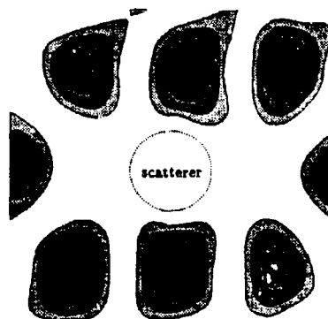
Figure 8 The scatterer is illuminated from left (TM-case). The plot shows the (wrong!) instantaneous value of the total electromagnetic field energy obtained by MEI with a poor set of multipoles. Note that the patches are traveling from right to left, just as the multipoles. Here \lambda/d = 30 , diameter of the scattering cylinder: \lambda/2 .
