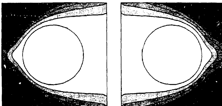
Figure 9 The use of different multipoles for the same scattering problem gives very different results. Both pictures show the time mean value of the total Poynting field. Outgoing multipoles as multipoles yield a correct solution (left) while ingoing multipoles as multipoles yield a totally wrong power flux looking as if it came from the opposite side than the incident field but the power flux is from left to right in both cases. Here \lambda/d = 30 , diameter of the scattering cylinder: \lambda/2 .
