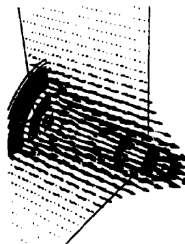
Figure 11: Poynting vector
