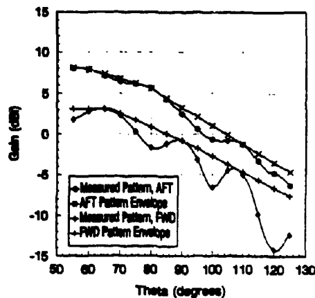
Figure 3. Antenna Patterns Measured on 1/4 Scale Model
