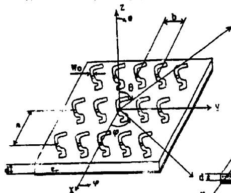
Fig.(1) Geometry of the infinite array of arbitrary shape printed antenna
