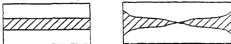
Figure 2: a) Conventional resonator b) Resonator shaped for maximum Q
