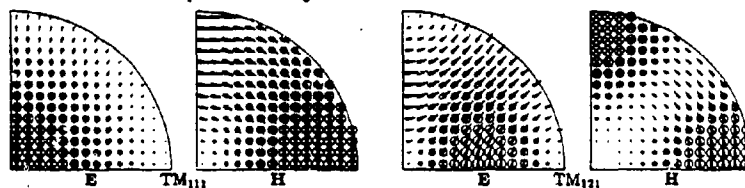
Figure 6. Field plots of the two lowest m = 1 modes of a sphere based on the 256 element mesh in figure 4. The triangles represent the magnitude and direction of the fields E_s and H_s . The size of the circles represent the magnitude of the (imaginary) fields E_s and H_s . A crossed circle indicates the field is negative.
