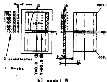
Fig. 4 Specified positions for magnetic flux densities
