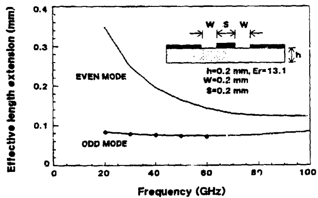
Figure 5: Effective length extension of a CPW short-end. — unified full-wave method, • Dib & Katehi [11]
