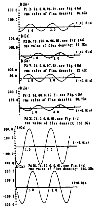
Fig. 12 Waveform of magnetic flux densities at prescribed positions, Date: Points P1-P6, see Fig. 4
