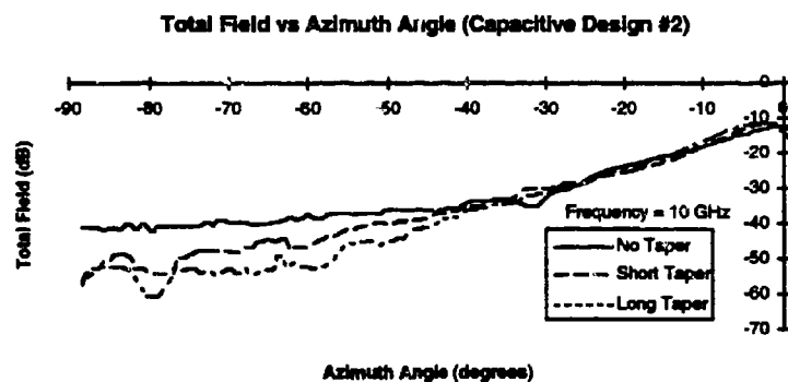
Figure 6. Azimuth Cut of Capacitive Design at 10 GHz, showing improvement more than 30^\circ into the shadow region.
