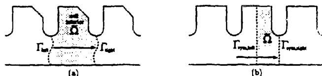
Figure 1. The shaded region \tilde{\Omega} (a) is one cell of a periodic structure. The dashed lines are periodic boundaries. The arrow shows the rigid motion \hat{R} translating a point from the boundary \Gamma_{left} to the boundary \Gamma_{right} . The shaded region \tilde{\Omega} (b) represents one half-cell of a symmetric periodic structure. The dashed lines are symmetry planes.
