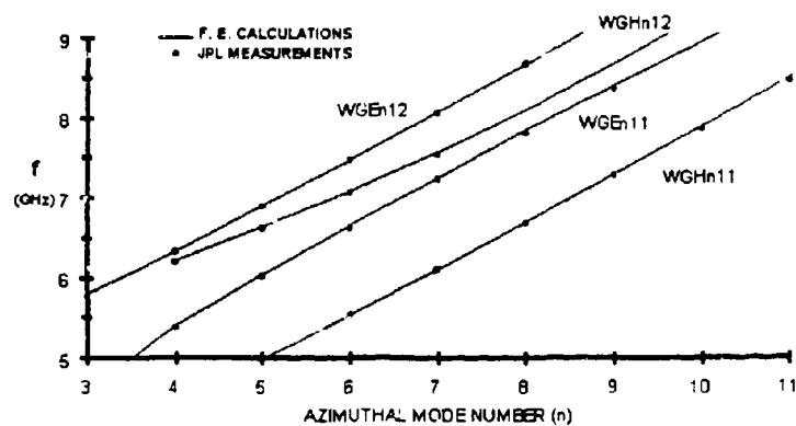
Figure 7. Comparison of resonant frequencies obtained from finite element analyses with measurements made on a cylindrical sapphire resonator.
