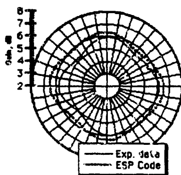
Fig. 14 Loop-fed Slot, 1.0 f_c on 9 wavelength dia. ground alone, 60° azimuth pattern
