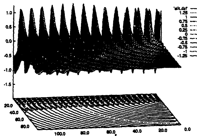
Figure 6: Near field electric field diffracted through a slit
