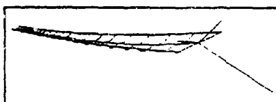
Figure 4. Schematic illustrating sag for horizontally deployed LPDA. All wires, catenaries and staywires are shown.
