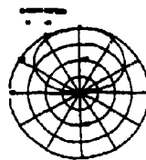
Figure 6 E-plane pattern at 1.2 GHz
