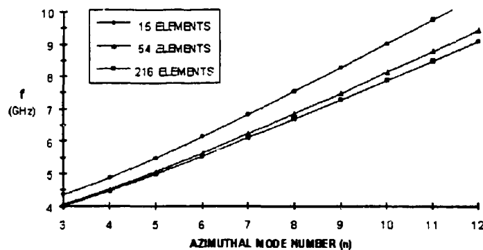
Figure 6. Convergence curves of the finite element frequency for the fundamental WGH_{n,1} family in the sapphire resonator using different mesh sizes.
