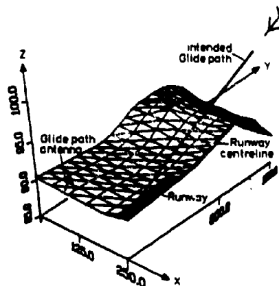
Figure 7: Modelling of 3D-terrain by triangles for UTD optimization of ILS-glidepath
