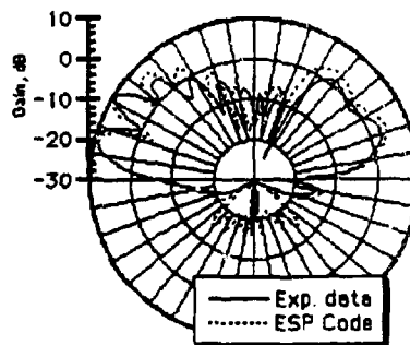
Fig. 21 Horizontally polarized Loop-fed Slot, 1.13 f_c with large plate scatterer, elevation pattern
