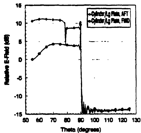
Figure 7. NEC-BSC X-Z Plane Pattern for Large Plate/Cylinder Model
