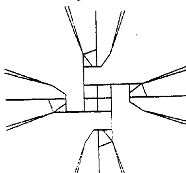
Fig. 3. Closeup Top View Showing NEC Model Tower Crosssection and Feed Region.
