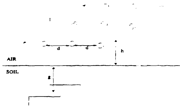
Figure 1: Geometry for a balanced bridge mine detection system as it appears in the TLM mesh.
