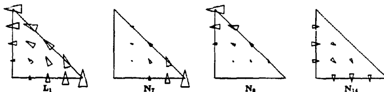
Figure 3. Examples of local basis functions: L_1 is a vector field normal to sides 2 and 3. This field could be a basis function for a linear edge element. N_7 , N_8 and N_{14} are quadratic basis functions for the vector field E_1 constructed from L_1 . N_7 and N_8 have non-zero tangential field on side 1. The size and direction of the triangles indicate the magnitude and direction of the vector basis function.
