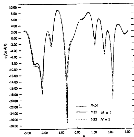
Fig.3 RCS of a elliptic dielectric cylinder
