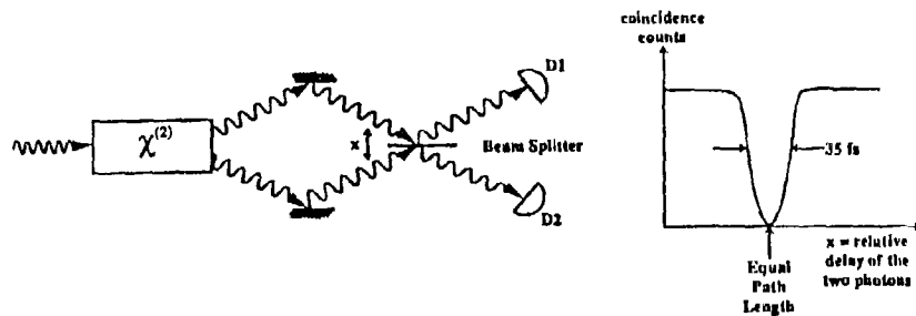
Figure 10. Hong-Ou-Mandel interferometer
