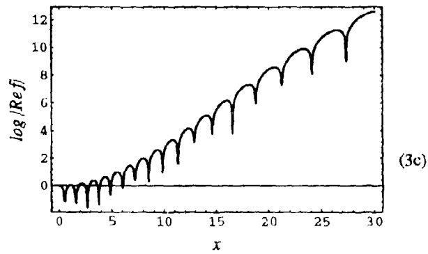
Figure 3. Computations of f(x, 2, 0.2) for the truncated integral, Eq.(11), showing (a), superoscillations, and (b) conventional oscillations. Circles: exact expression, Eq.(12); full lines: saddle-point approximation, Eq.(16). In (c) the logarithms are base 10
