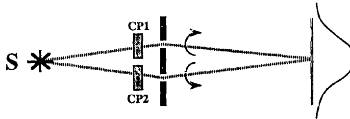
Figure 8. Young's two-slit experiment with circular polarizers CP1 & CP2
