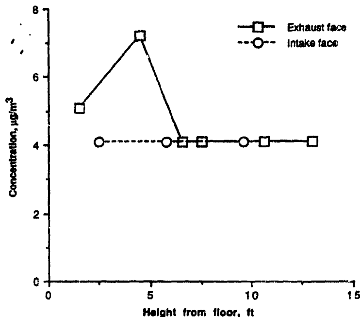
Figure 48. Concentrations of HDI Measured at the Intake and Exhaust Faces—Test 4.
