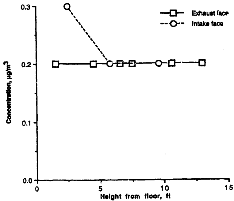
Figure 39. Concentrations of Lead at the Intake and Exhaust Faces—Test 5.
