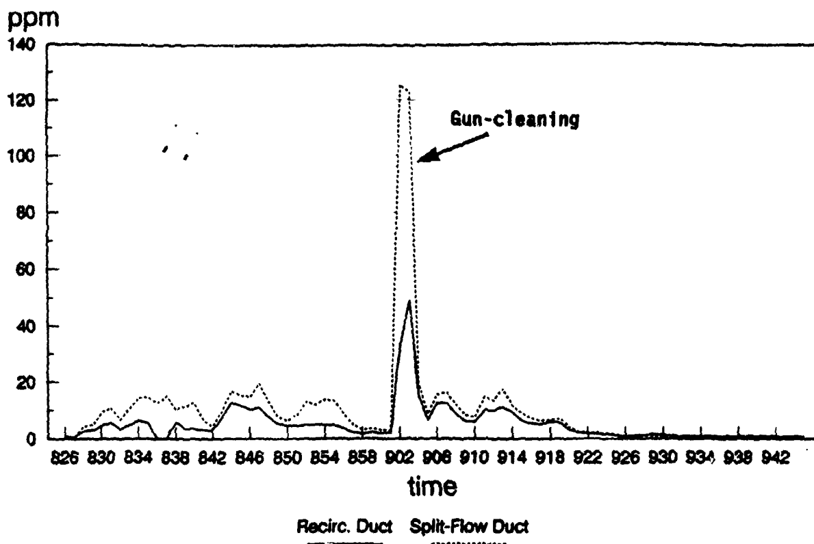
Figure 49. Representative Results from Continuous Emission Monitoring by EPA Method 25A—Topcoat Painting.
