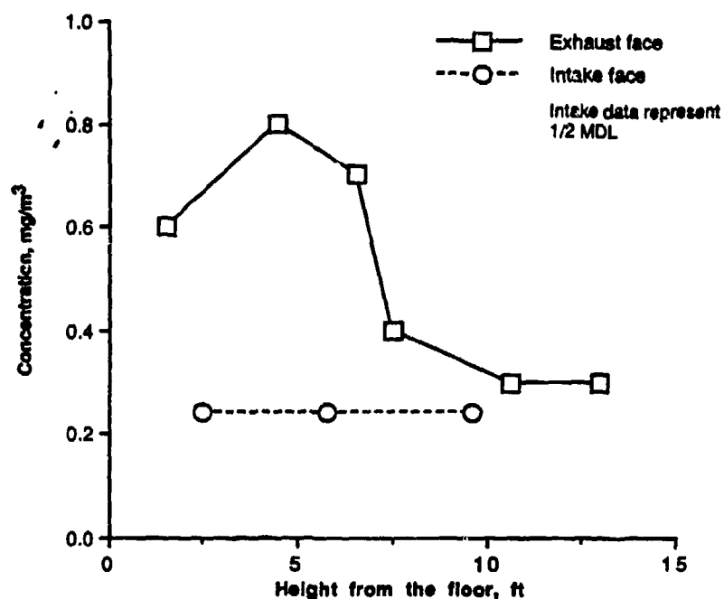
Figure 27. Measured Concentrations of Particulate at the Intake and Exhaust Faces During Split-flow/Recirculating Ventilation—Test 5.
