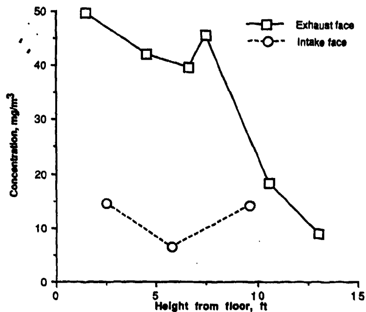
Figure 18. Results of Organic Measurements at the Intake and Exhaust Faces During Split-flow/Recirculating Ventilation—Test 3.
