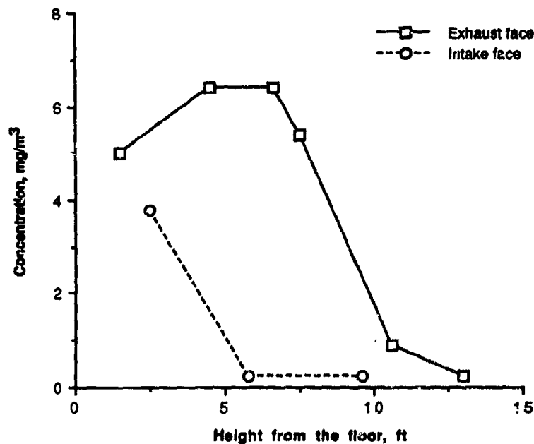
Figure 24. Measured Concentrations of Particulate at the Intake and Exhaust Faces During Split-flow/Recirculating Ventilation—Test 2.
