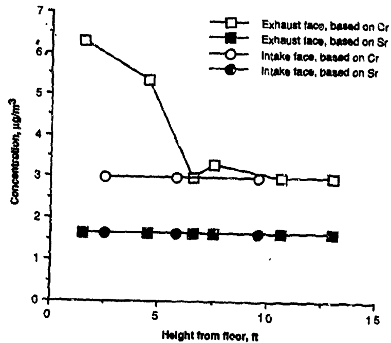
Figure 34. Concentrations of Strontium Chromate Measured at the Intake and Exhaust Faces—Test 5.
