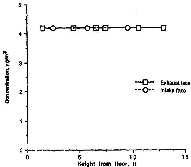
Figure 45. Concentrations of HDI Measured at the Intake and Exhaust Faces—Test 1.
