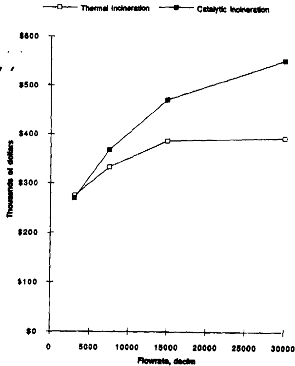
Figure 52. Capital Costs for Incineration as a Function of Exhaust Flow Rate.
