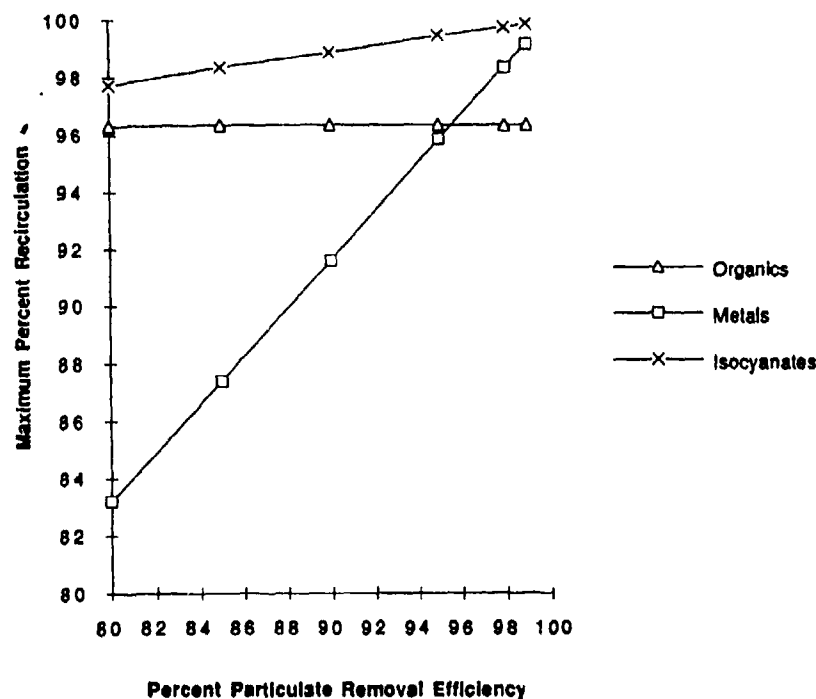
Figure 55. Dependence of Maximum Projected Recirculation on Percent Particulate Removal Efficiency — Recirculating Ventilation.
