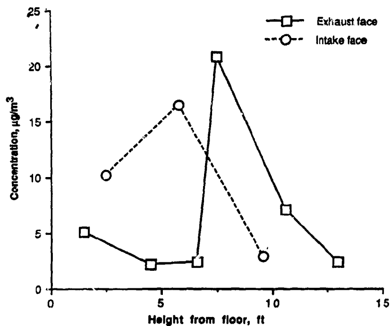
Figure 44. Concentrations of Zinc at the Intake and Exhaust Faces—Test 5.
