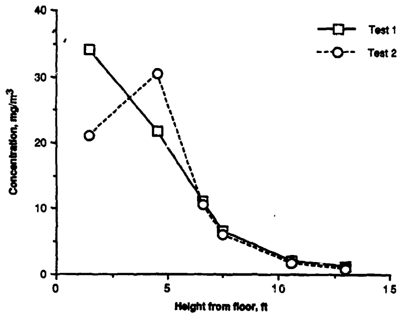
Figure 8. Results of Organic Measurements at the Exhaust Face During Baseline Testing.
