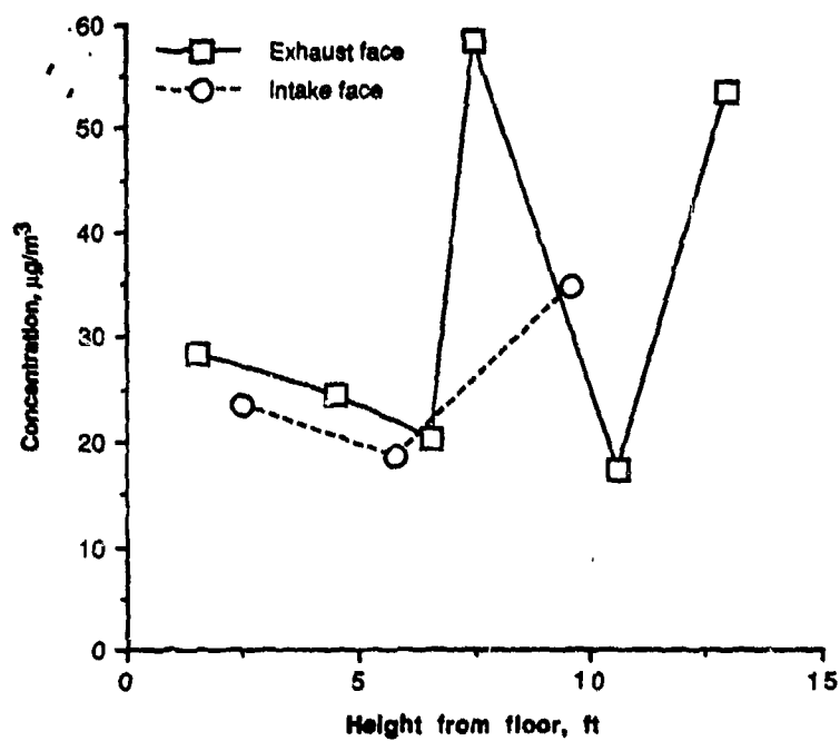
Figure 42. Concentrations of Zinc at the Intake and Exhaust Faces—Test 3.
