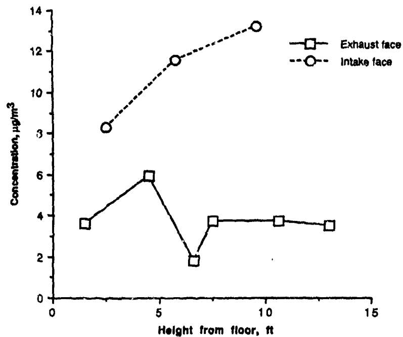
Figure 43. Concentrations of Zinc at the Intake and Exhaust Faces—Test 4.
