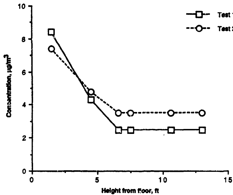
Figure 11. Baseline HDI Concentrations Measured at the Exhaust Face.
