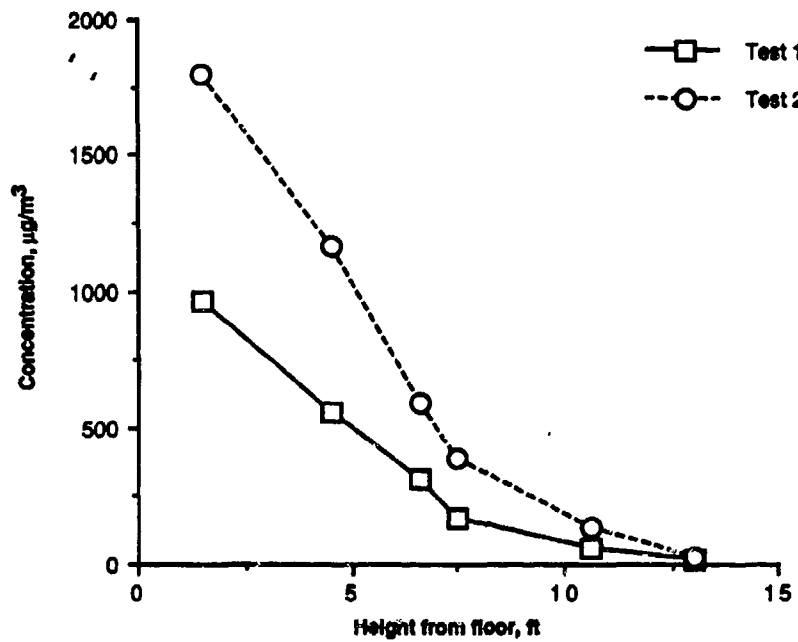
Figure 10. Concentrations of Strontium Chromate Measured at the Exhaust Face.
