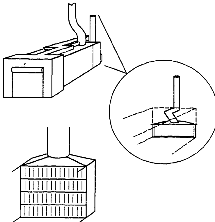
Figure 5. Schematic Diagram of Modified Paint Spray Booth 2.
