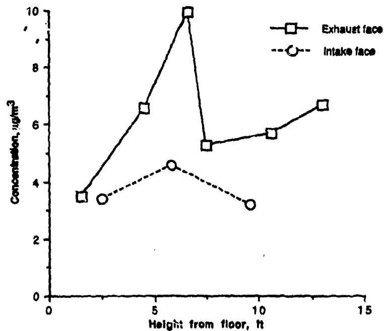
Figure 40. Concentrations of Zinc at the Intake and Exhaust Faces—Test 1.
