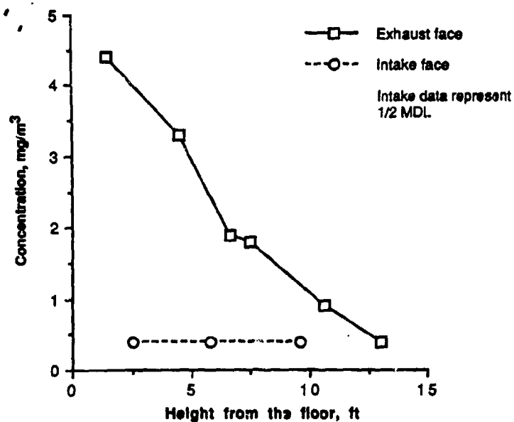
Figure 23. Measured Concentrations of Particulate at the Intake and Exhaust Faces During Split-flow/Recirculating Ventilation—Test 1.
