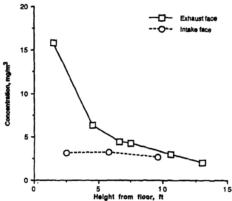
Figure 19. Results of Organic Measurements at the Intake and Exhaust Faces During Split-flow/Recirculating Ventilation—Test 4.
