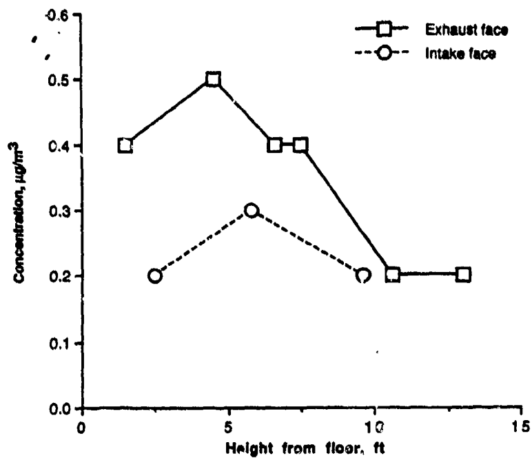
Figure 38. Concentrations of Lead at the Intake and Exhaust Faces—Test 4.
