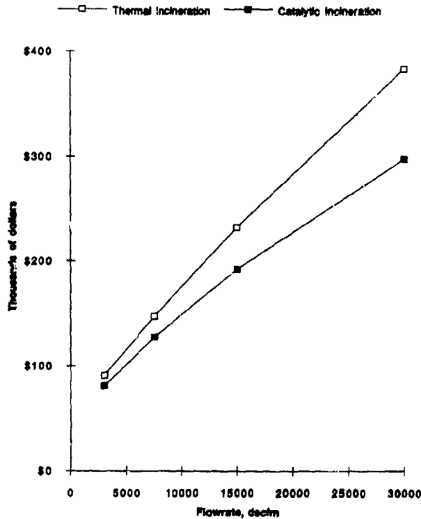
Figure 53. Annual Operating Costs for Incineration as a Function of Exhaust Flow Rate.
