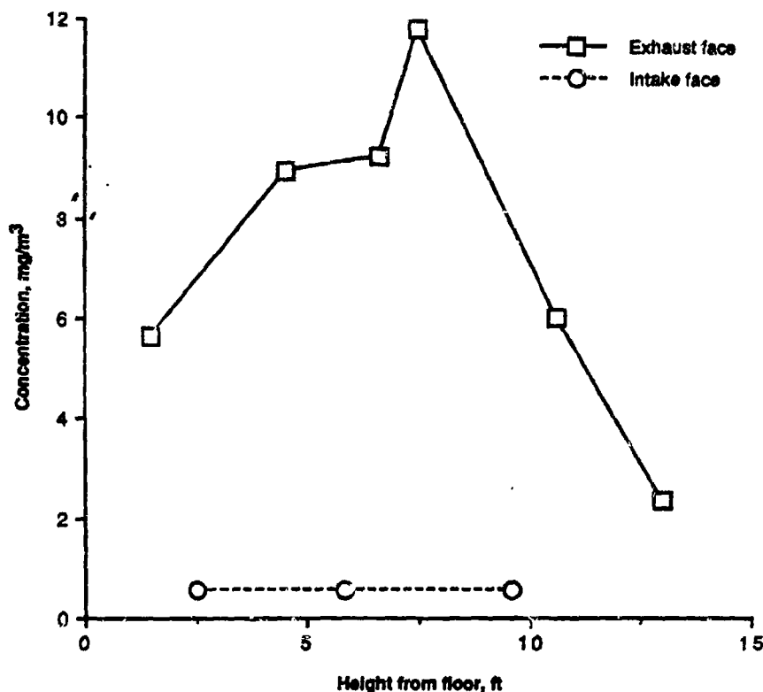
Figure 22. Results of Organic Measurements at the Intake and Exhaust Faces During Split-flow Ventilation—Test 1.
