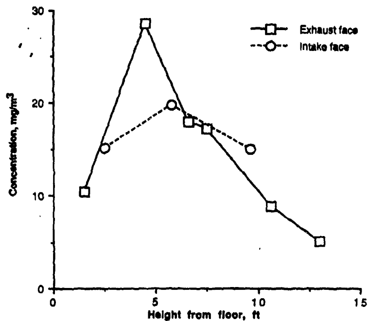
Figure 16. Results of Organic Measurements at the Intake and Exhaust Faces During Split-flow/Recirculating Ventilation—Test 1.
