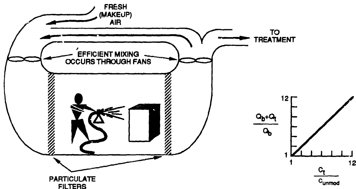
Figure 2. Schematic Diagram of a Paint Spray Booth Recirculating Ventilation System.
