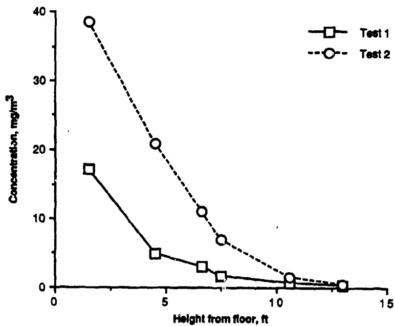
Figure 9. Measured Concentrations of Particulate at the Exhaust Face During Baseline Testing.
