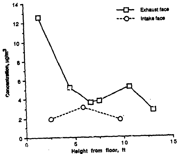
Figure 41. Concentrations of Zinc at the Intake and Exhaust Faces—Test 2.
