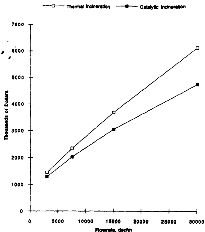
Figure 54. Total Emission Control Costs for Incineration Over 10 Years.
