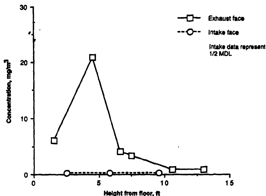
Figure 29. Measured Concentrations of Particulate at the Intake and Exhaust Faces During Split-flow Ventilation—Test 2.
