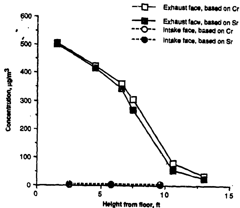
Figure 32. Concentrations of Strontium Chromate Measured at the Intake and Exhaust Faces—Test 3.
