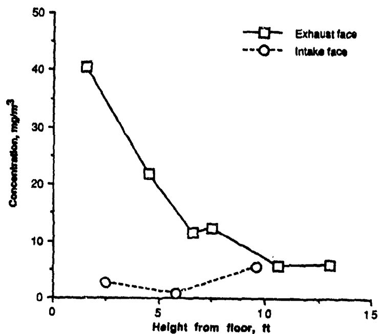
Figure 17. Results of Organic Measurements at the Intake and Exhaust Faces During Split-flow/Recirculating Ventilation—Test 2.
