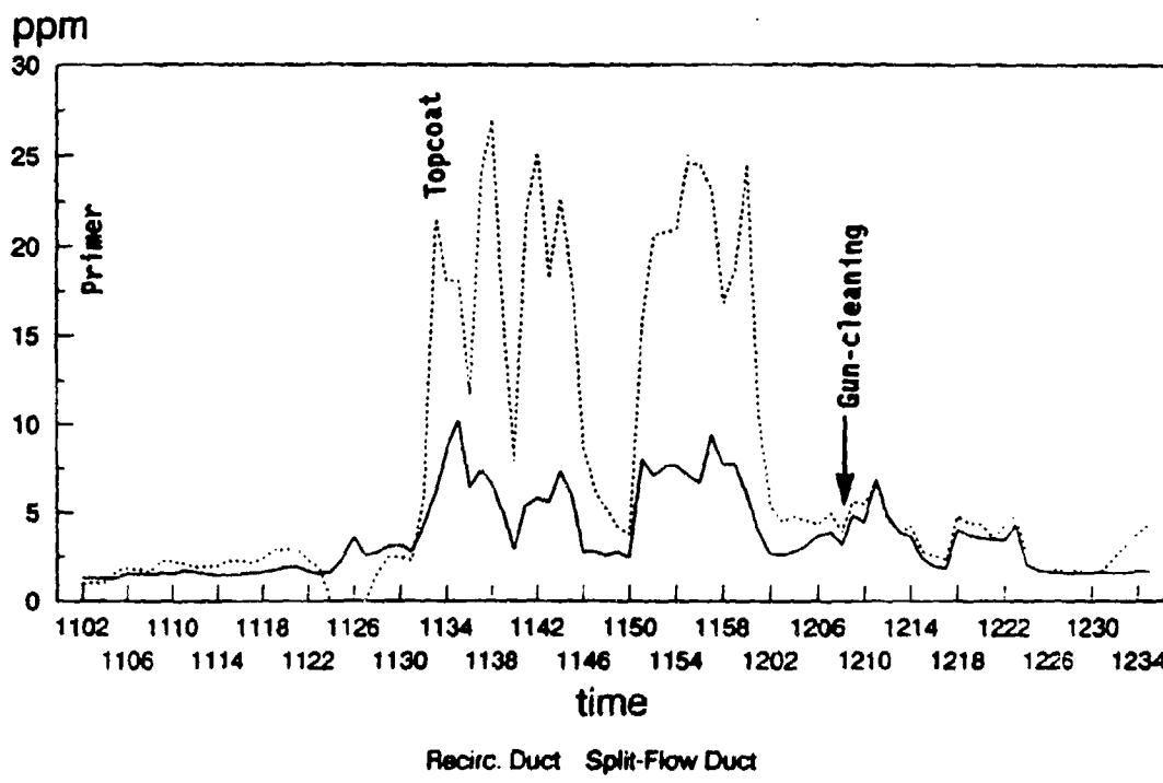
Figure 51. Representative Results from Continuous Emission Monitoring by EPA Method 25A—Split-flow Test.
