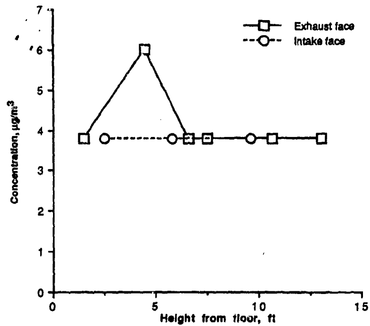
Figure 46. Concentrations of HDI Measured at the Intake and Exhaust Faces—Test 2.
