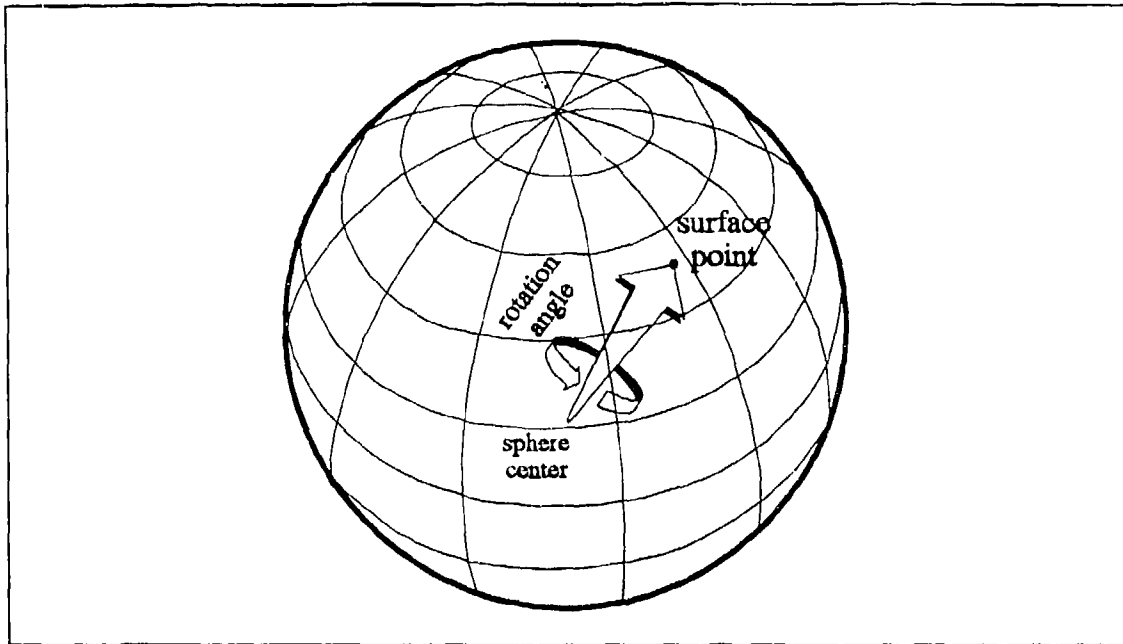
Figure 6.6. Quaternion representation.
