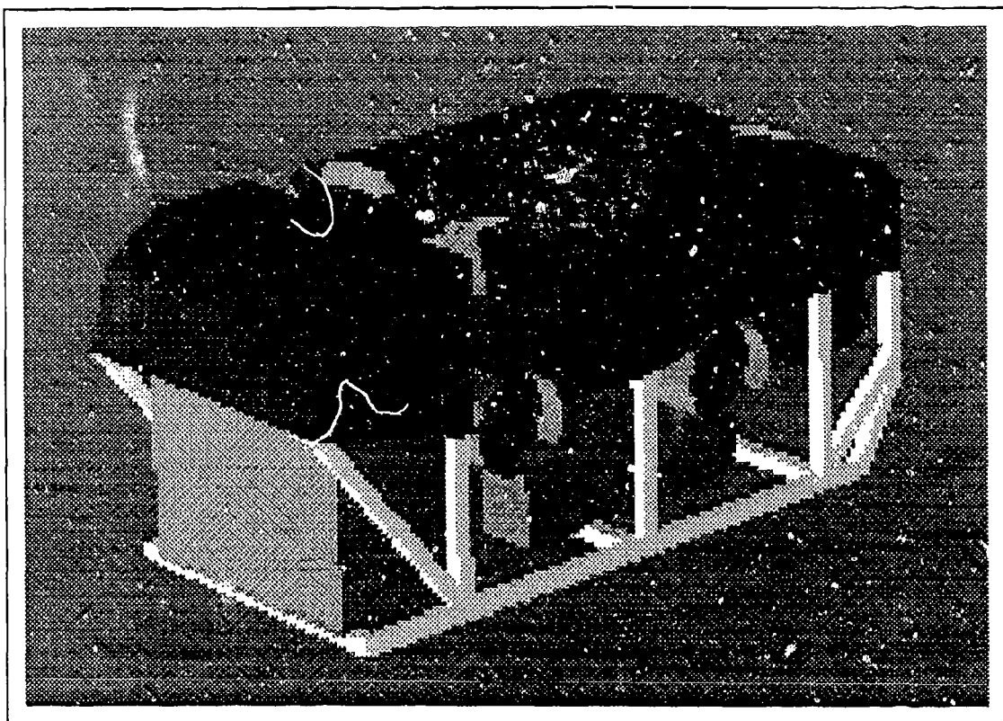
Figure 5.2. Open Inventor rendering of JASON ROV graphics model.
