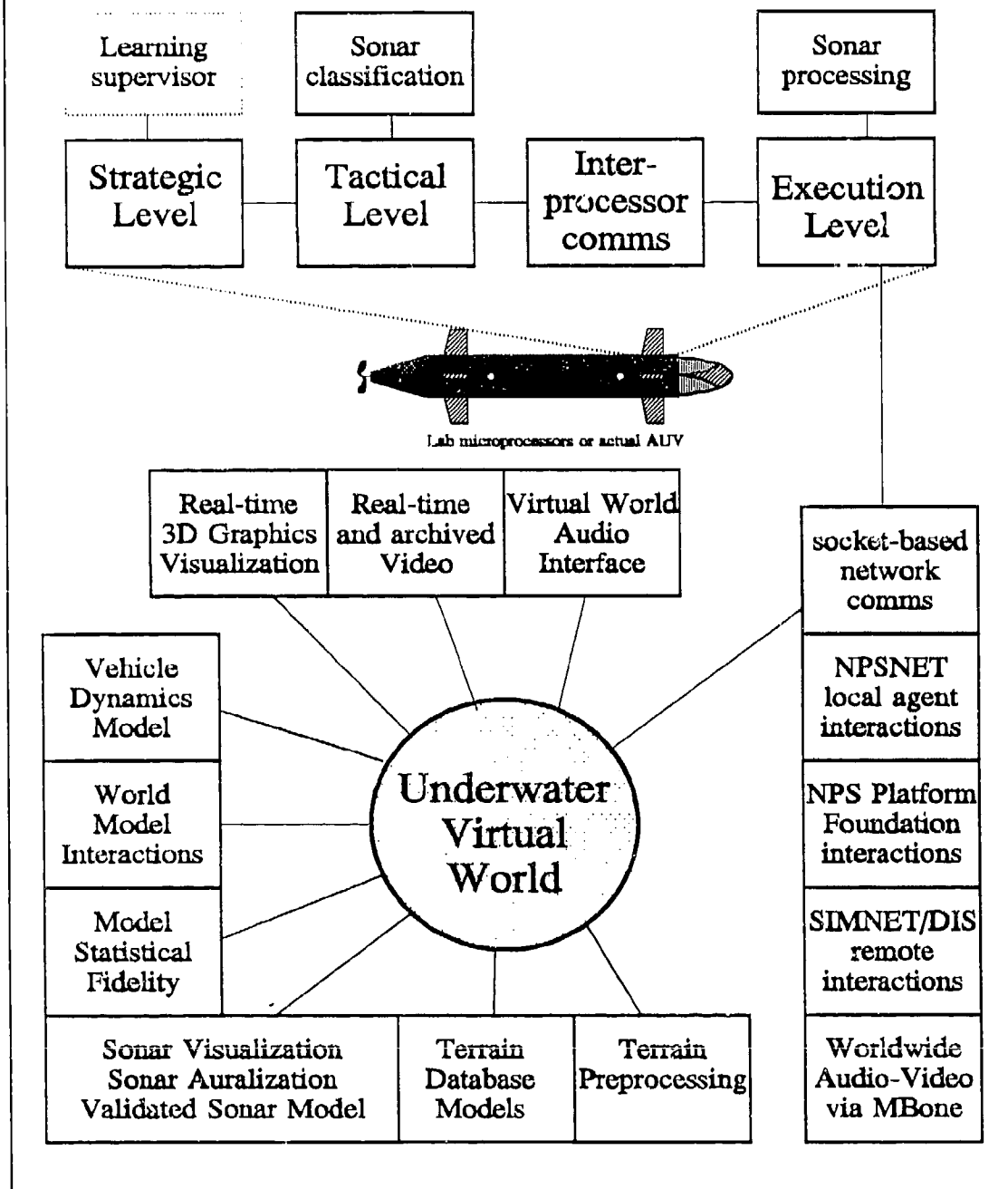
Figure 3.1. NPS AUV underwater virtual world software architecture.
