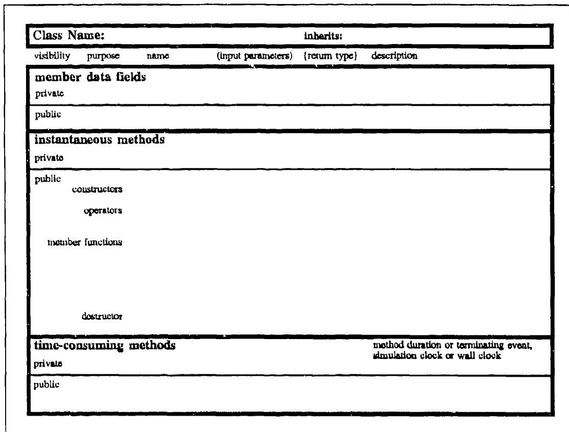
Figure 6.8. OOSPIC class diagram template for C++ class definitions. Separation of class name, data fields, instantaneous methods and time-consuming methods clarifies class functionality and design.
