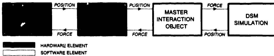
Figure 5-8: Power flow between two-port elements in IDMS.
