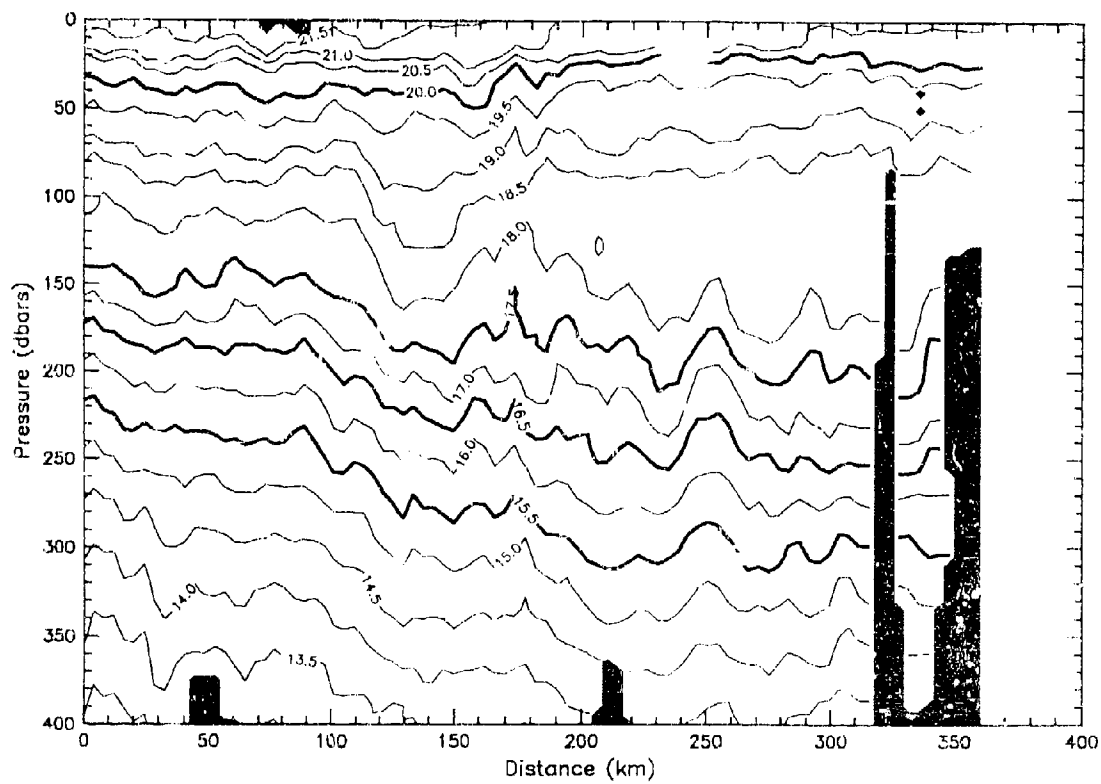
Theta - Sub 4, Transect 5 - S - N
