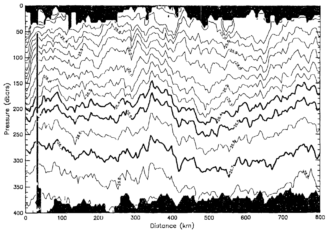
Sigma Theta - Sub 4, Transect 1 - SE - NW
