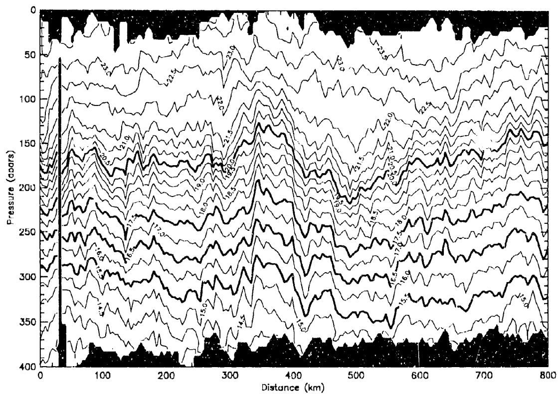
Theta - Sub 4, Transect 1 -- SE - NW
