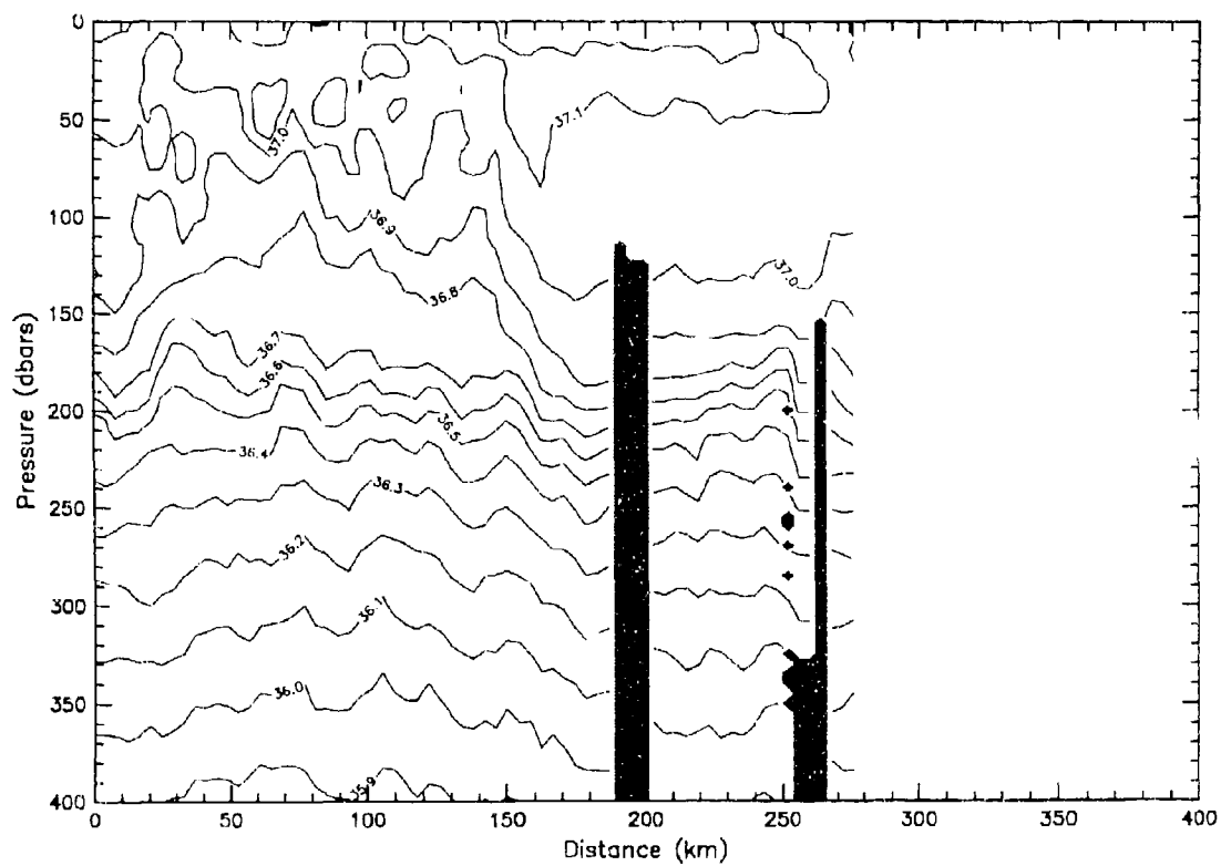
Salinity - Sub 4, Transect 3 - E - W
