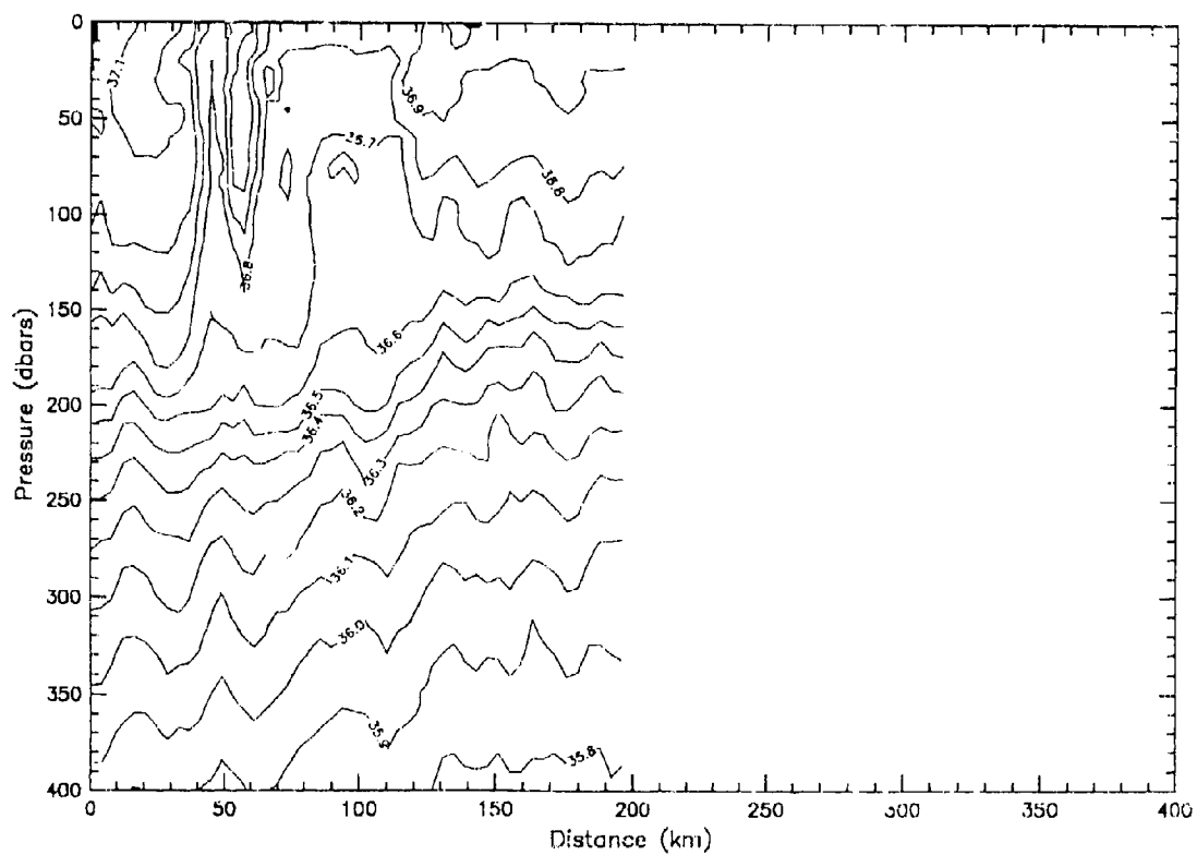
Salinity - Sub 4, Transect 4 - S - N
