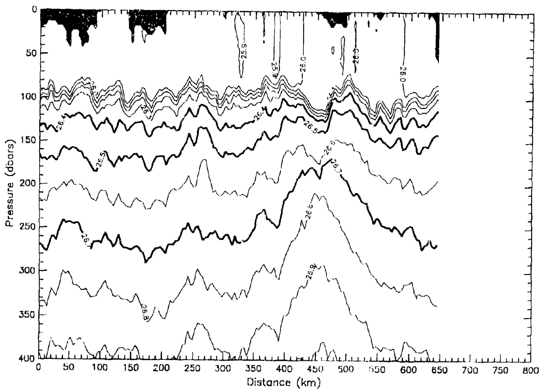
Sigma Theta - Sub 3, Transect 2 -- S -- N
