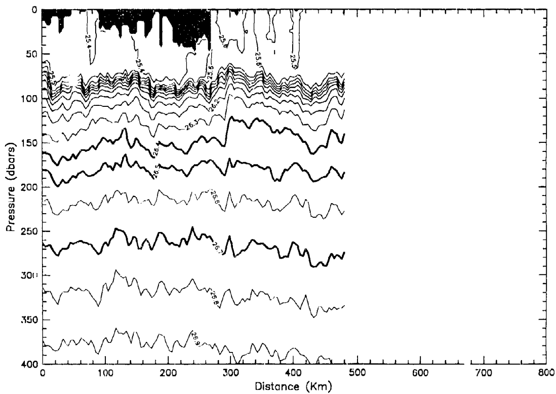
Sigma Theta — Sub 3, Transect 1 — SW — NE
