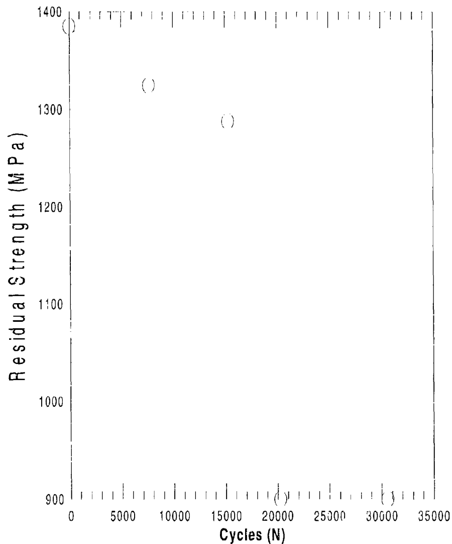
Figure 13. Residual Strength & Cycles Relationship for [0]_E Laminate at 427^\circ\text{C} , R=0.05 , \sigma_{\text{max}}=900 MPa, f=10 Hz Conditions
