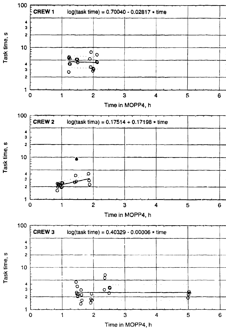
Figure C-75. Task times with regression lines for fire in MOPP4-S.
