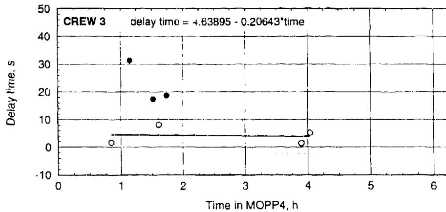
Figure C-11. Task times with regression lines for begin set deflection in MOPP4-R.
