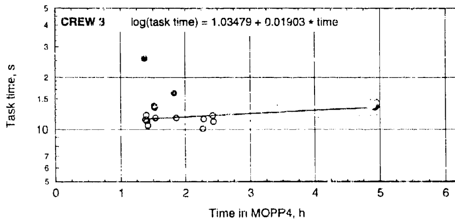
Figure C-111. Task times with regression lines for reload projo and pwdr in MOPP4-S.
