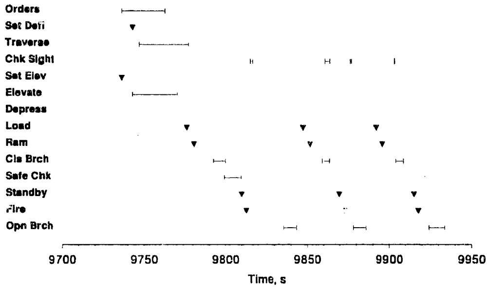
Figure A-21. Crew 2 timelines for fire missions 5 and 6 in MOPP4-R.
