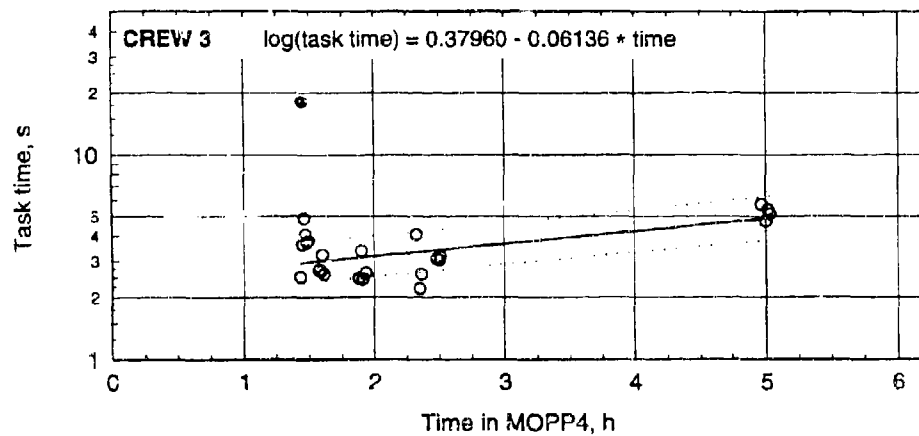
Figure C-51. Task times with regression lines for load projectile in MOPP4-S.
