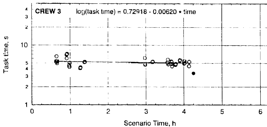
Figure C-85. Task times with regression lines for swab chamber in BDU.
