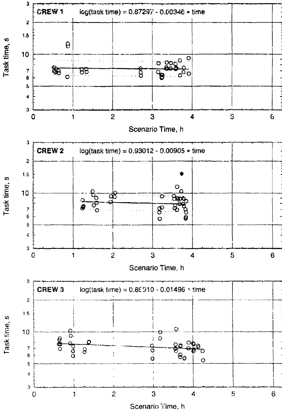
Figure C-109. Task times with regression lines for reload proj0 and pwdr in BDU.
