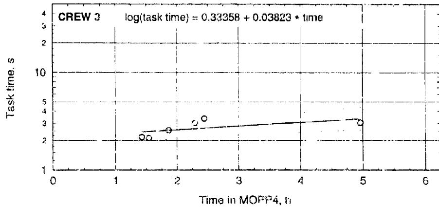
Figure C-117. Task times with regression lines for last open breach in MOPP4-S.
