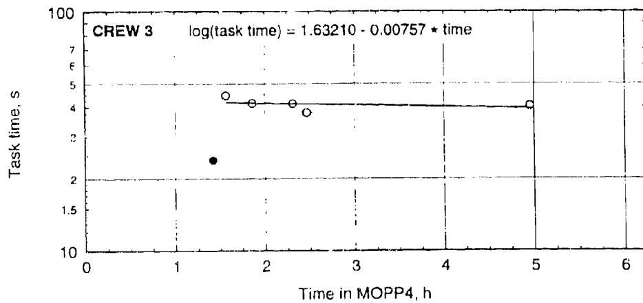
Figure C-3. Task times with regression lines for relay orders in MOPP4-S.
