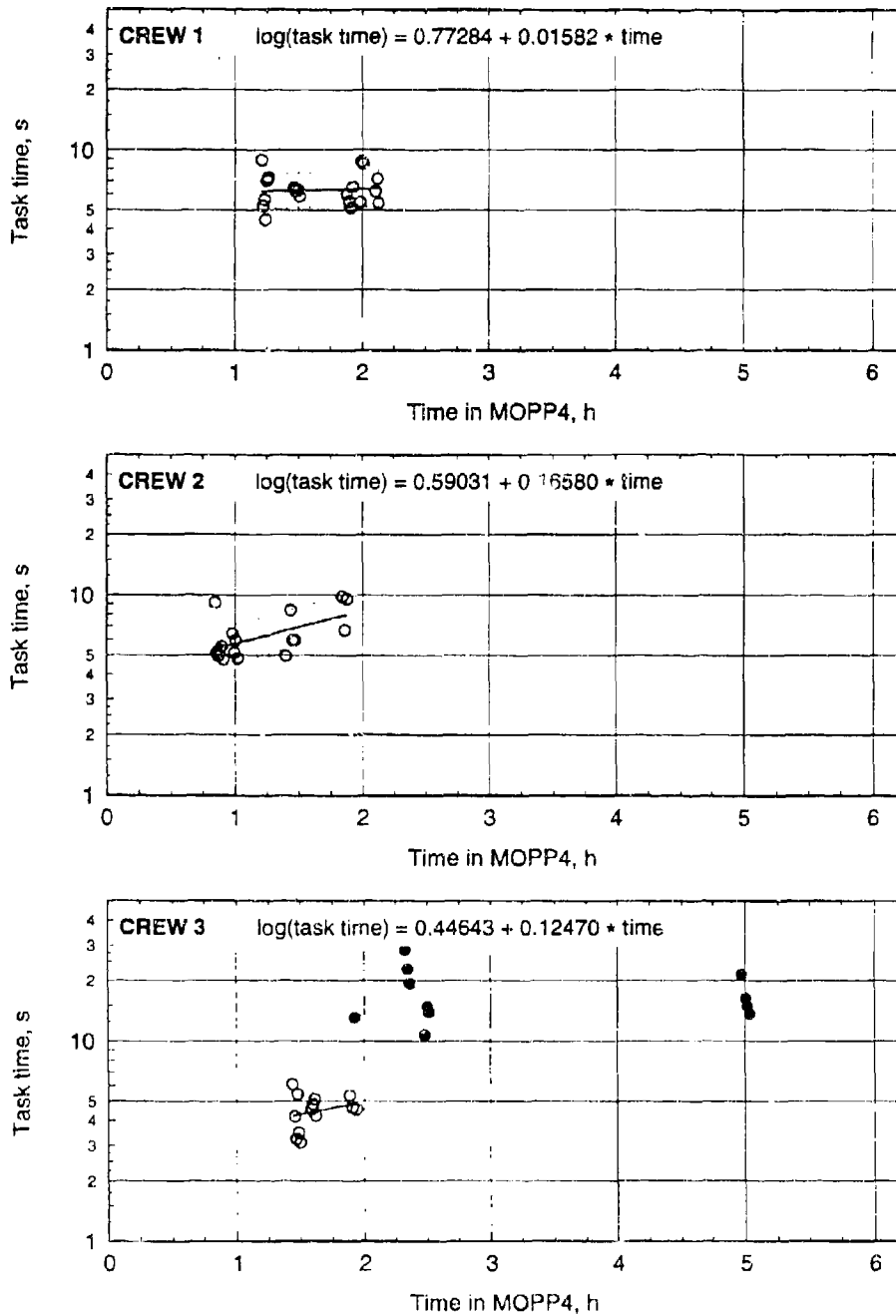
Figure C-69. Task times with regression lines for lock breach and prime in MOPP4-S.
