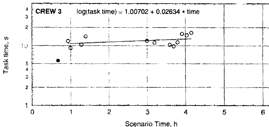
Figure C-121. Task times with regression lines for swab and inspect in BDU.
