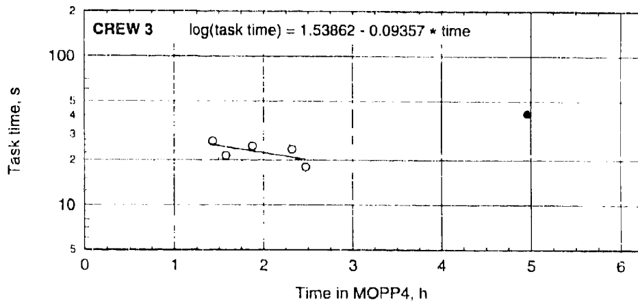
Figure C-21. Task times with regression lines for traverse tube in MOPP4-S.
