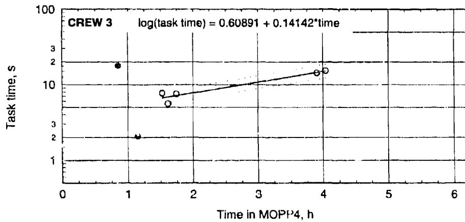
Figure C-35. Task times with regression lines for set elevation in MOPP4-R.
