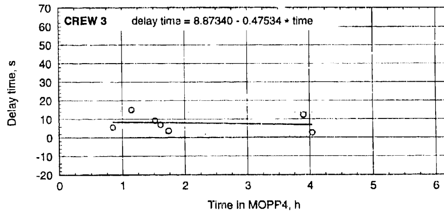
Figure C-29. Task times with regression lines for begin set elevation in MOPP4-R.
