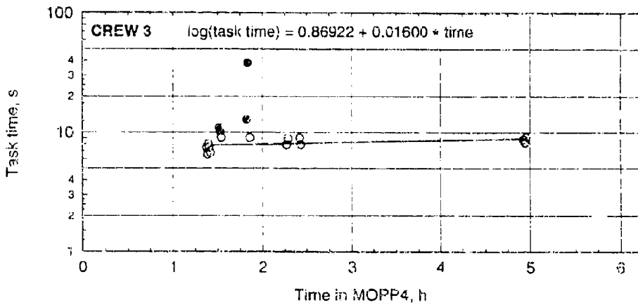
Figure C-105. Task times with regression lines for reload powder in MOPP4-S.
