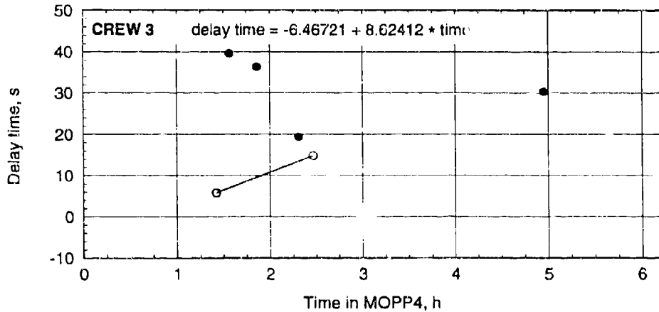
Figure C-9. Task times with regression lines for begin set deflection in MOPP4-S.
