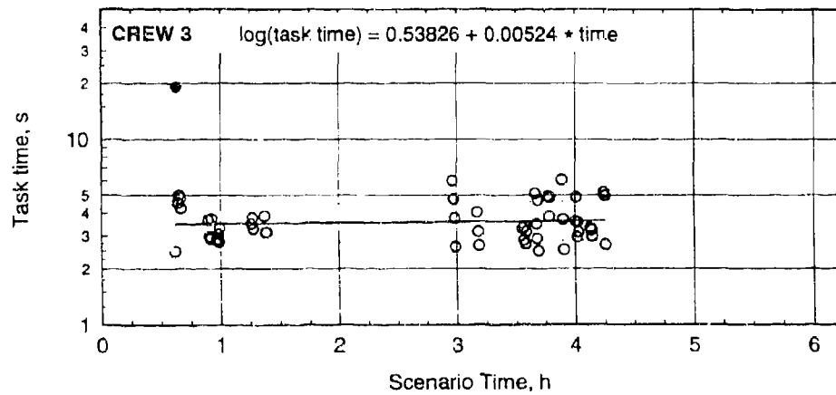
Figure C-67. Task times with regression lines for lock breach and prime in BDU.
