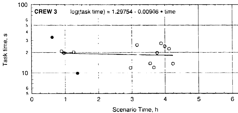
Figure C-19. Task times with regression lines for traverse tube in BDU.
