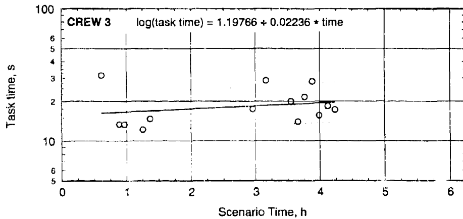
Figure C-37. Task times with regression lines for elevate tube in BDU.
