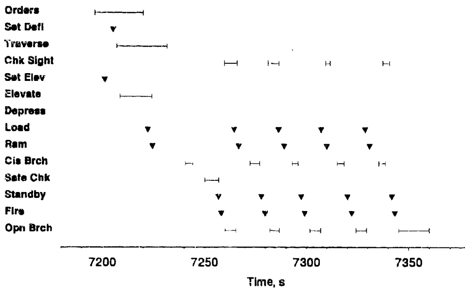
Figure A-35. Crew 3 timelines for fire missions 14 and 15 in BDU.
