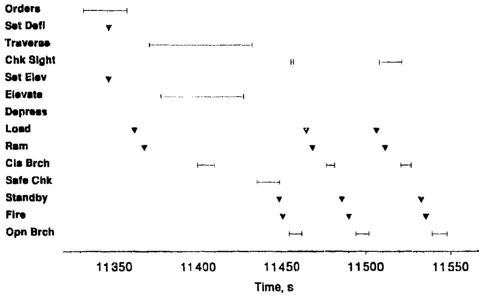
Figure A-25. Crew 2 timelines for fire missions 14 and 15 in MOPP4-R.
