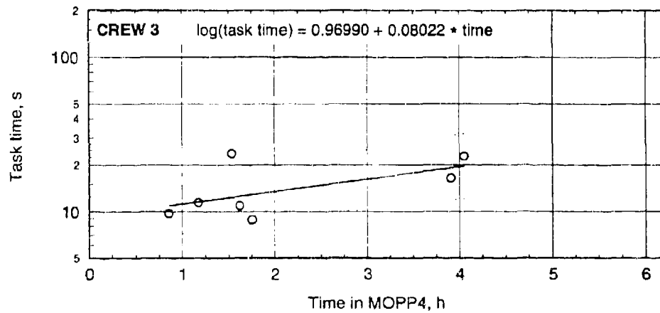
Figure C-65. Task times with regression lines for load first projo and pwdr in MOPP4-R.
