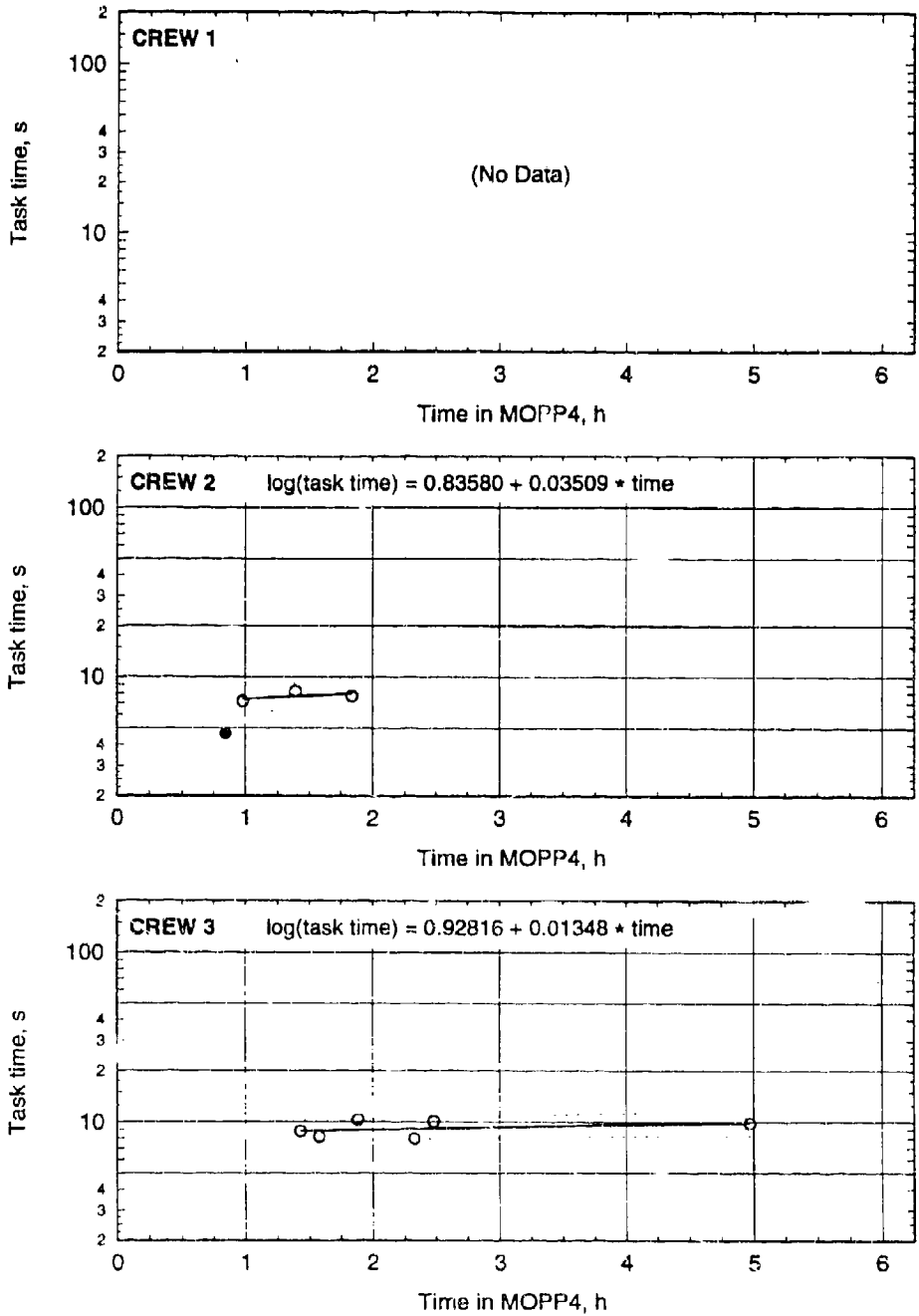
Figure C-57. Task times with regression lines for load first powder in MOPP4-S.
