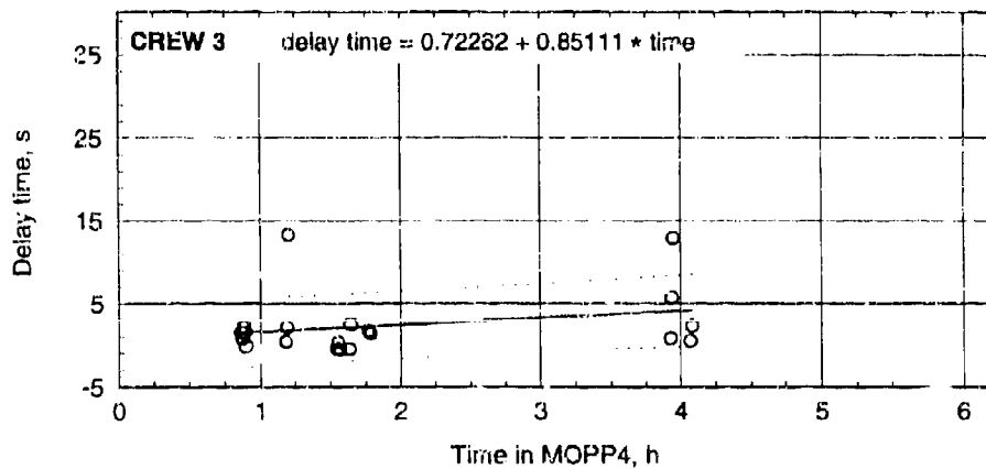
Figure C-101. Task times with regression lines for begin reload in MOPP4-R.
