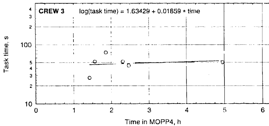
Figure C-45. Task times with regression lines for begin first load in MOPP4-S.
