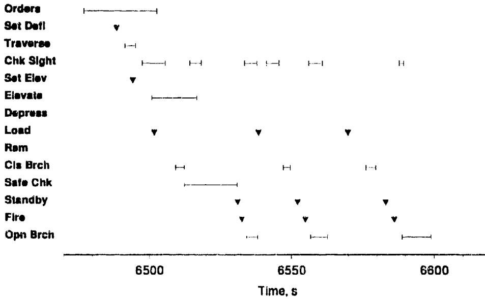
Figure A-9. Crew 1 timelines for fire missions 14 and 15 in BDU.
