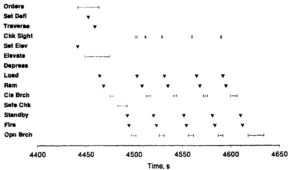
Figure A-14. Crew 2 timelines for fire missions 9 and 11 in BDU.
