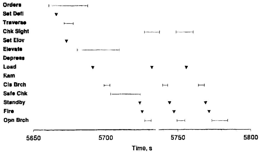
Figure A-8. Crew 1 timelines for firemissions 12 and 13 in BDU.
