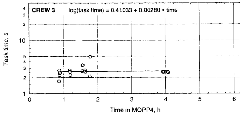
Figure C-83. Task times with regression lines for open breach in MOPP4-R.
