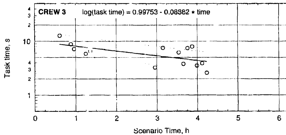
Figure C-91. Task times with regression lines for check sight in BDU.
