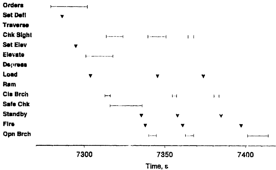
Figure A-10. Crew 1 timelines for fire missions 16 and 17 in BDU.
