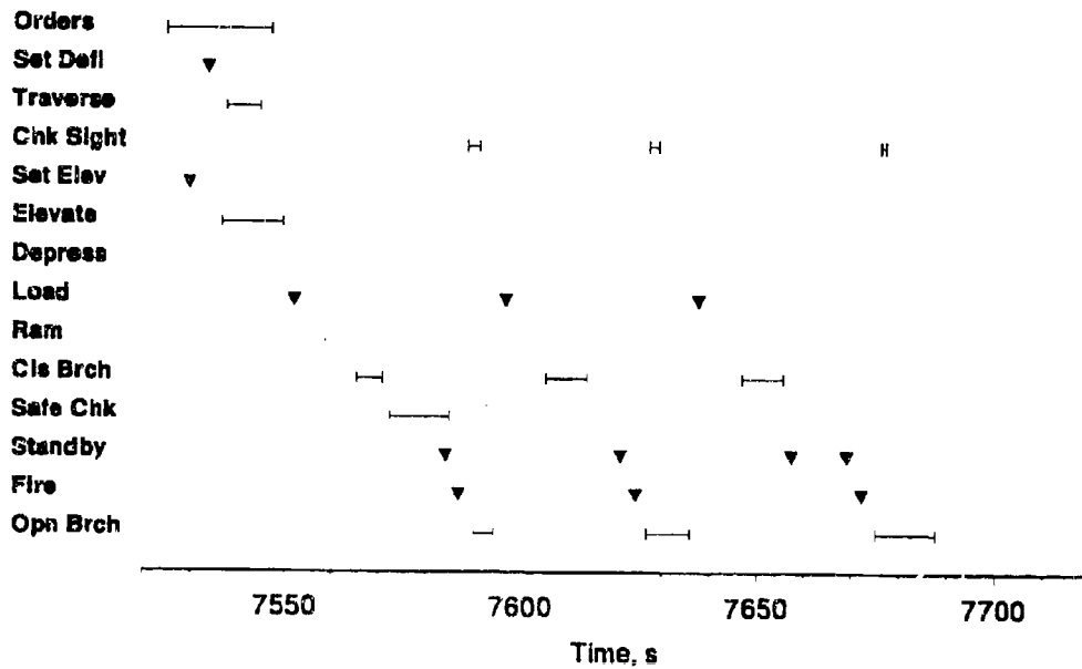
Figure A-2. Crew 1 timelines for fire missions 5 and 6 in MOPP4-S.
