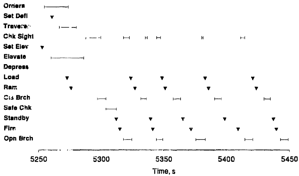
Figure A-16. Crew 2 timelines for fire missions 14 and 15 in BDU.
