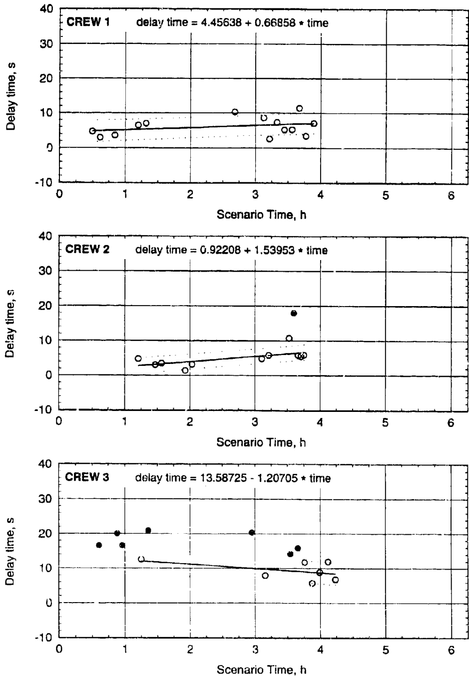
Figure C-7. Task times with regression lines for begin set deflection in BDU.
