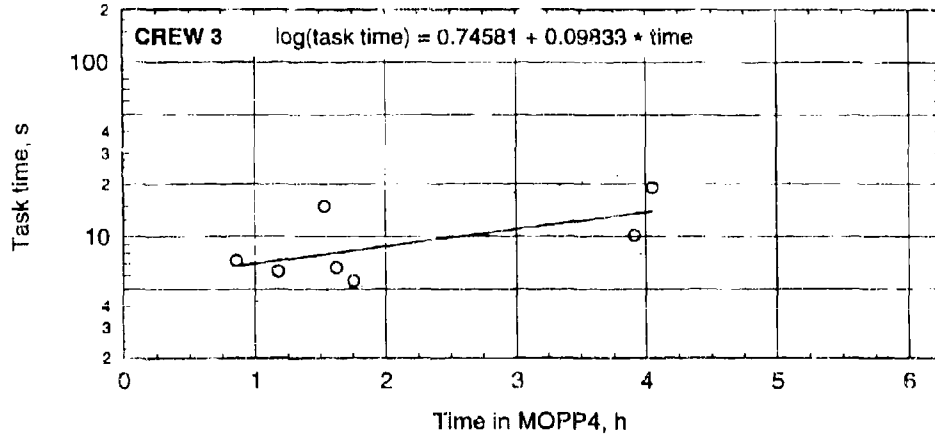
Figure C-59. Task times with regression lines for load first powder in MOPP4-R.
