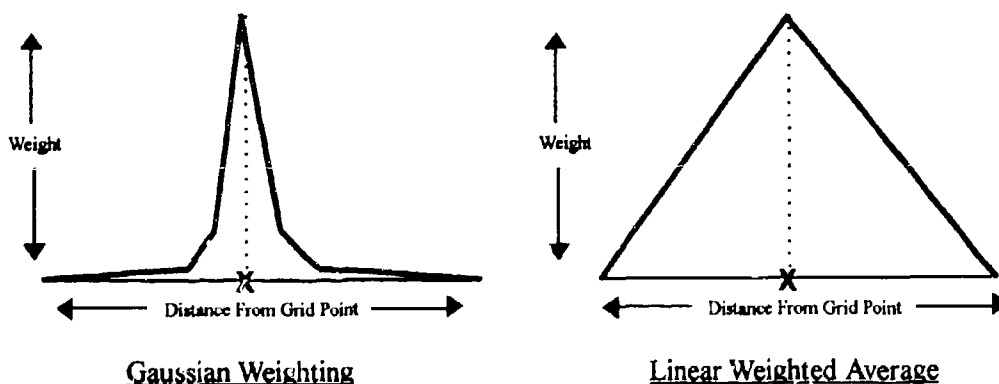
Figure 8. Examples of Gaussian and Linear Weighting
