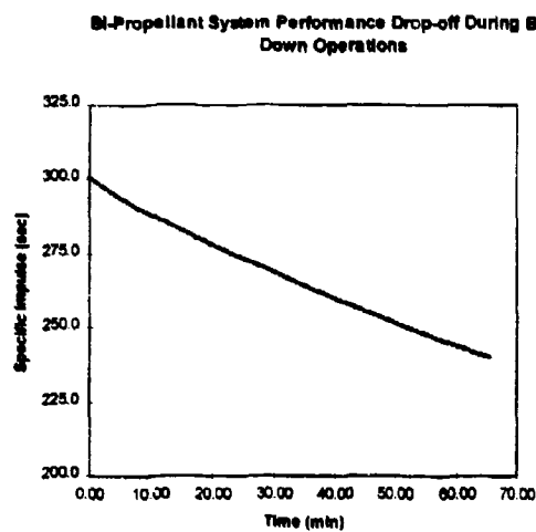
Figure 6-9: Bi-propellant System performance drop-off during blow-down operations. Simulation assumes 1 litre initial ullage in propellant tanks with initial ullage tank pressure of 35 bar.
