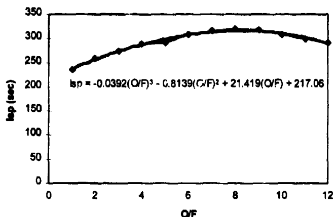
Figure 5-16: Relationship between O/F and I_{sp} for 17.5 bar (250 psi) chamber pressure, 150:1 expansion and 85% HTP. Darker line indicates derived 3 rd order polynomial relationship between the parameters used in simulation results.
